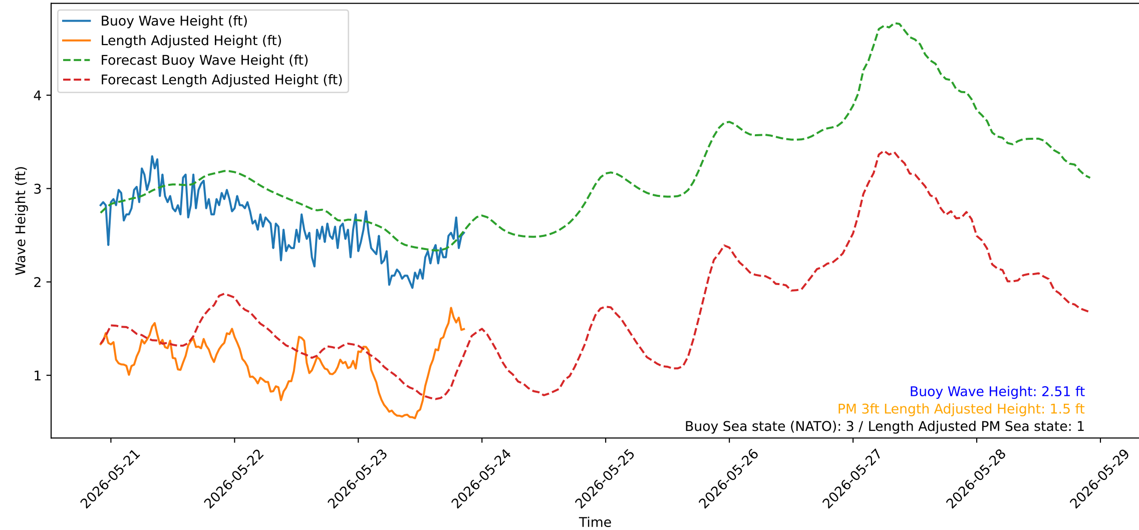
Wave Heights over Time for Red Beach at 2026-05-23 21:50:52
