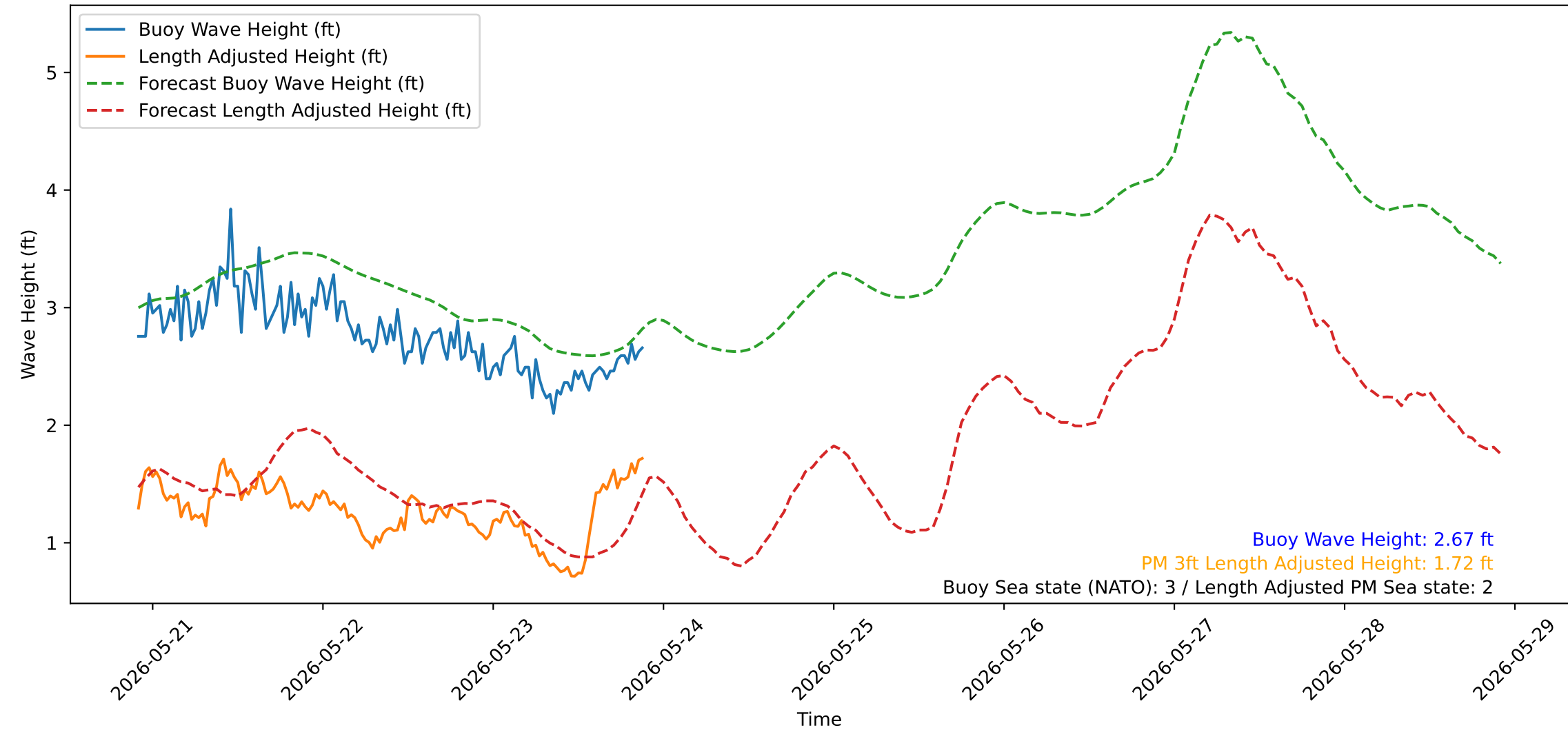
Wave Heights over Time for Oceanside Harbor at 2026-05-23 21:50:32
