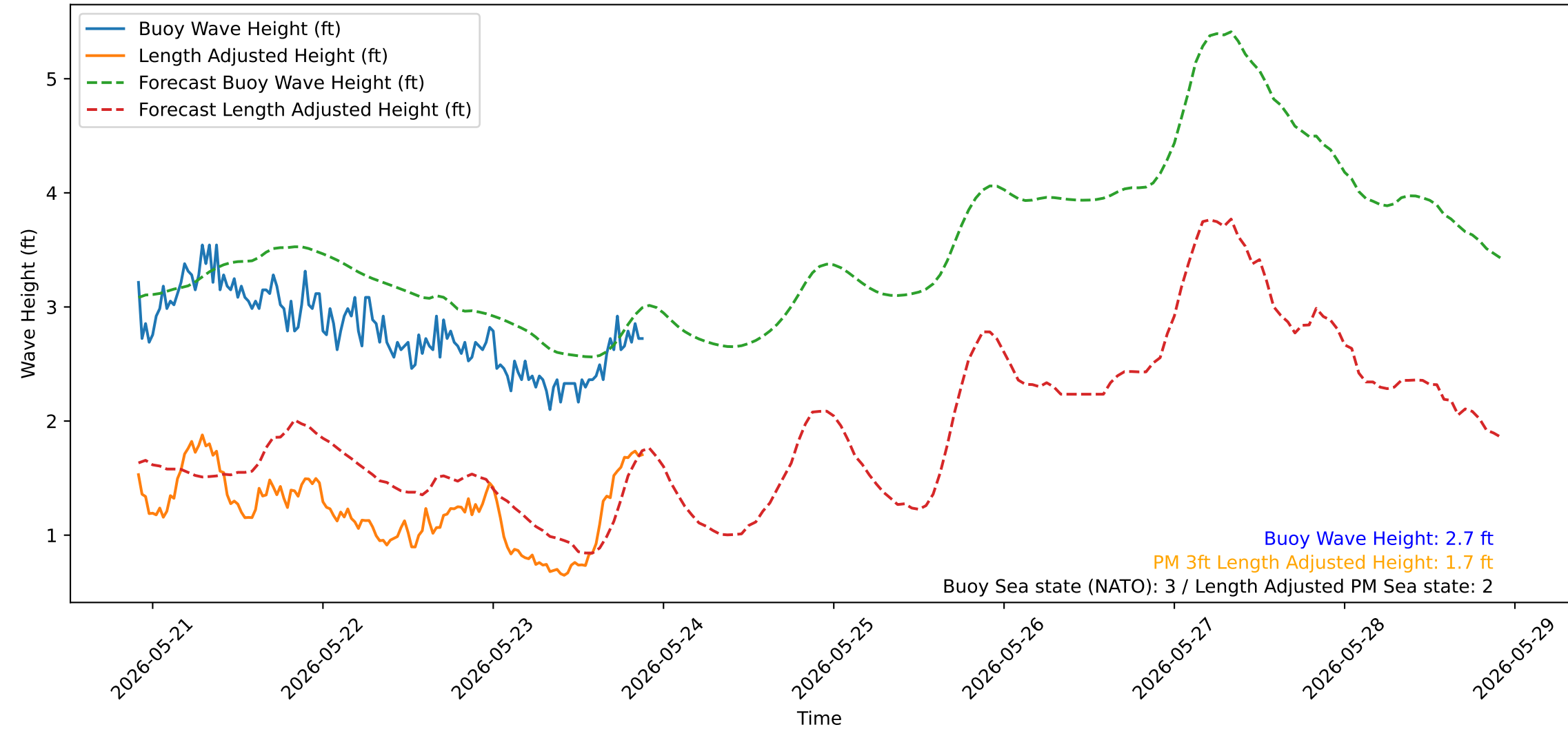
Wave Heights over Time for Green Beach at 2026-05-23 21:51:15
