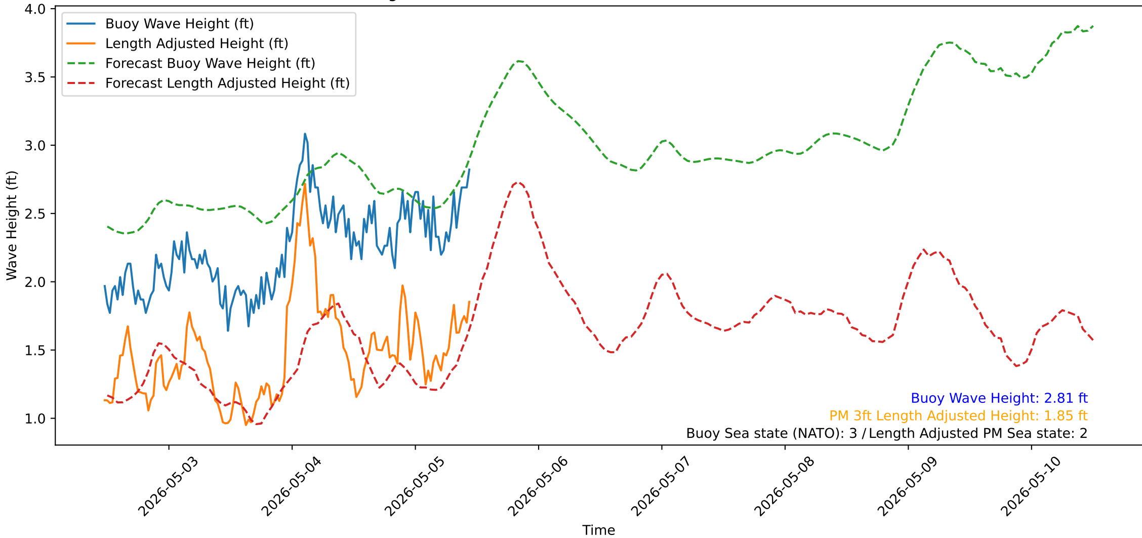
Wave Heights over Time for Oceanside Harbor at 2026-05-05 11:30:31
