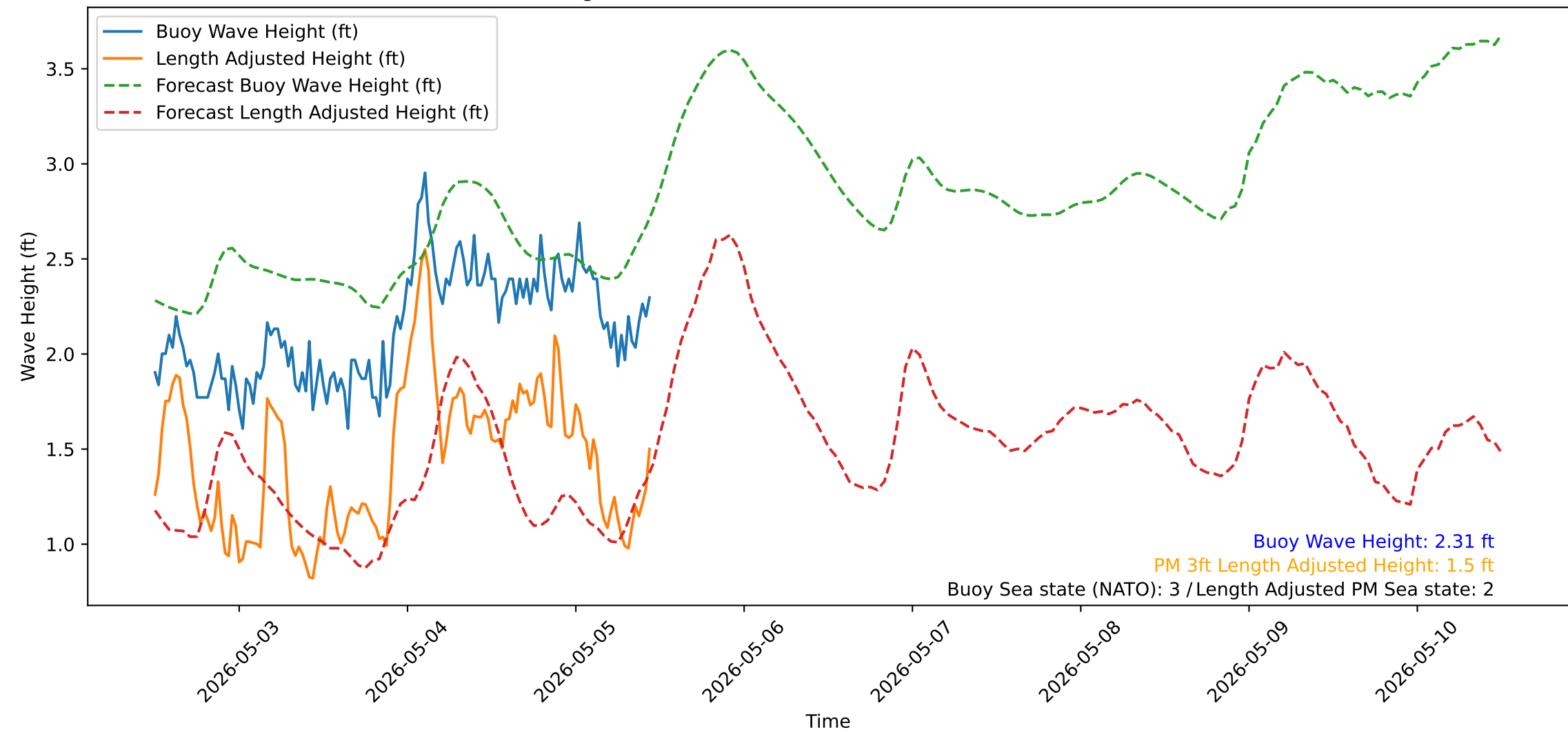
Wave Heights over Time for Red Beach at 2026-05-05 11:30:50
