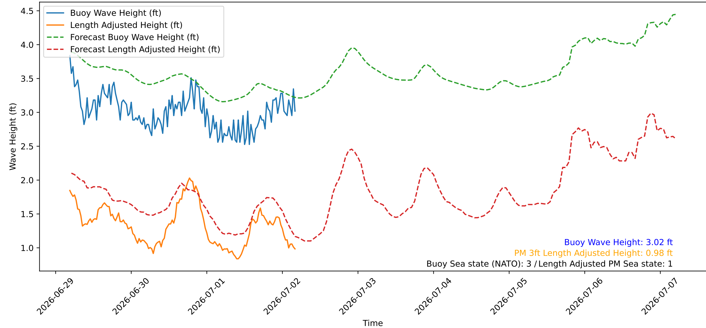
Wave Heights over Time for Green Beach at 2026-07-02 04:41:08
