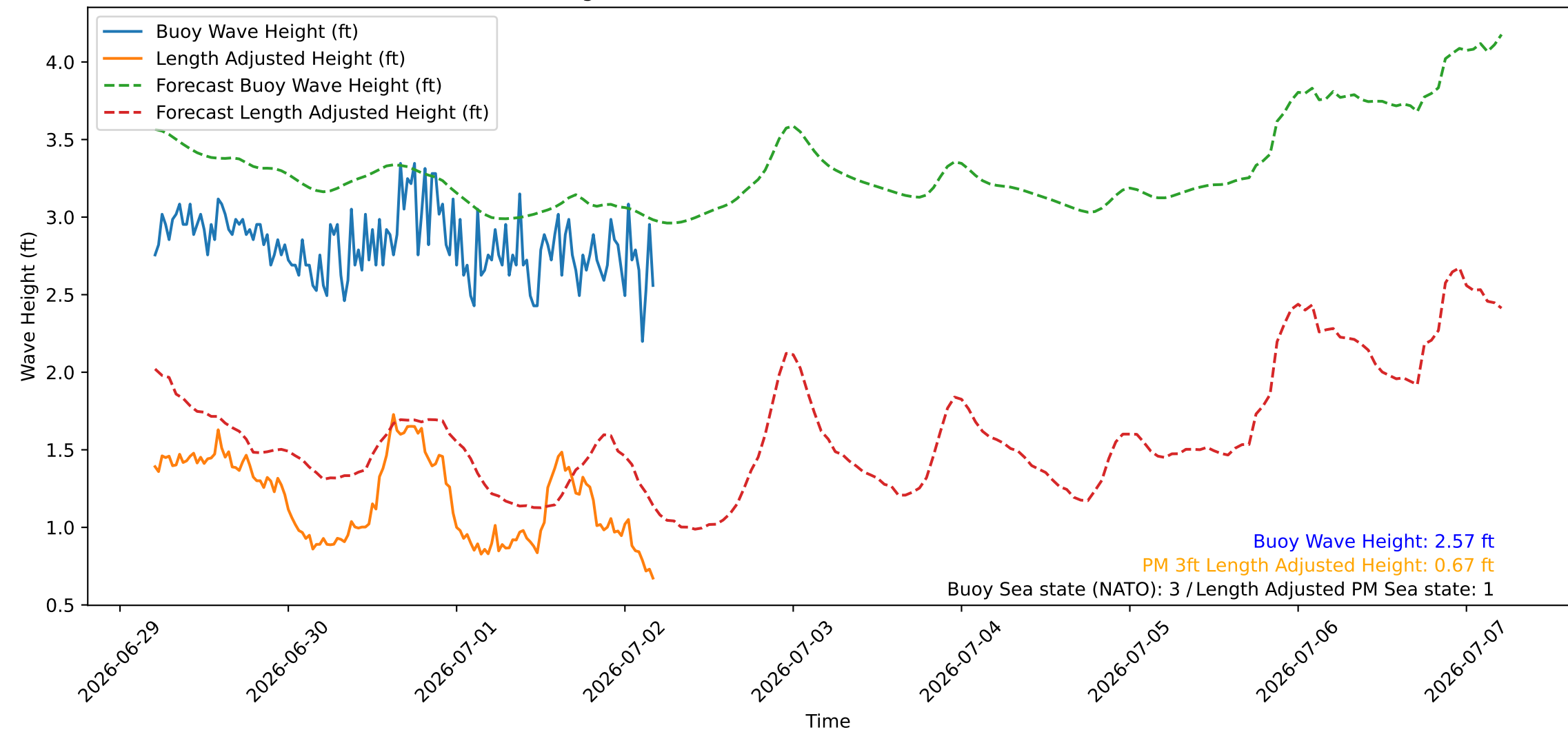
Wave Heights over Time for Red Beach at 2026-07-02 04:40:46
