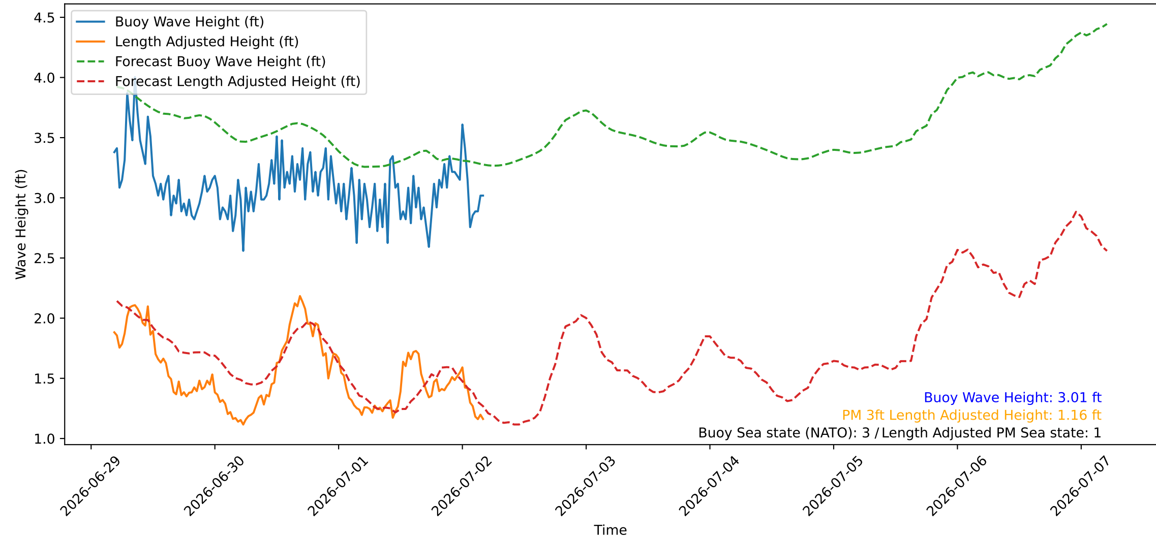
Wave Heights over Time for Oceanside Harbor at 2026-07-02 04:40:26
