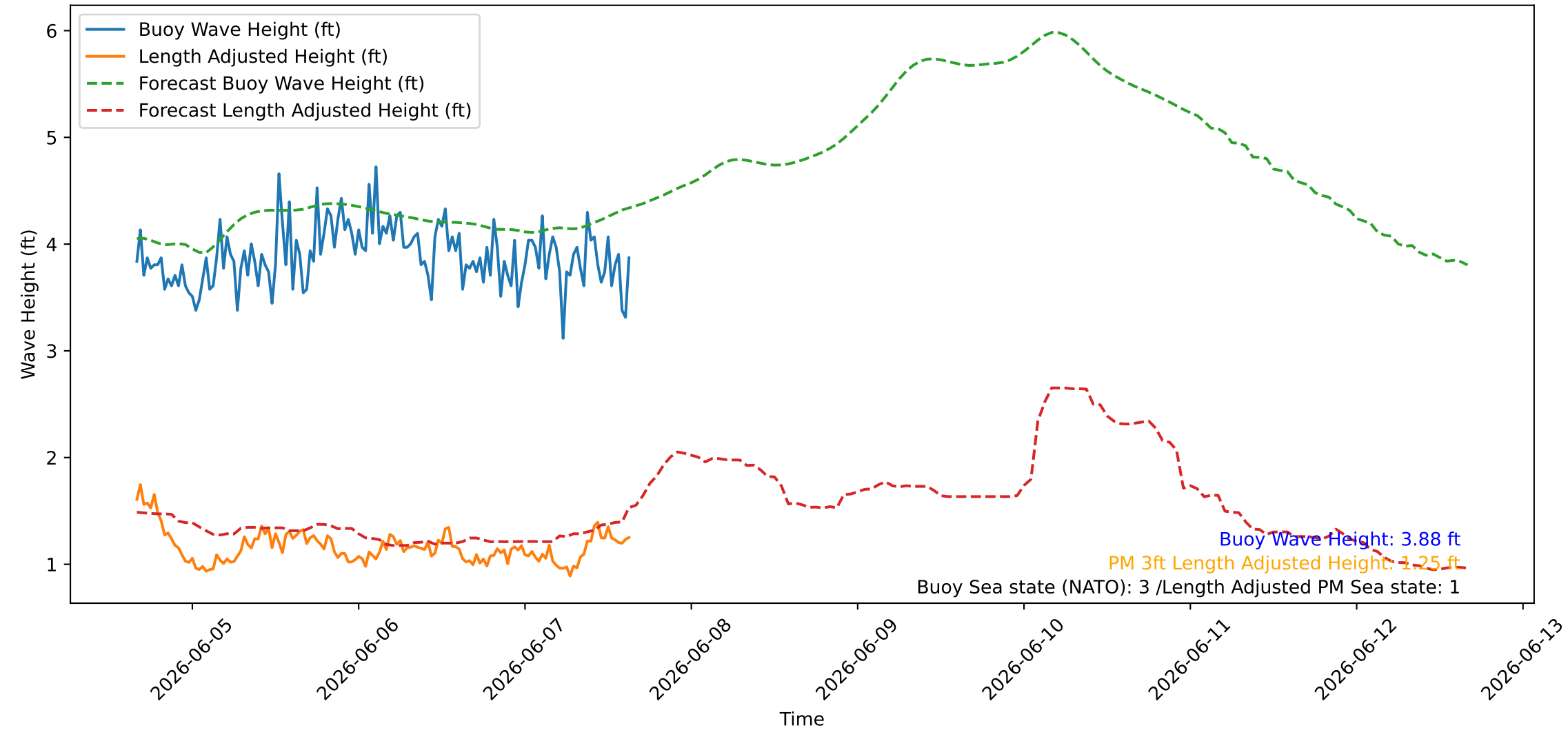
Wave Heights over Time for Green Beach at 2026-06-07 16:01:08
