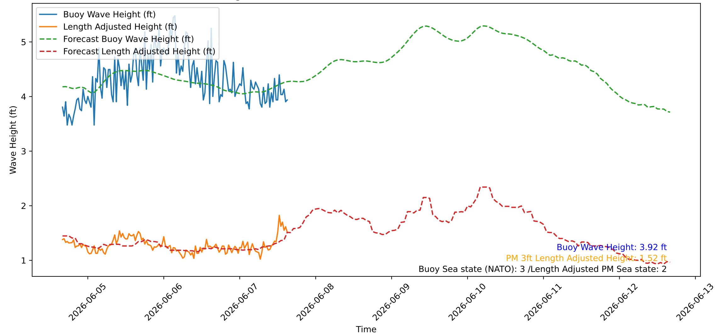
Wave Heights over Time for Oceanside Harbor at 2026-06-07 16:00:26
