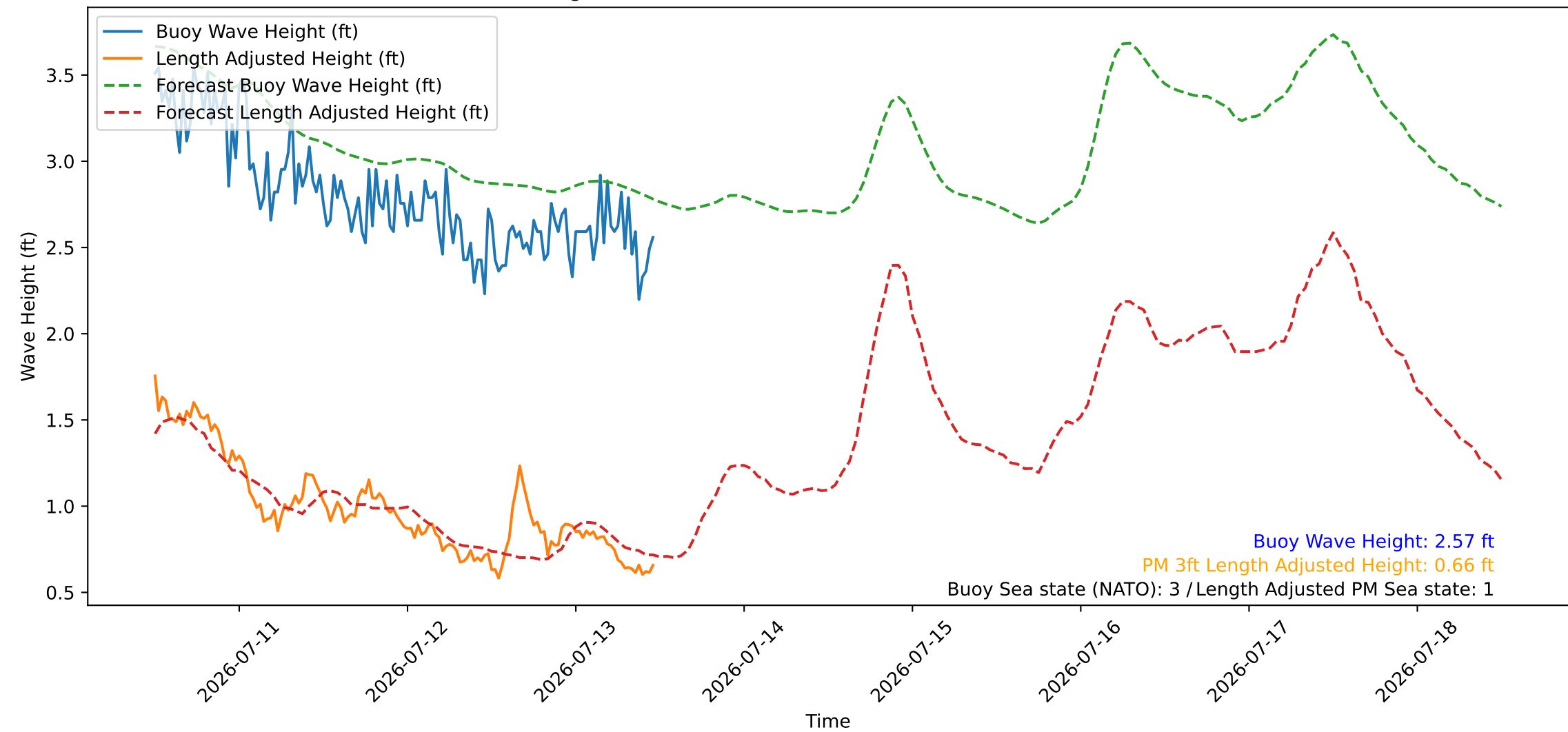
Wave Heights over Time for Green Beach at 2026-07-13 12:01:09
