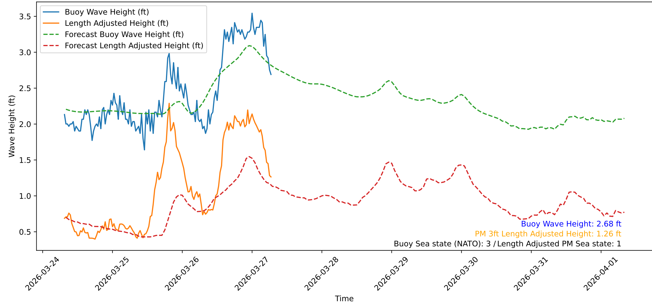
Wave Heights over Time for Green Beach at 2026-03-27 07:31:10
