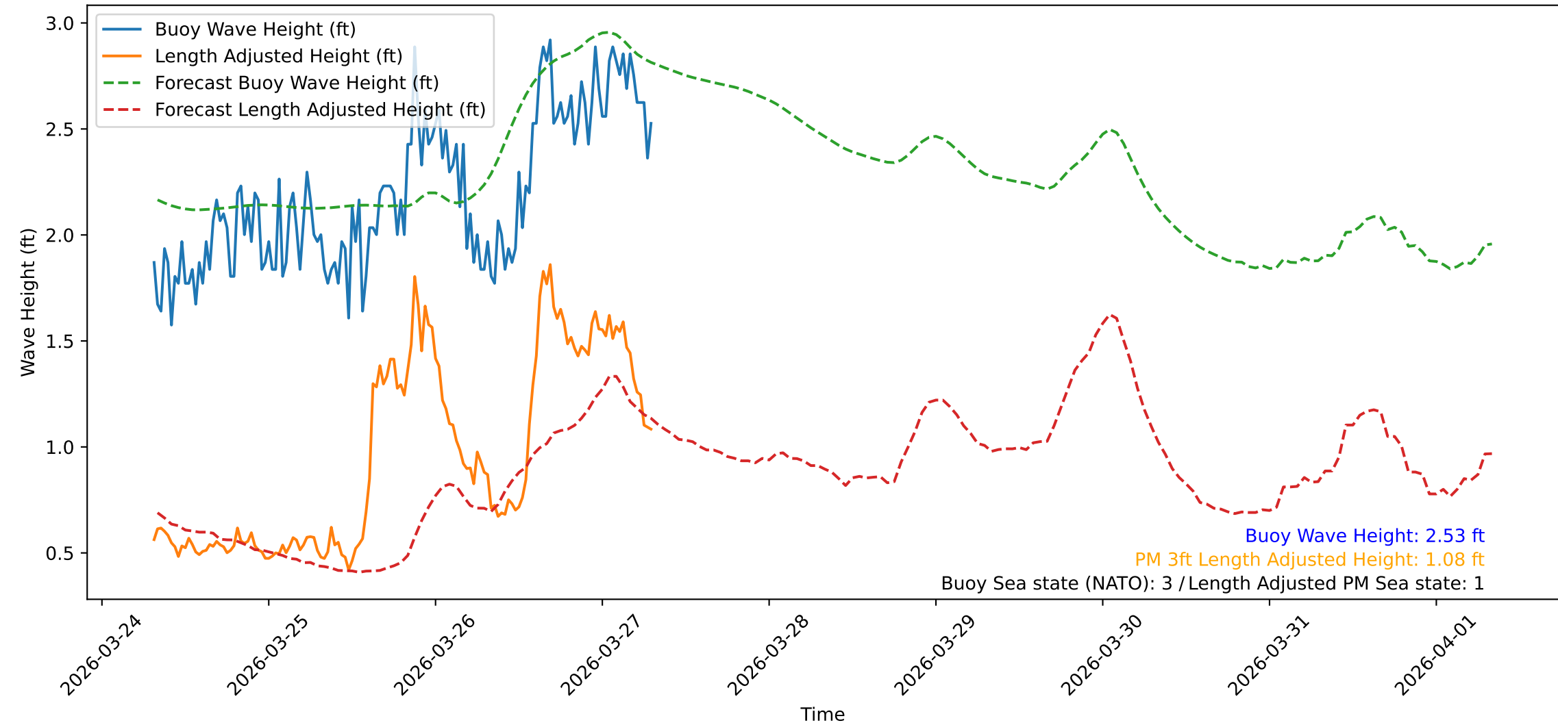
Wave Heights over Time for Oceanside Harbor at 2026-03-27 07:30:31
