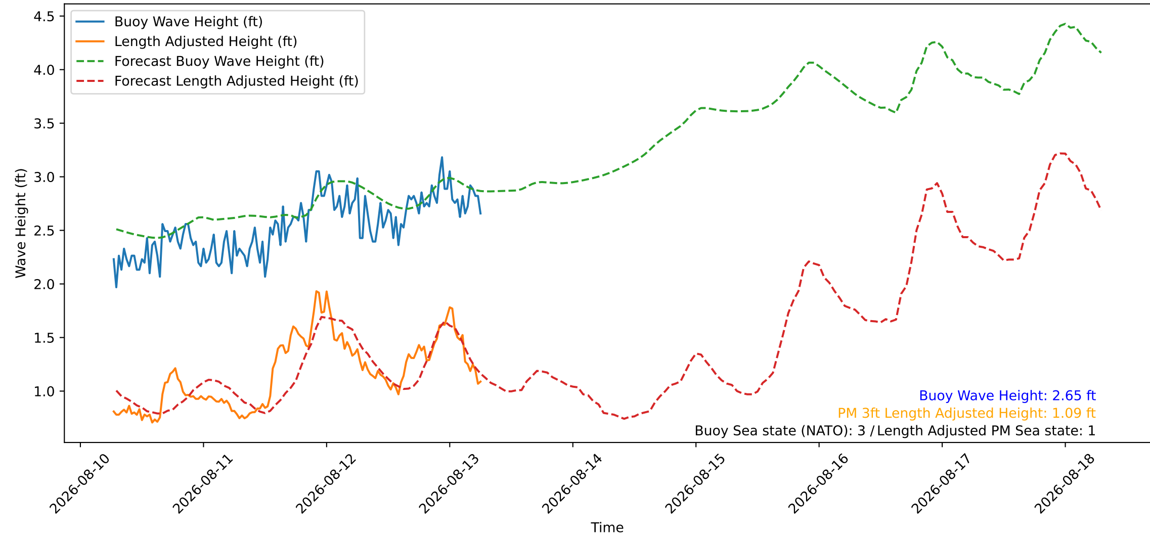
Wave Heights over Time for Oceanside Harbor at 2026-08-13 06:40:27
