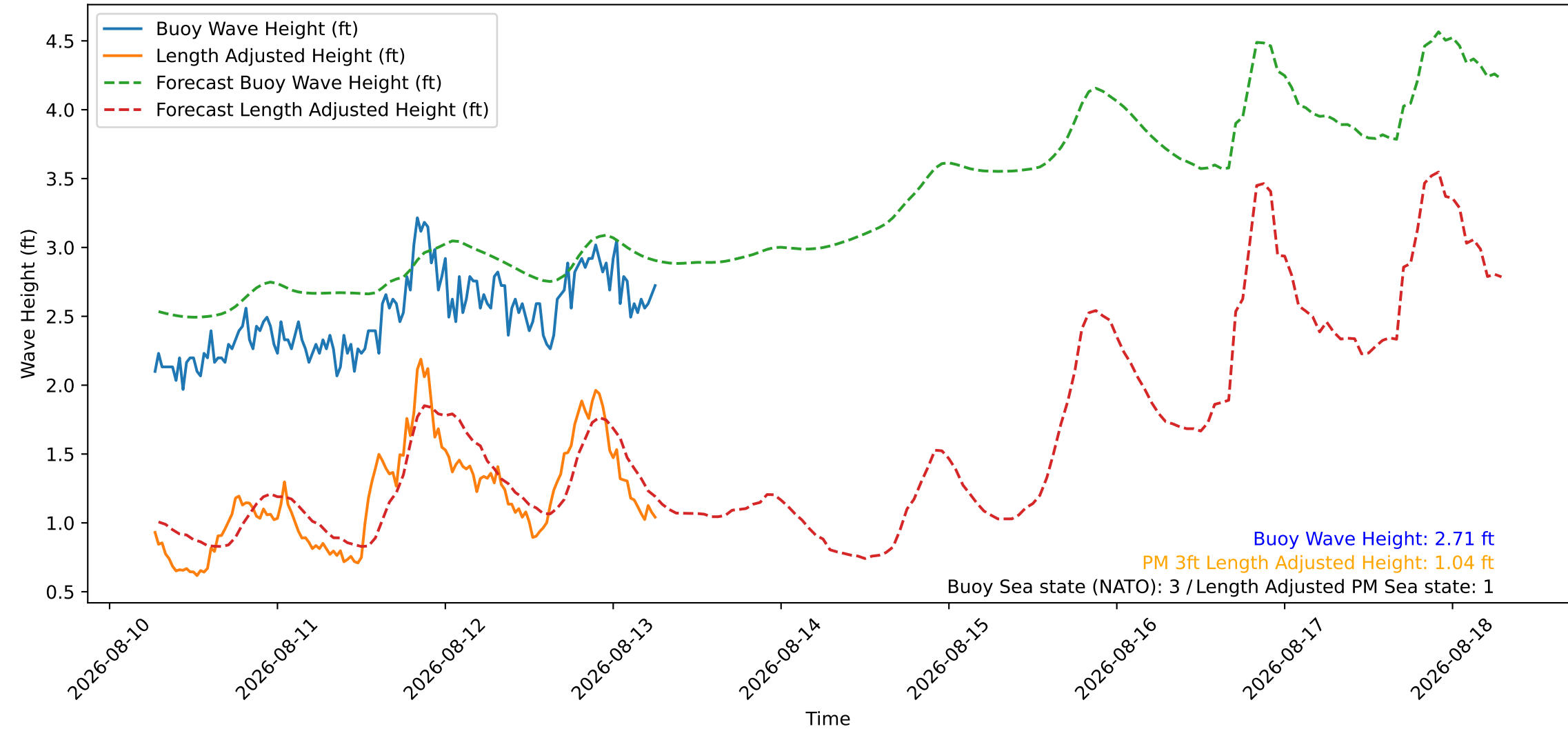
Wave Heights over Time for Green Beach at 2026-08-13 06:41:09
