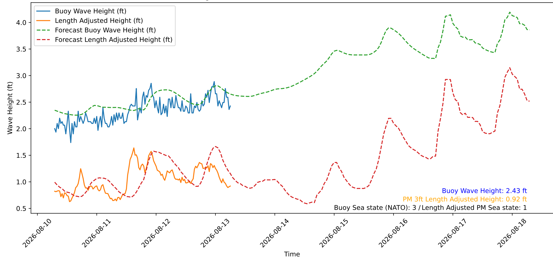
Wave Heights over Time for Red Beach at 2026-08-13 06:40:46
