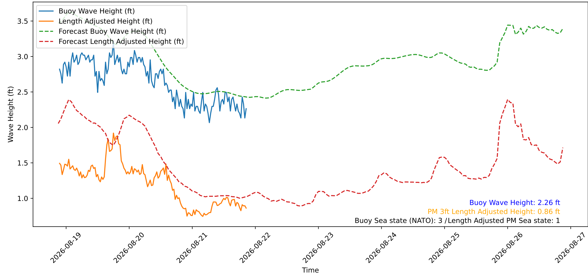
Wave Heights over Time for Red Beach at 2026-08-21 21:10:46
