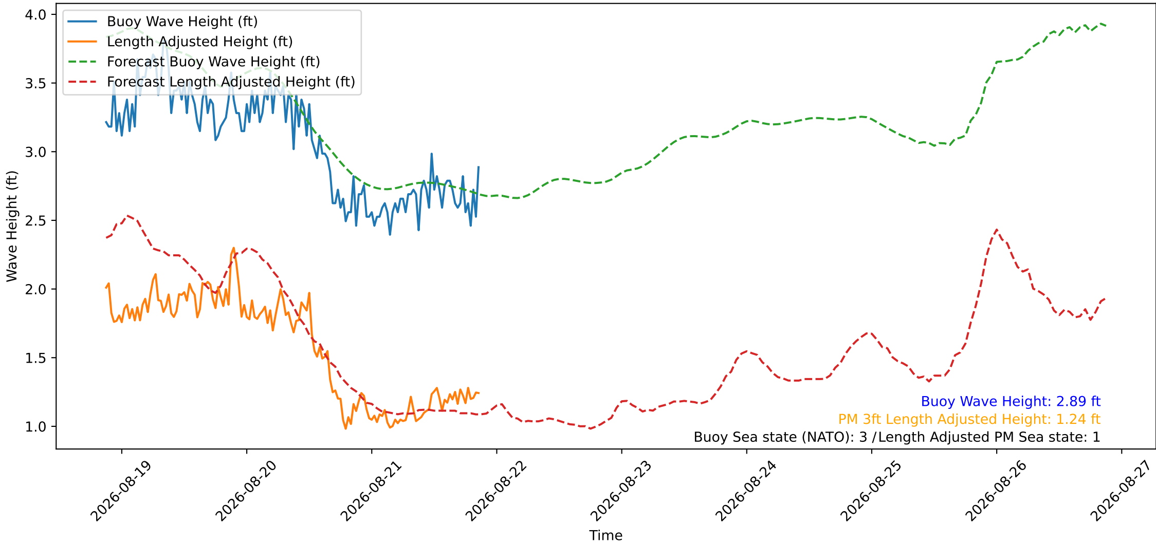
Wave Heights over Time for Oceanside Harbor at 2026-08-21 21:10:26
