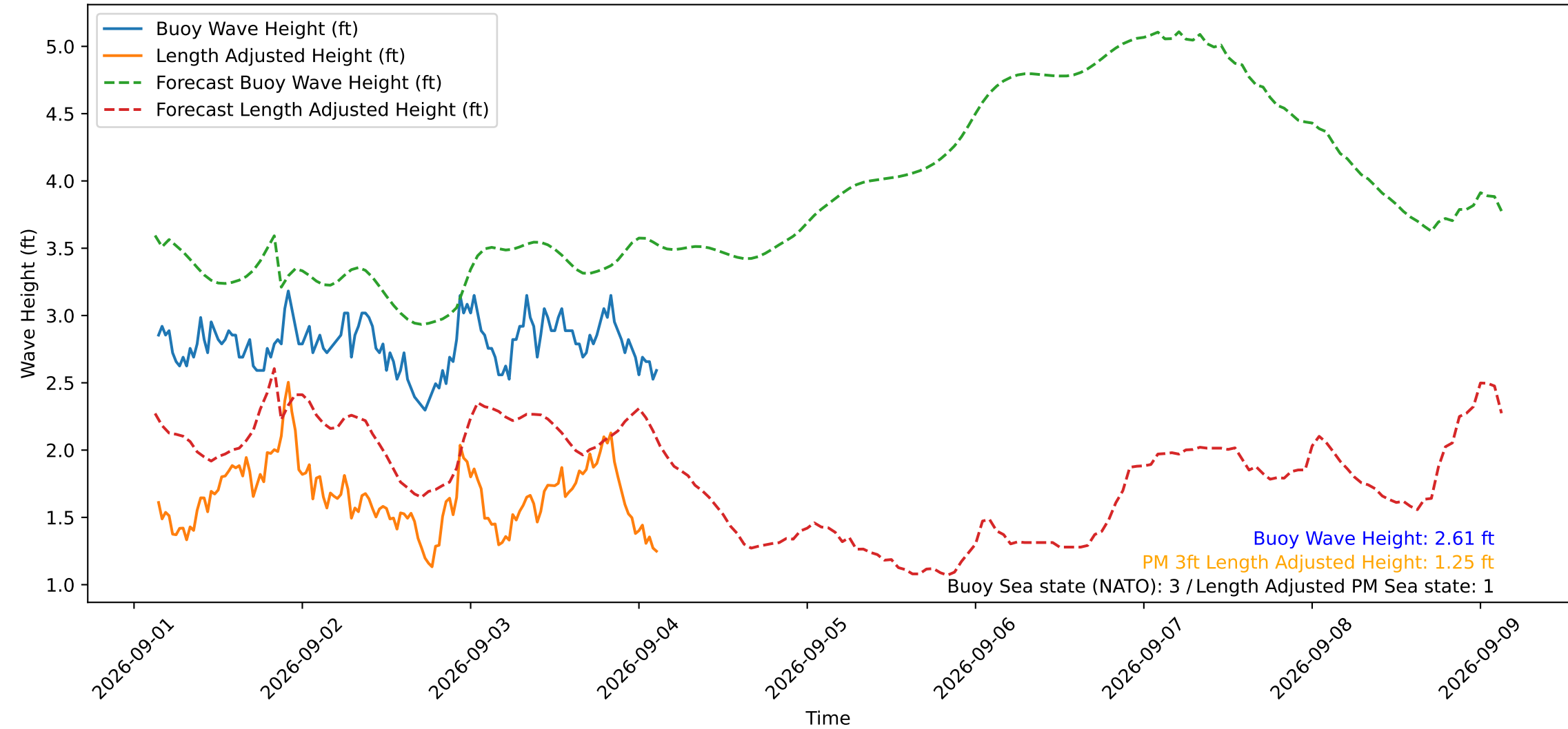
Wave Heights over Time for Red Beach at 2026-09-04 03:20:50
