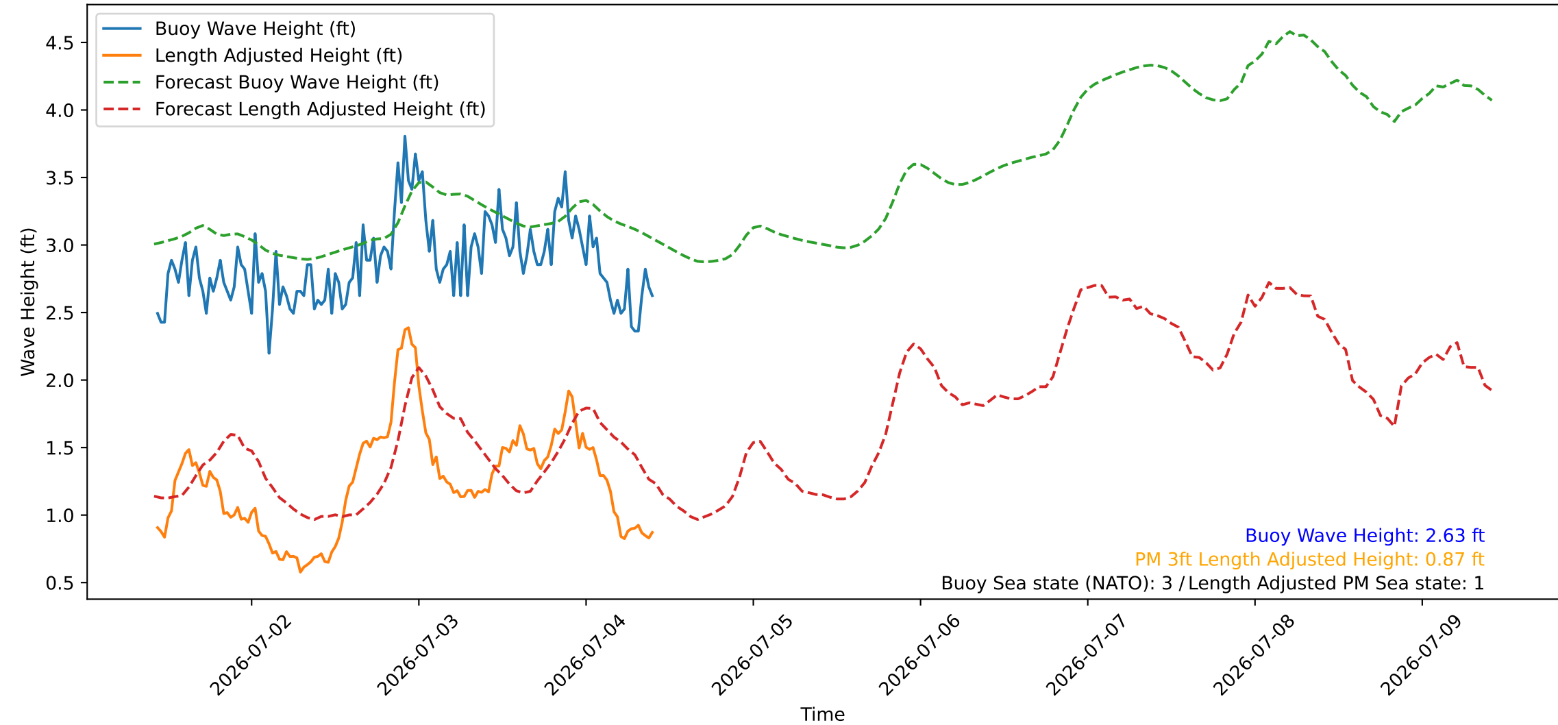
Wave Heights over Time for Red Beach at 2026-07-04 10:10:45
