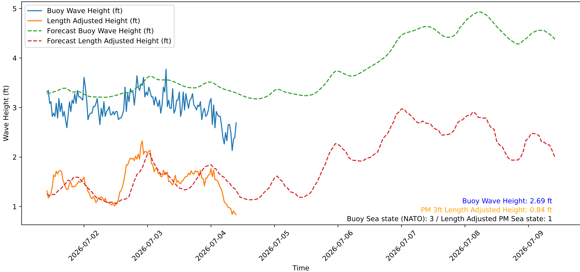
Wave Heights over Time for Oceanside Harbor at 2026-07-04 10:10:26
