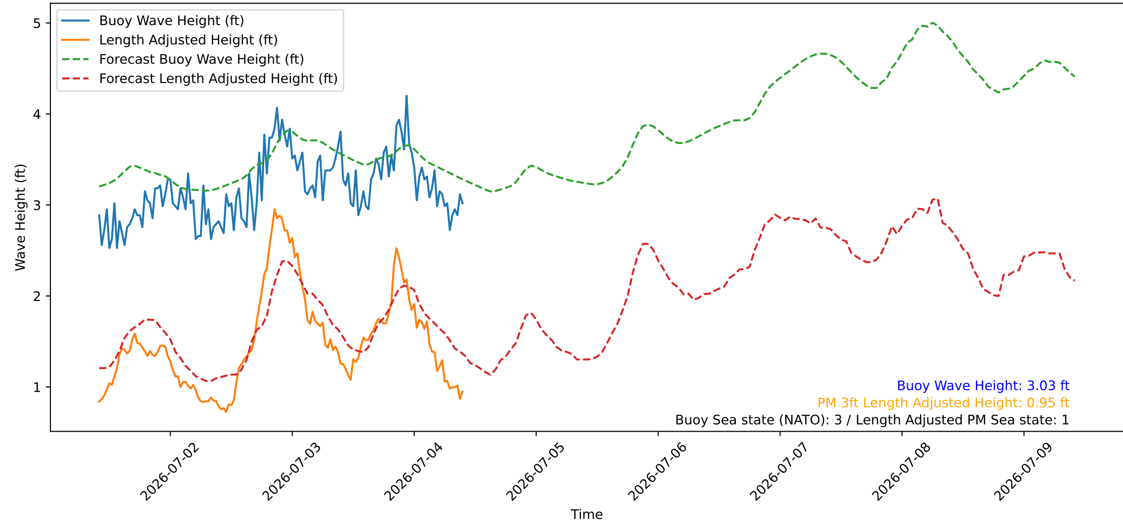
Wave Heights over Time for Green Beach at 2026-07-04 10:11:08
