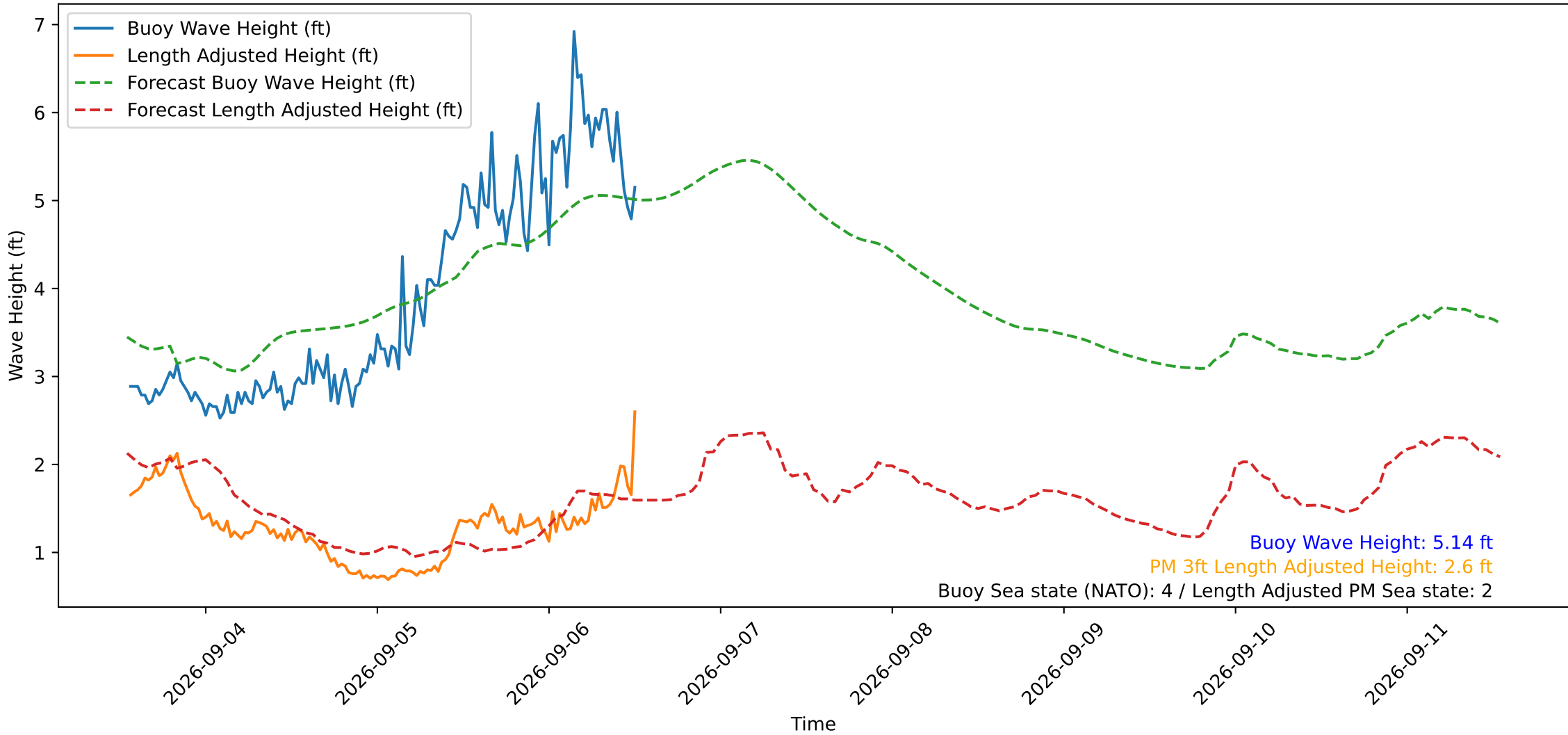
Wave Heights over Time for Red Beach at 2026-09-06 13:00:50
