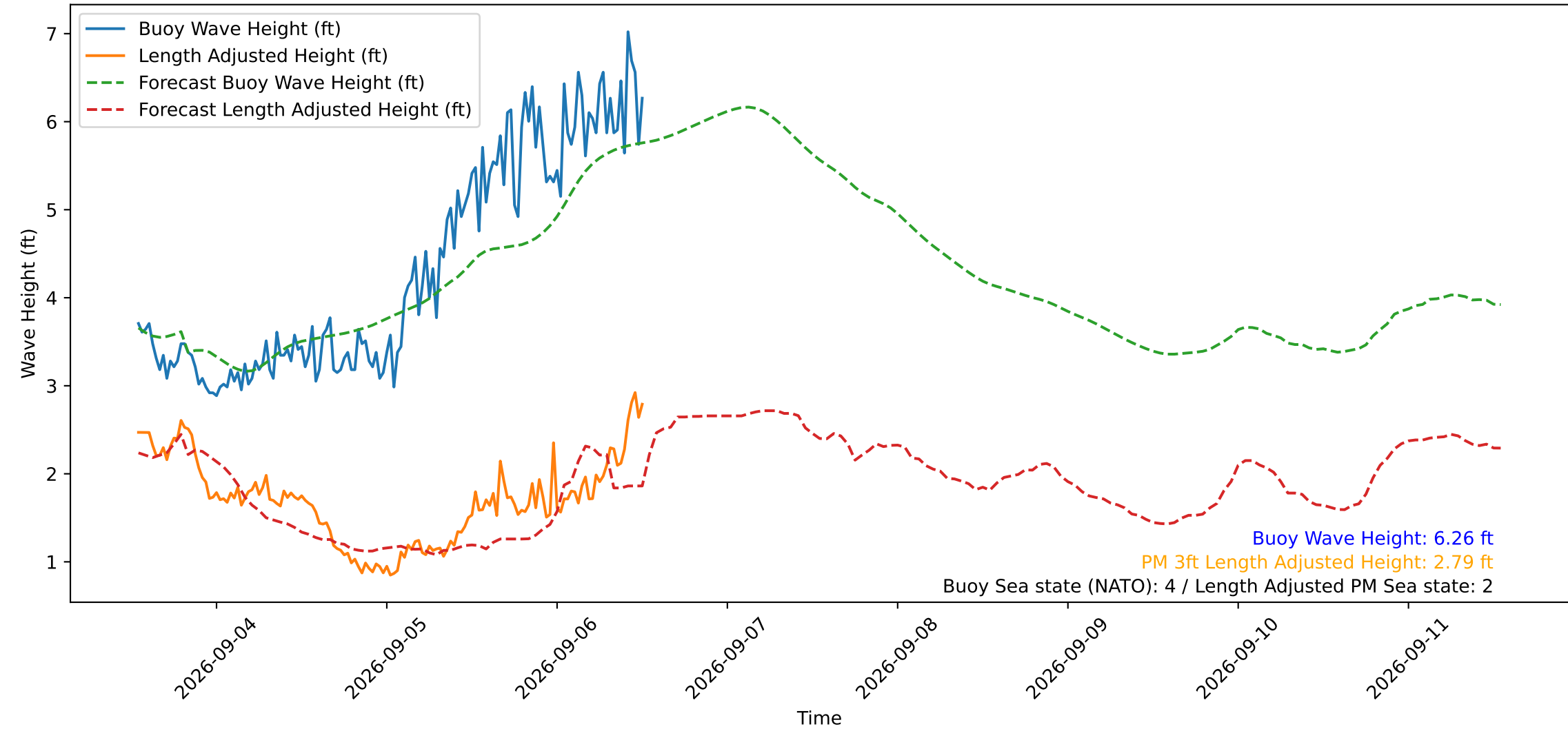
Wave Heights over Time for Oceanside Harbor at 2026-09-06 13:00:30
