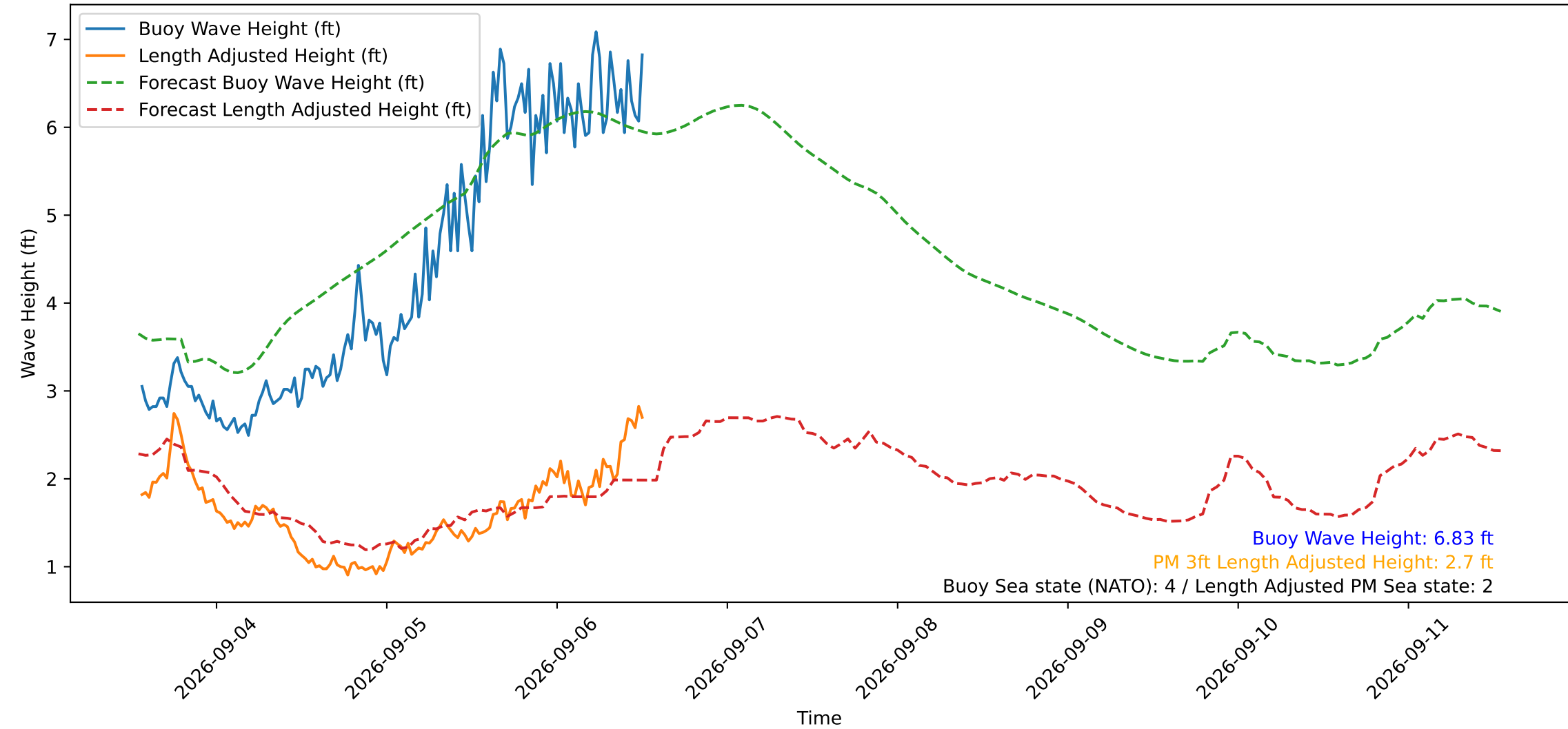
Wave Heights over Time for Green Beach at 2026-09-06 13:01:12
