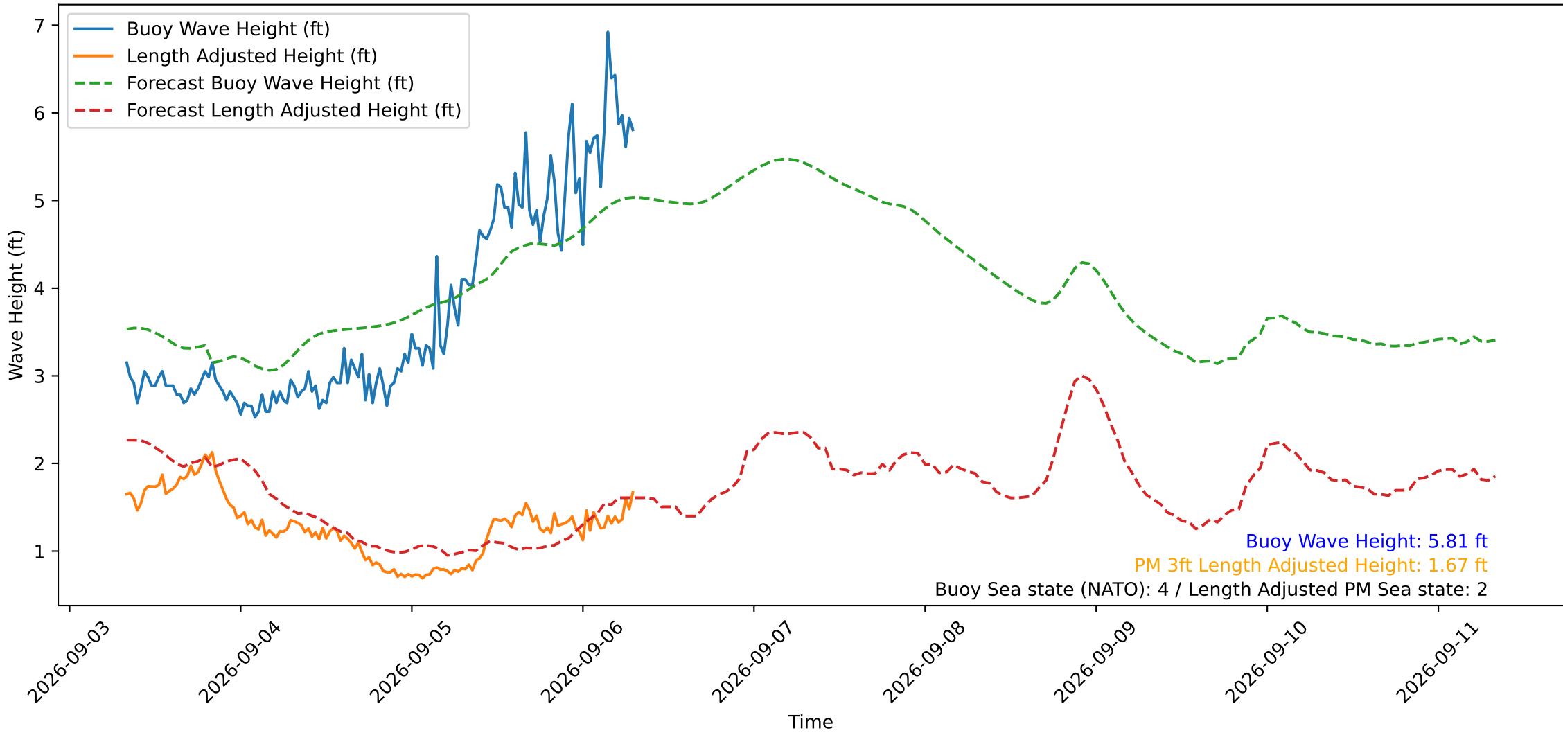
Wave Heights over Time for Red Beach at 2026-09-06 07:50:50
