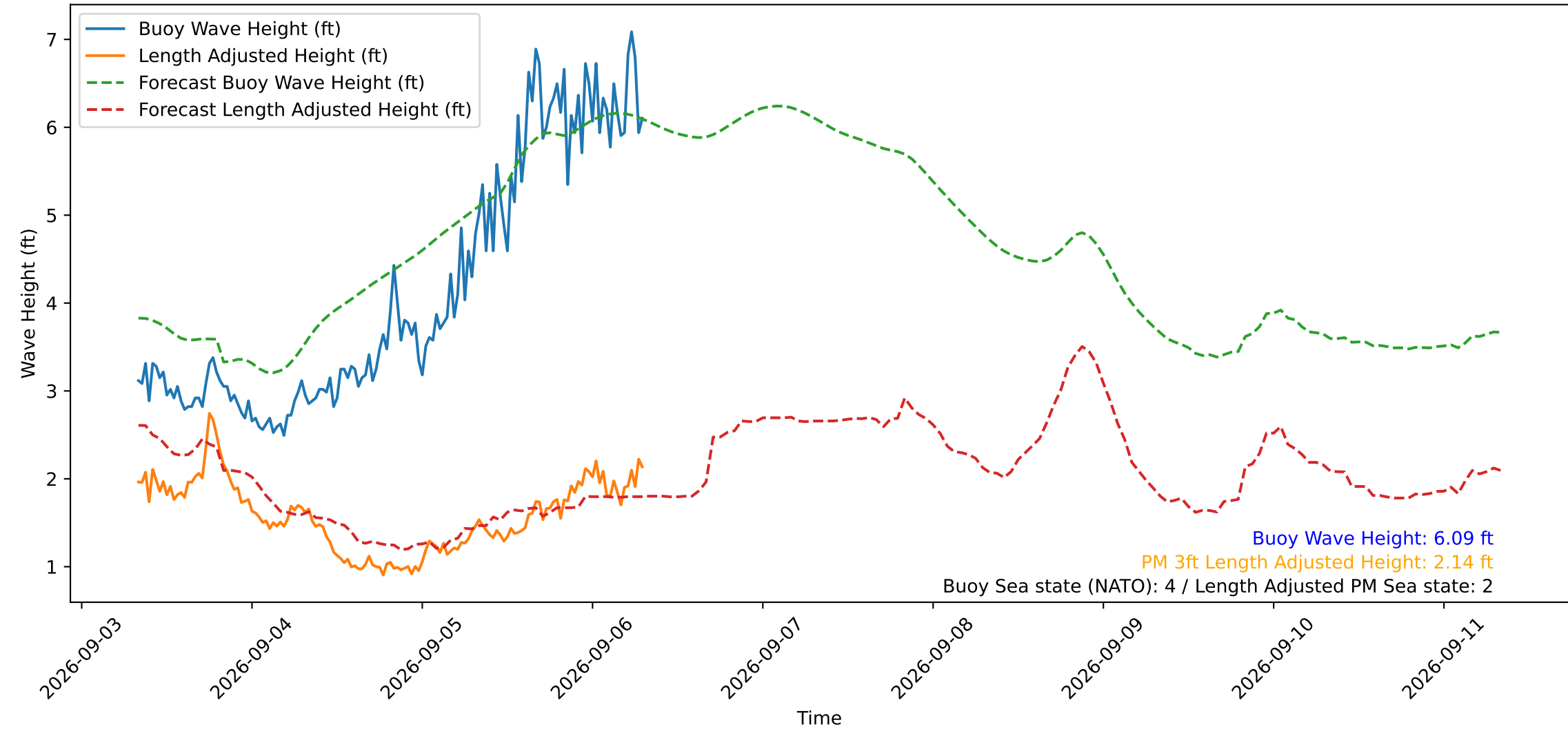
Wave Heights over Time for Green Beach at 2026-09-06 07:51:14
