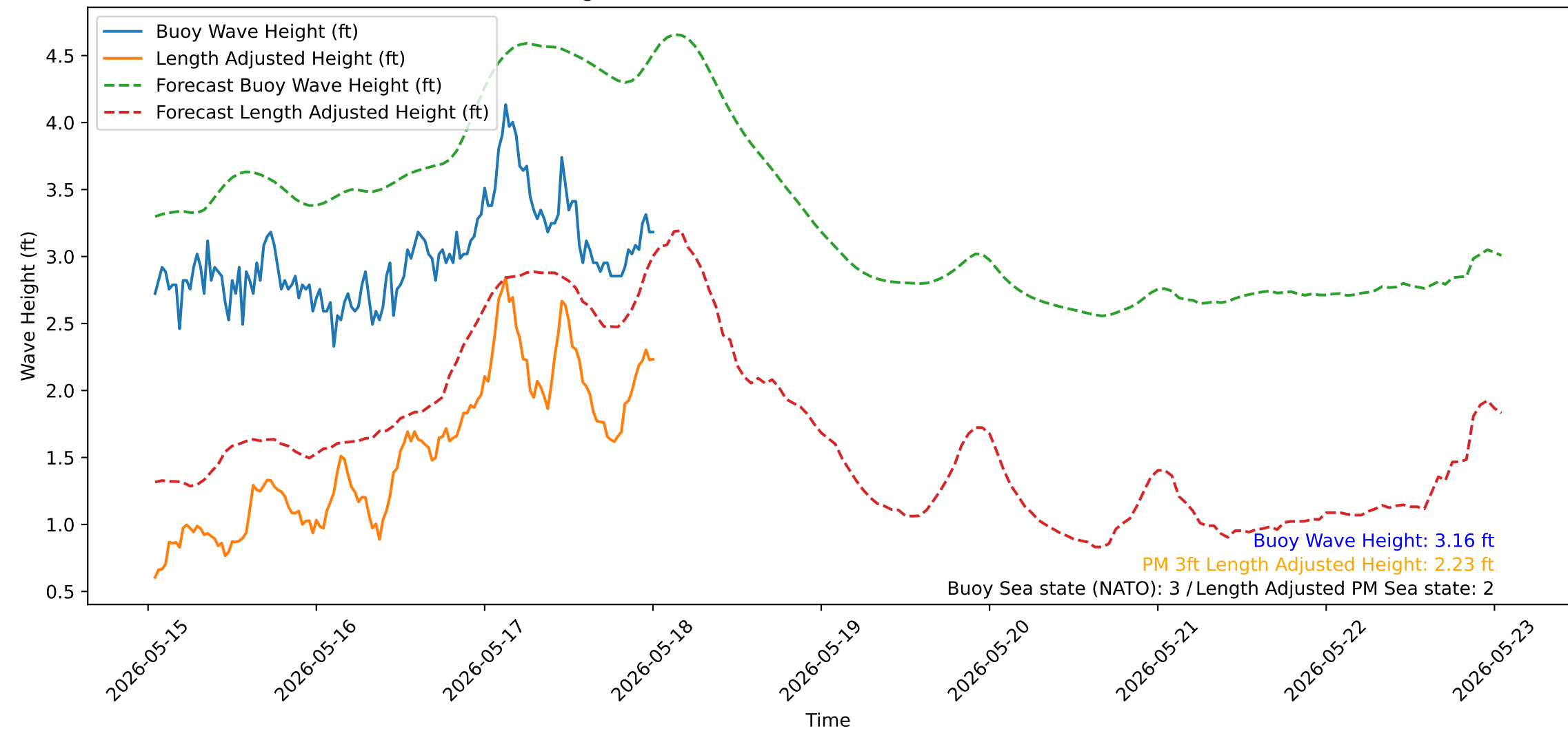
Wave Heights over Time for Red Beach at 2026-05-18 00:50:51
