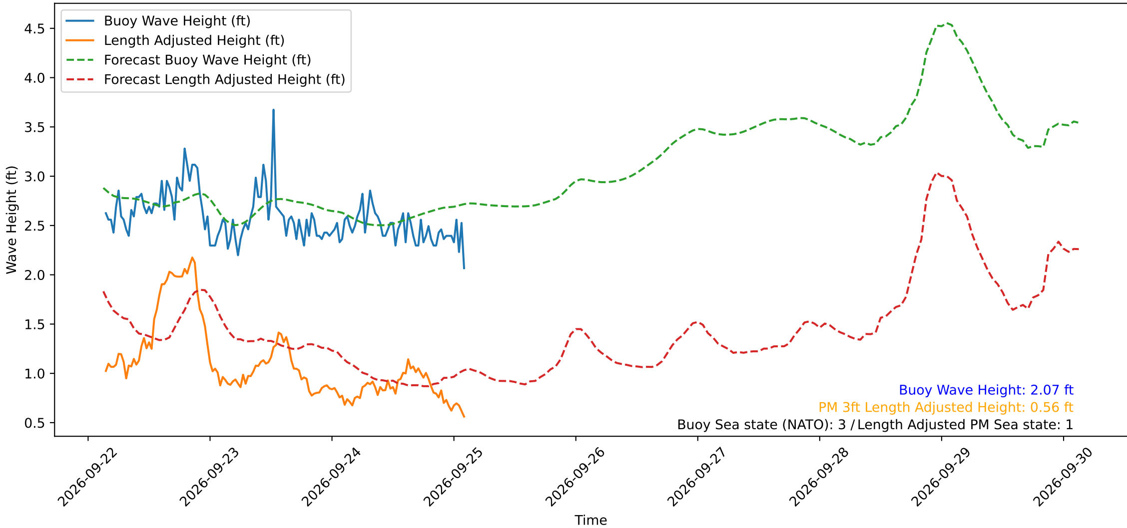
Wave Heights over Time for Red Beach at 2026-09-25 03:00:48
