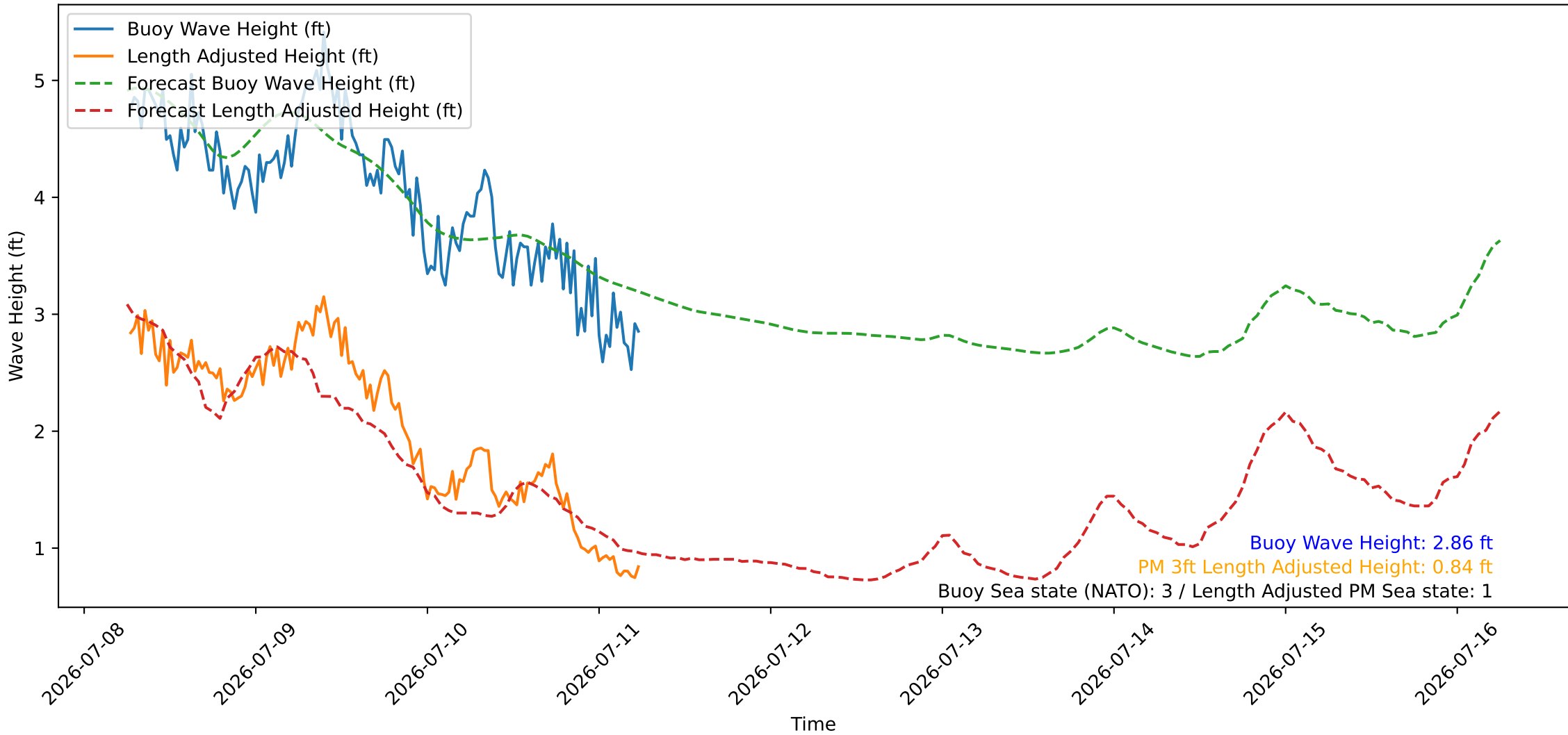
Wave Heights over Time for Oceanside Harbor at 2026-07-11 06:20:26
