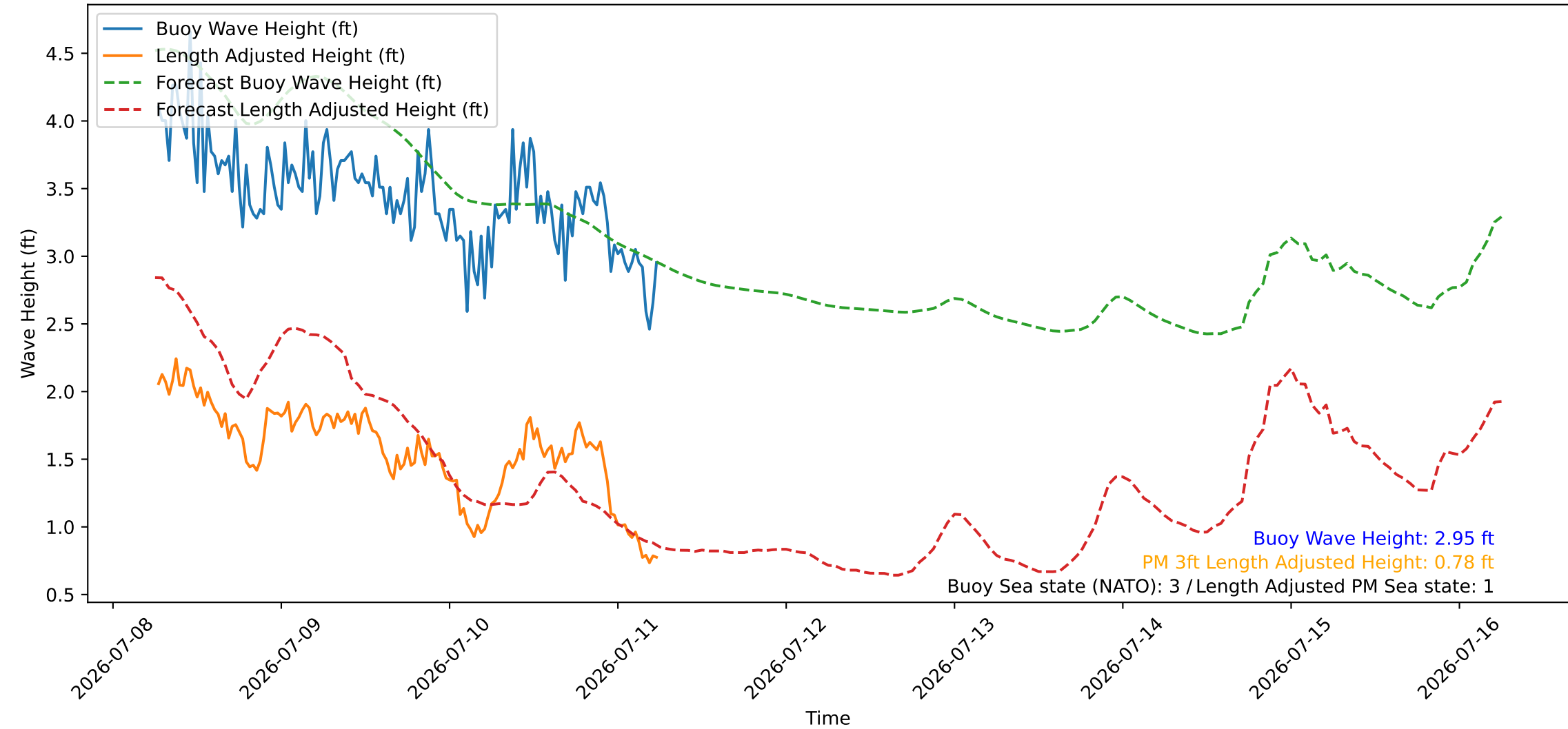
Wave Heights over Time for Red Beach at 2026-07-11 06:20:47
