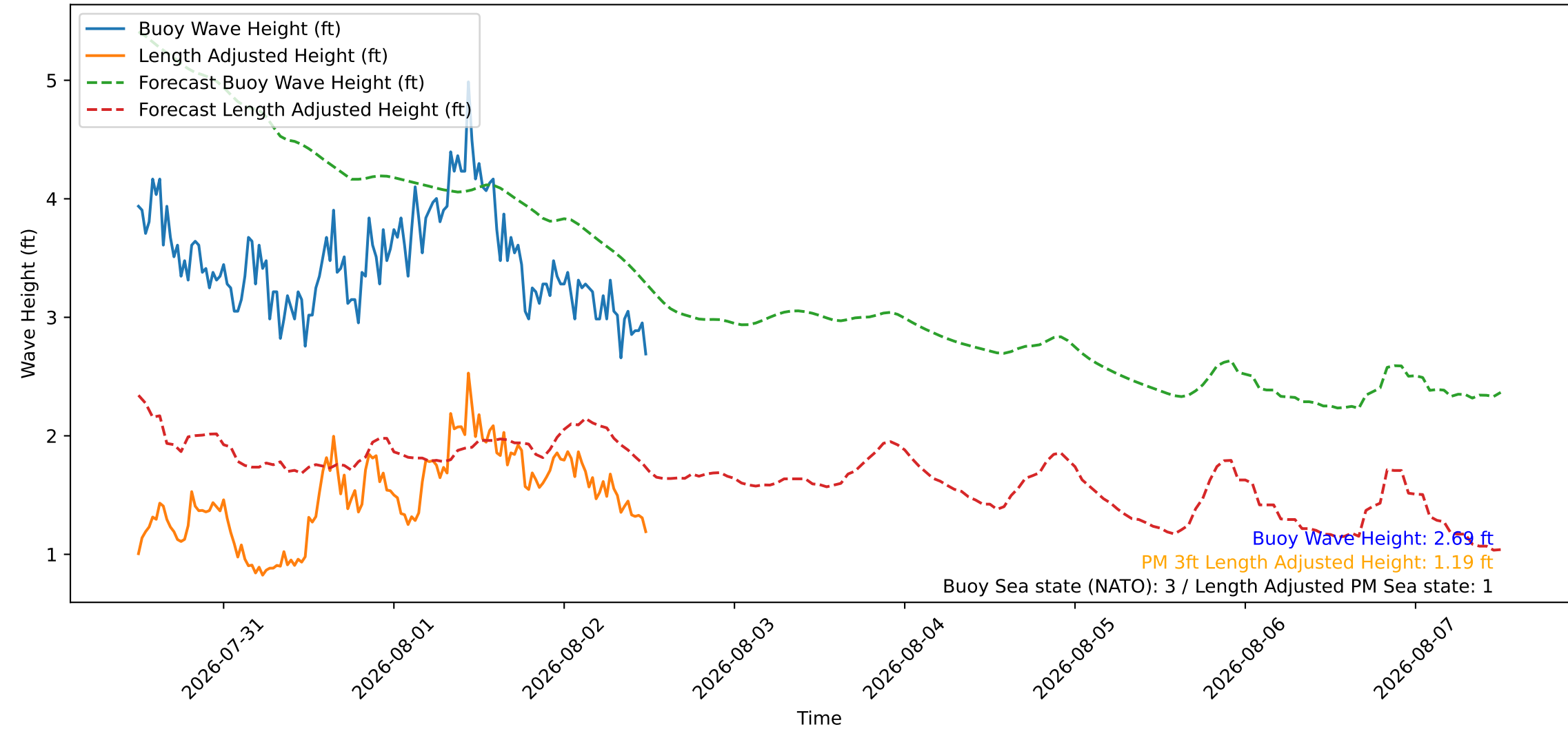
Wave Heights over Time for Green Beach at 2026-08-02 12:11:08
