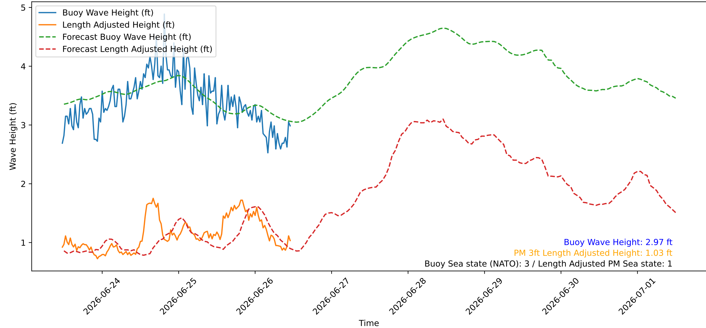
Wave Heights over Time for Oceanside Harbor at 2026-06-26 11:30:26
