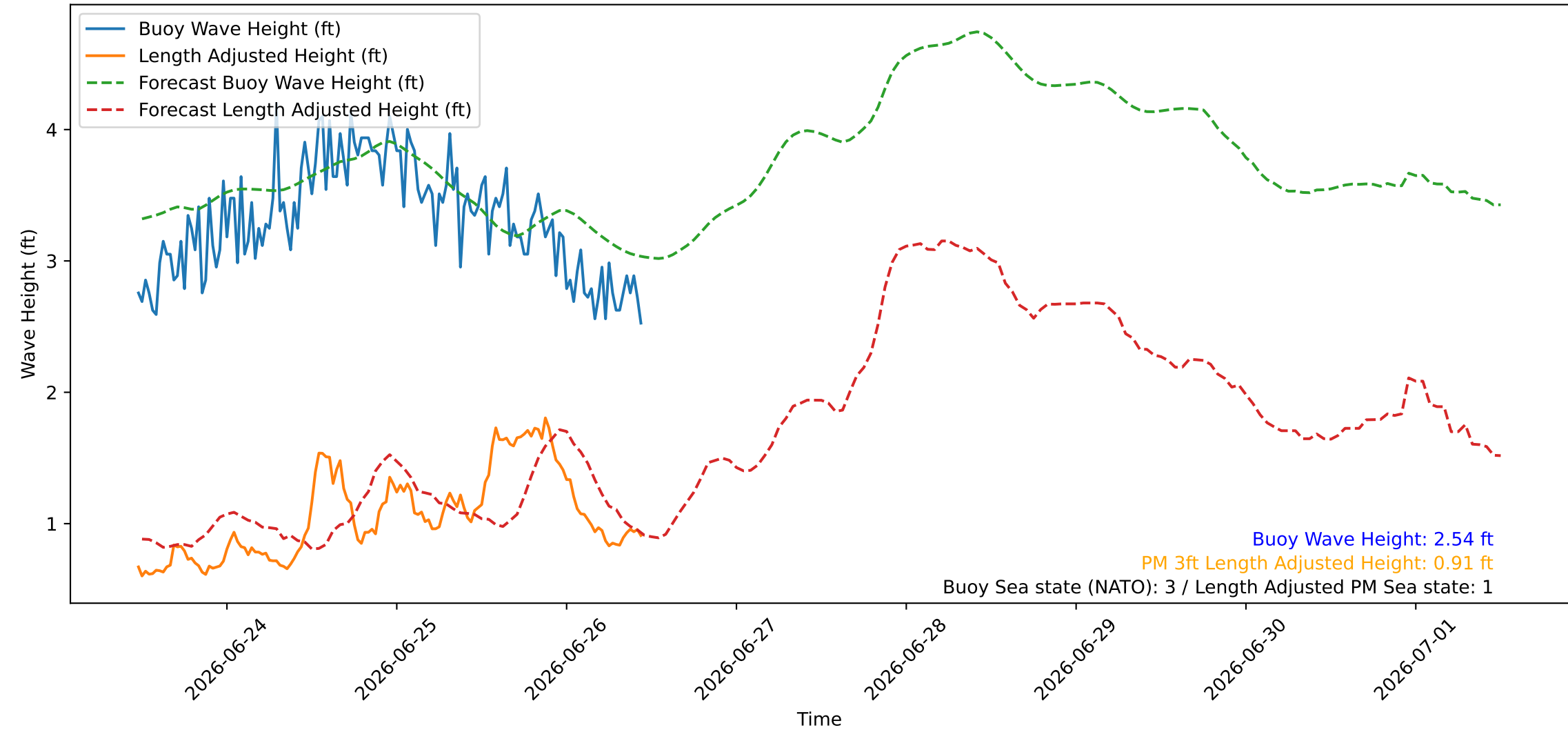
Wave Heights over Time for Green Beach at 2026-06-26 11:31:08
