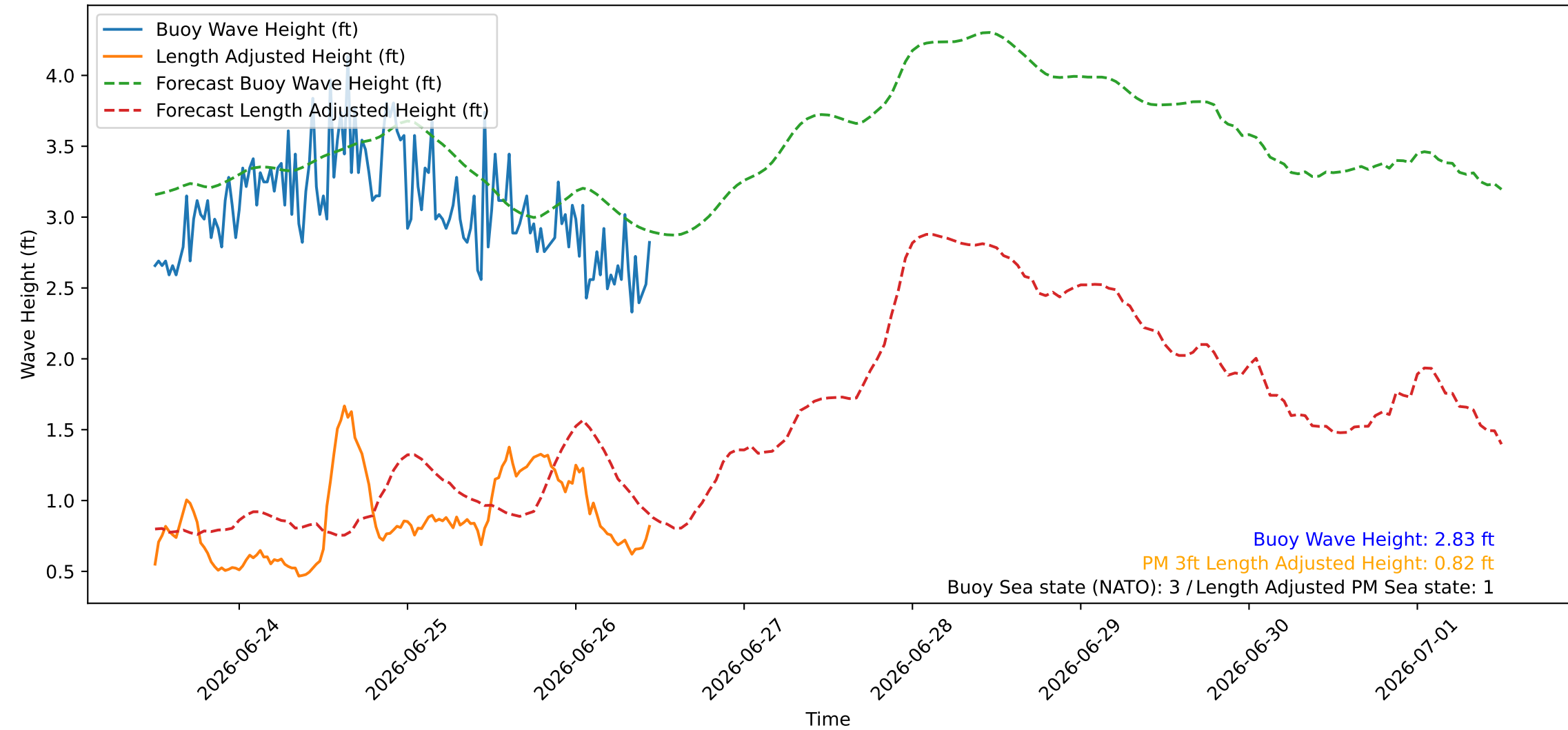
Wave Heights over Time for Red Beach at 2026-06-26 11:30:45
