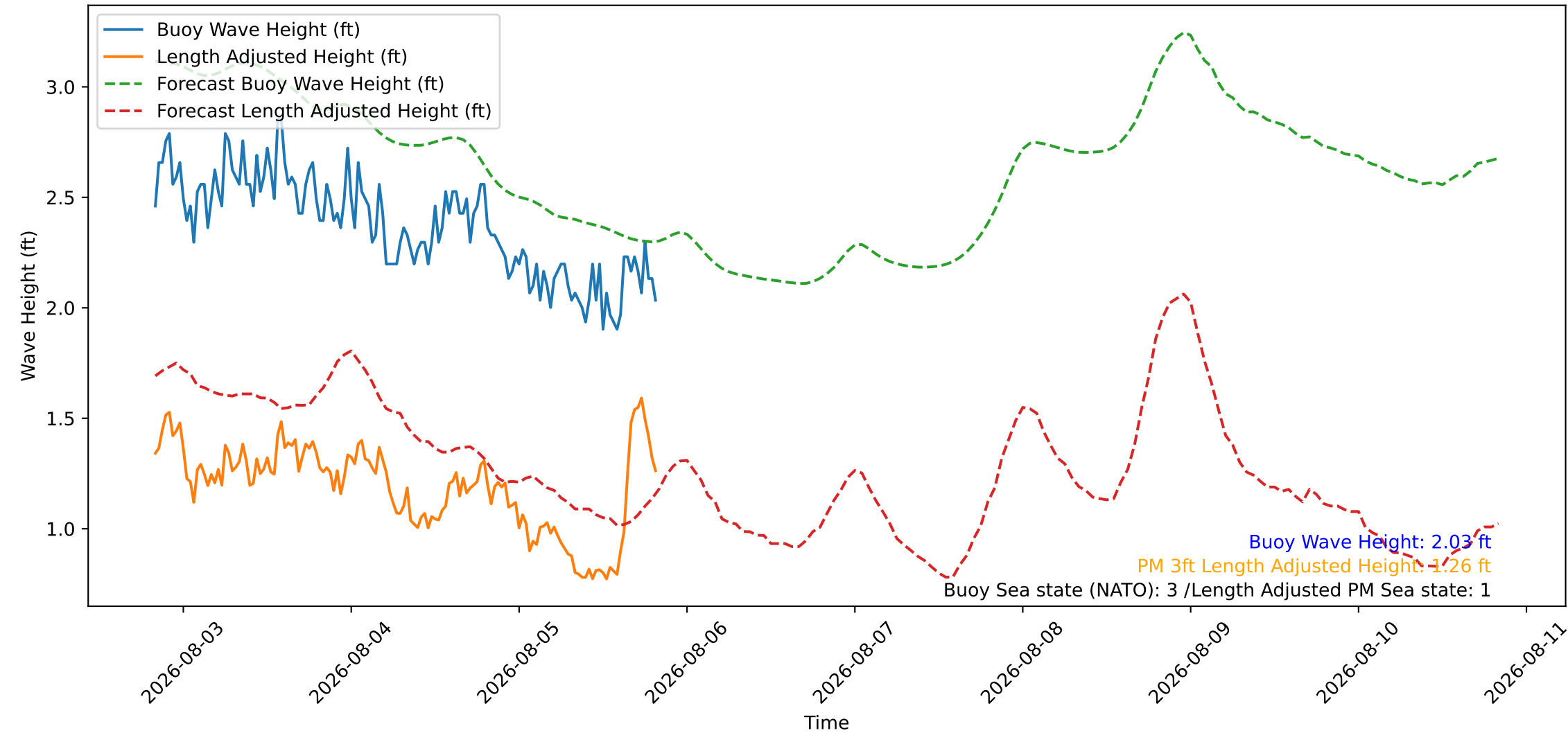
Wave Heights over Time for Oceanside Harbor at 2026-08-05 20:10:26
