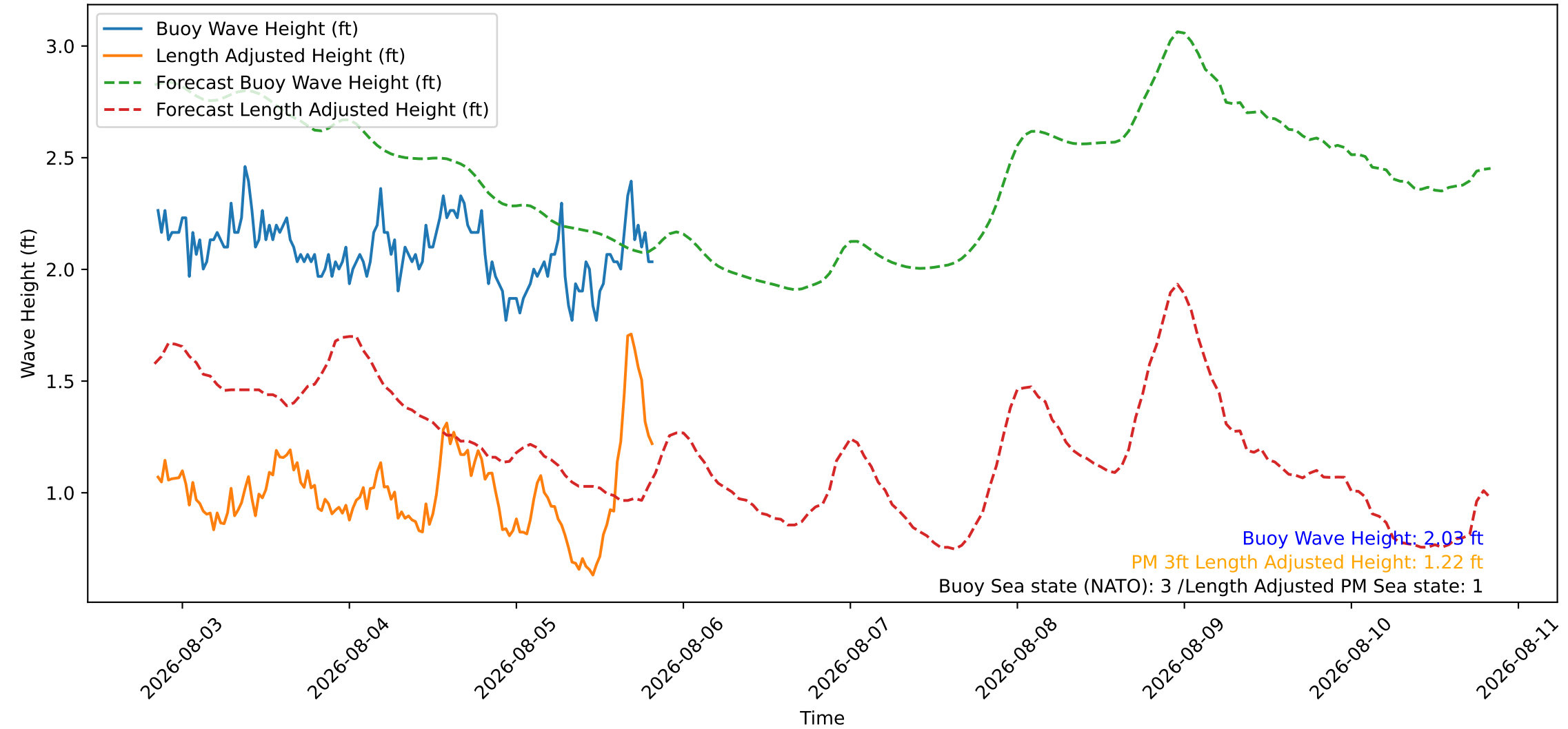
Wave Heights over Time for Red Beach at 2026-08-05 20:10:45
