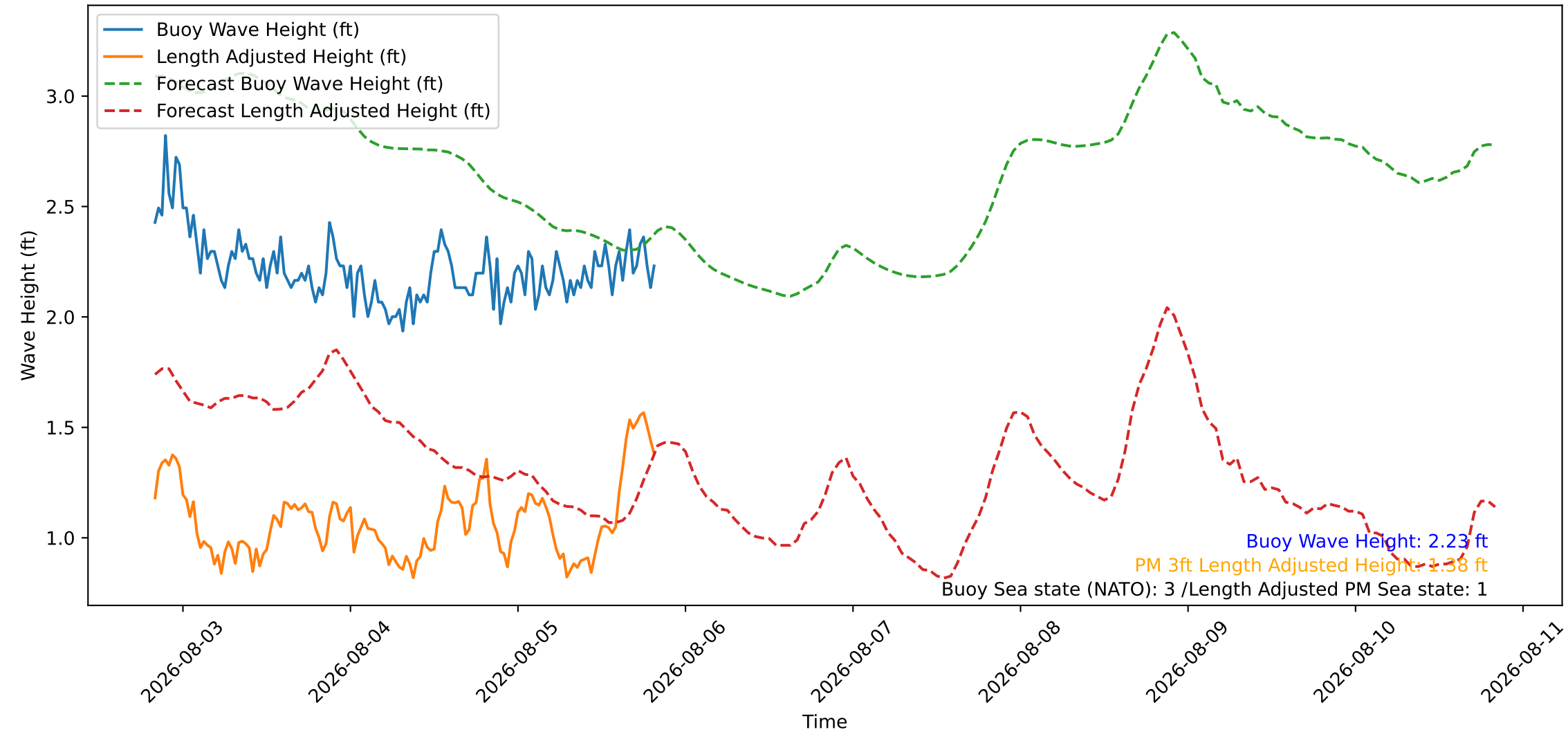
Wave Heights over Time for Green Beach at 2026-08-05 20:11:08
