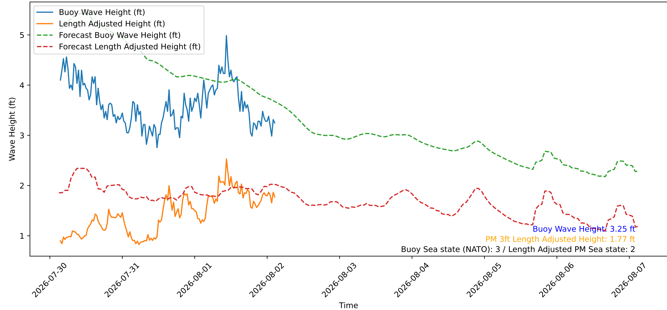
Wave Heights over Time for Green Beach at 2026-08-02 03:21:10
