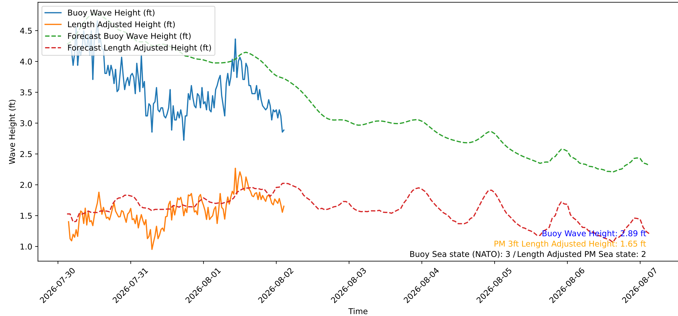
Wave Heights over Time for Oceanside Harbor at 2026-08-02 03:20:26
