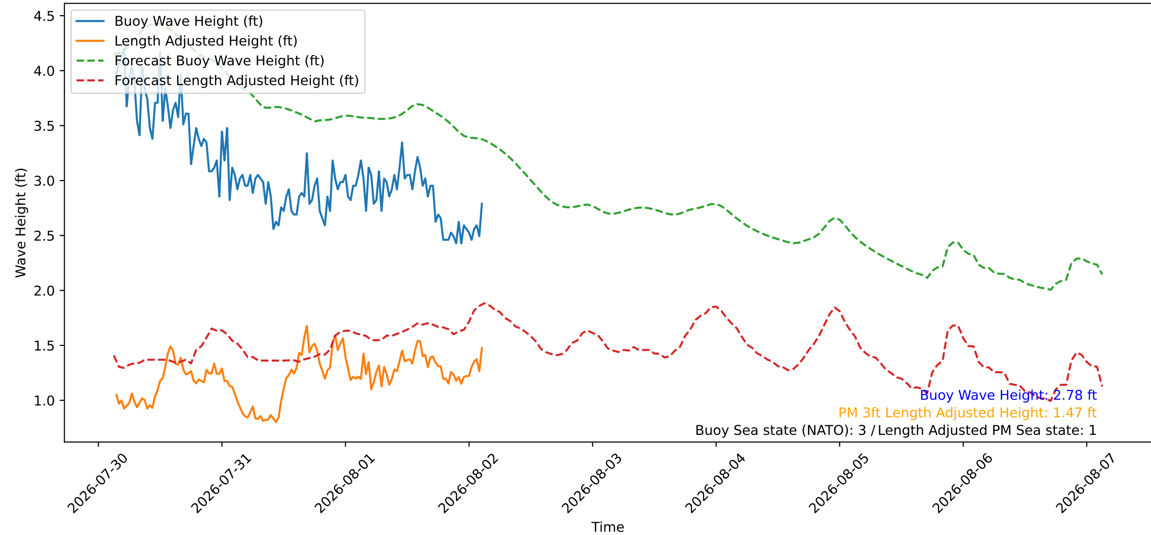
Wave Heights over Time for Red Beach at 2026-08-02 03:20:47
