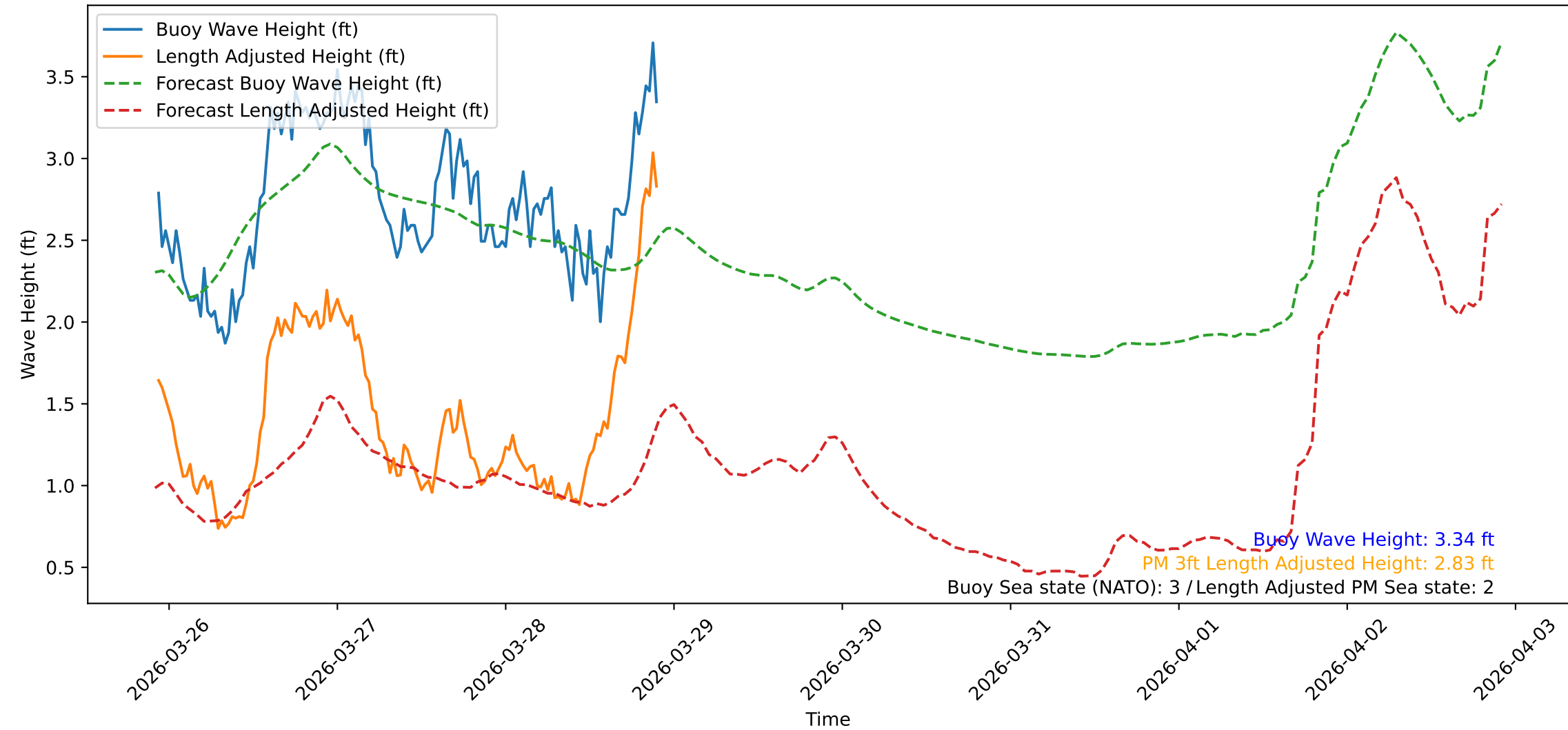
Wave Heights over Time for Green Beach at 2026-03-28 22:21:10
