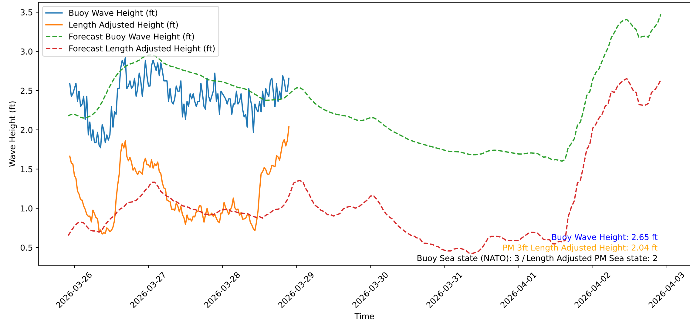
Wave Heights over Time for Oceanside Harbor at 2026-03-28 22:20:33
