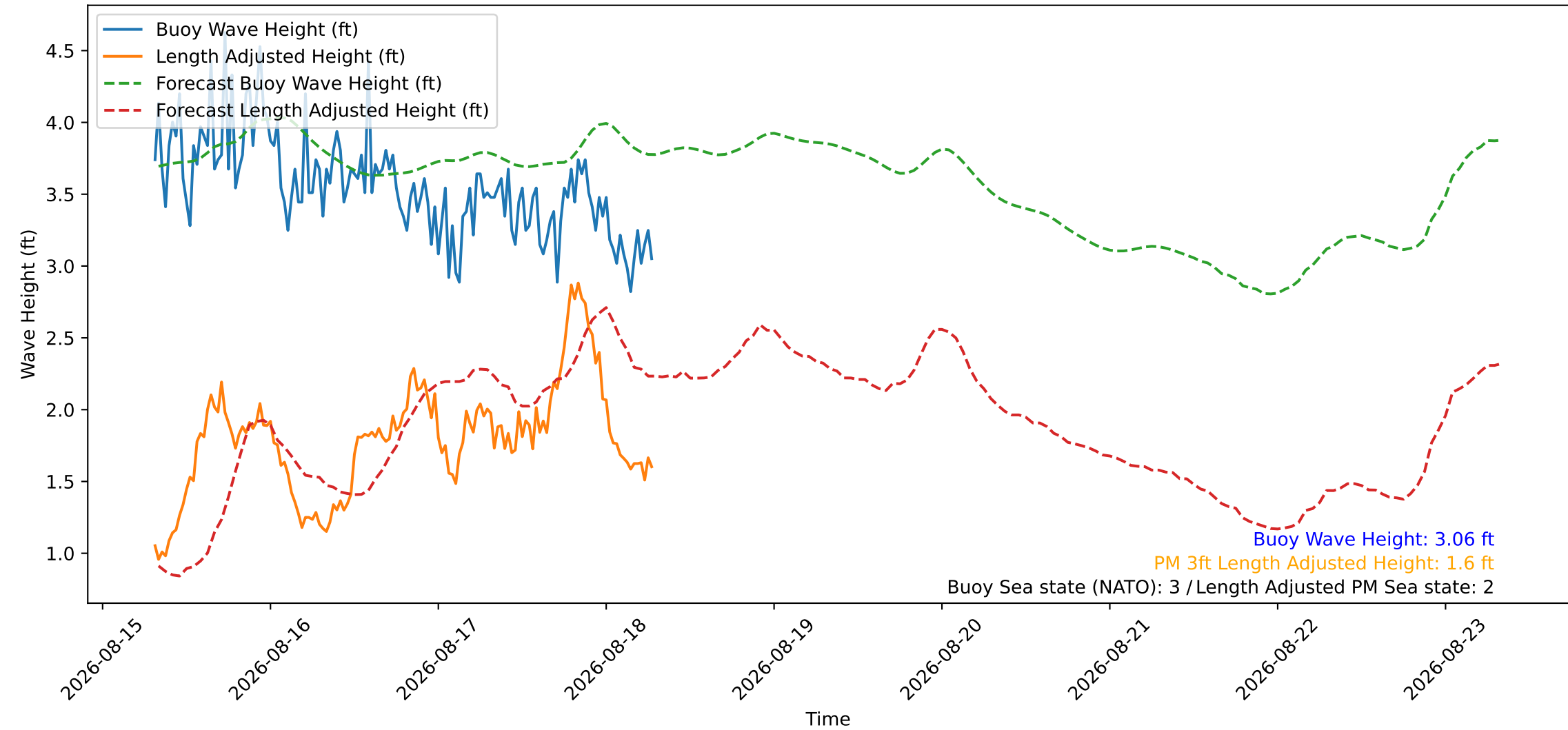
Wave Heights over Time for Oceanside Harbor at 2026-08-18 07:30:26
