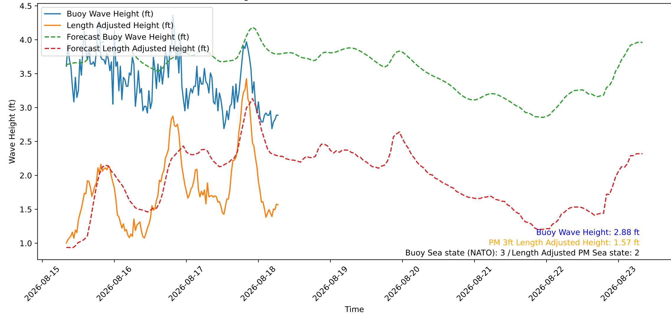
Wave Heights over Time for Green Beach at 2026-08-18 07:31:08
