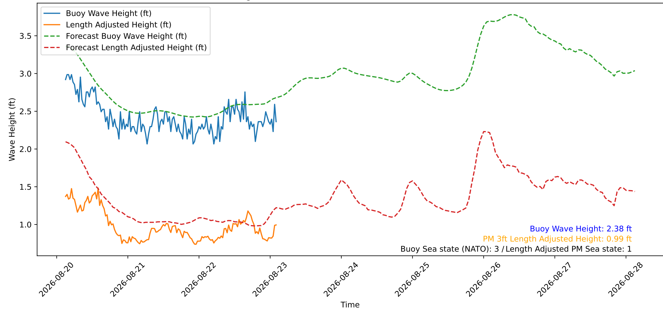
Wave Heights over Time for Red Beach at 2026-08-23 02:50:50
