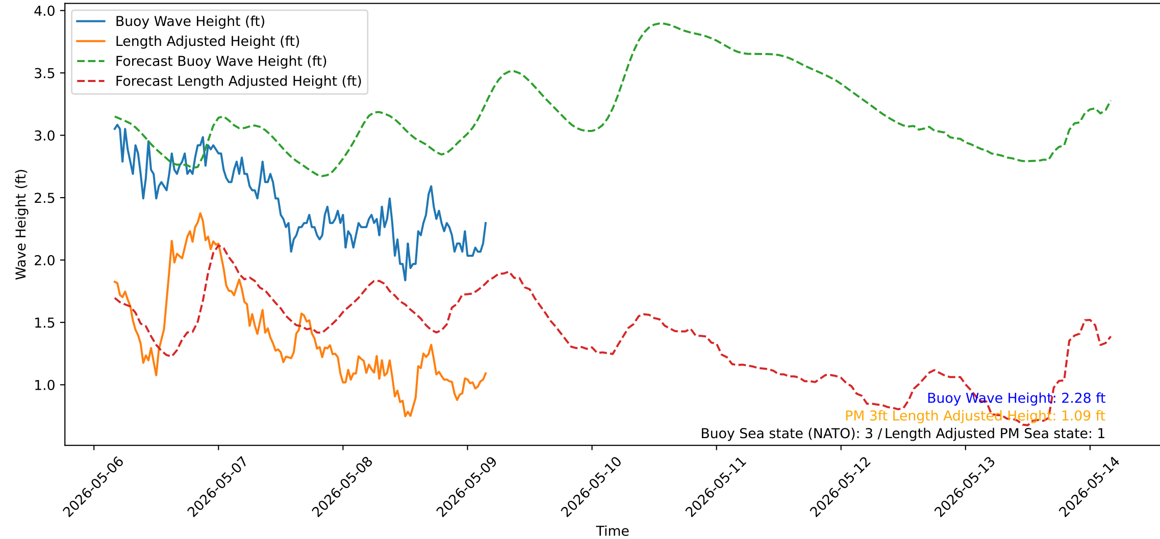
Wave Heights over Time for Green Beach at 2026-05-09 04:11:12
