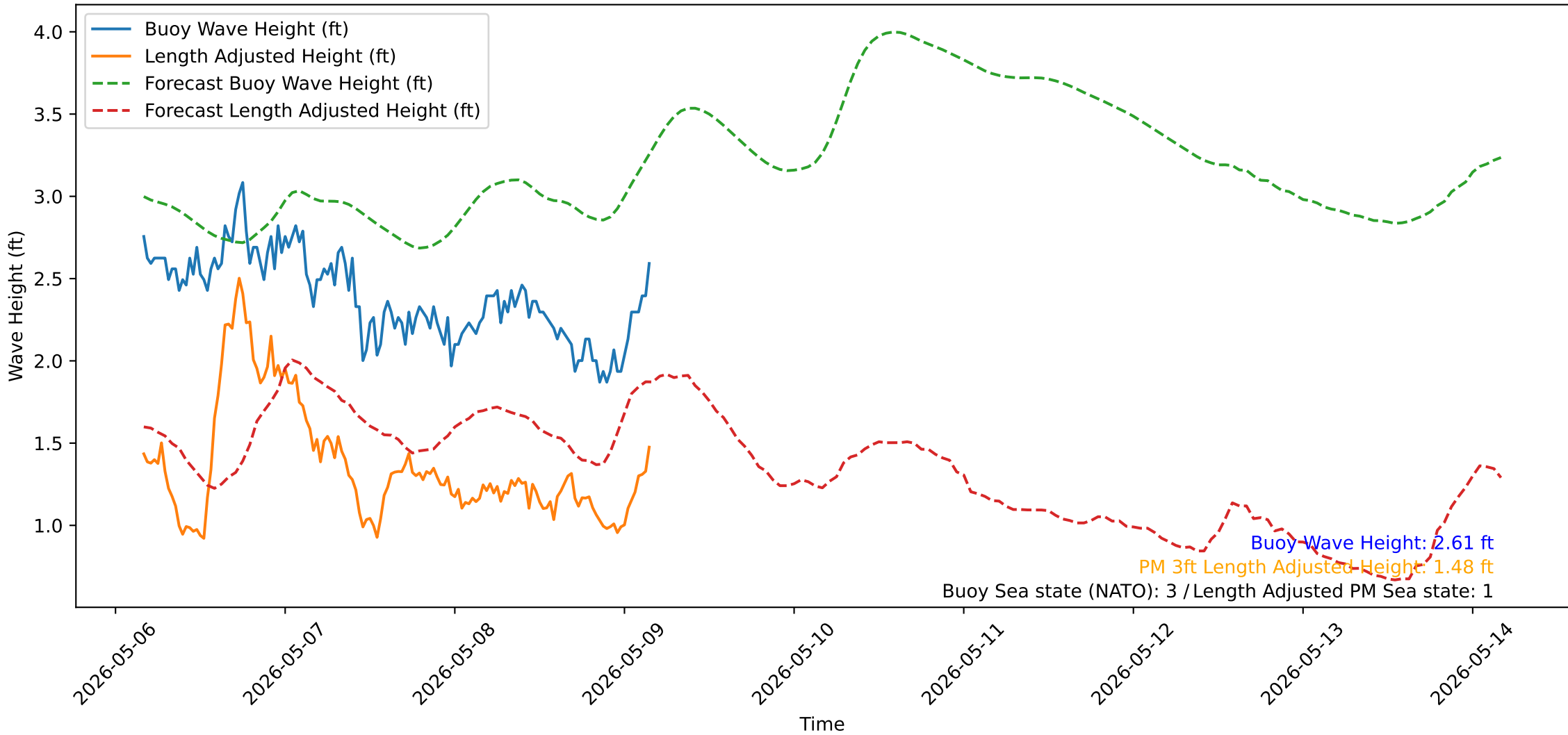
Wave Heights over Time for Oceanside Harbor at 2026-05-09 04:10:31
