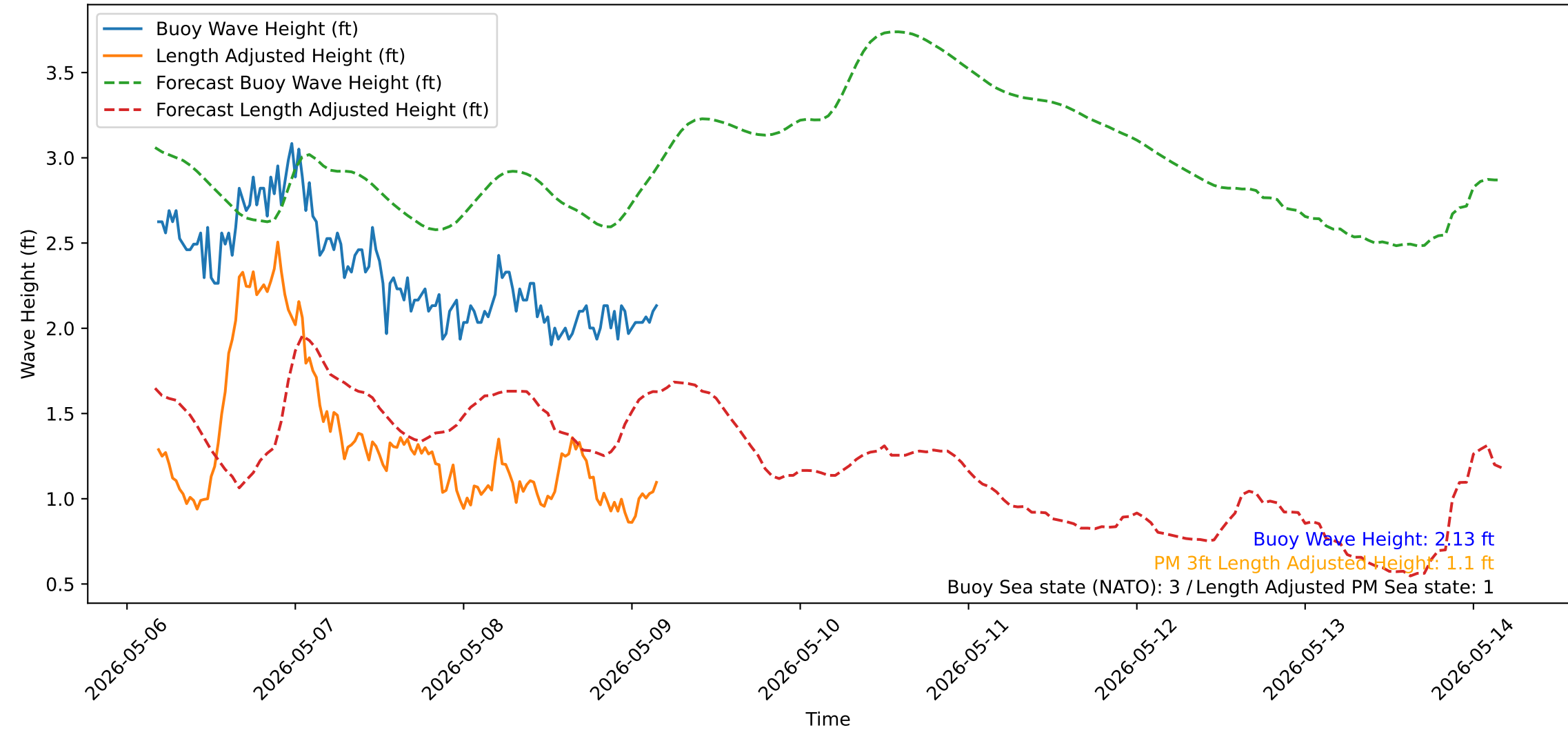
Wave Heights over Time for Red Beach at 2026-05-09 04:10:50
