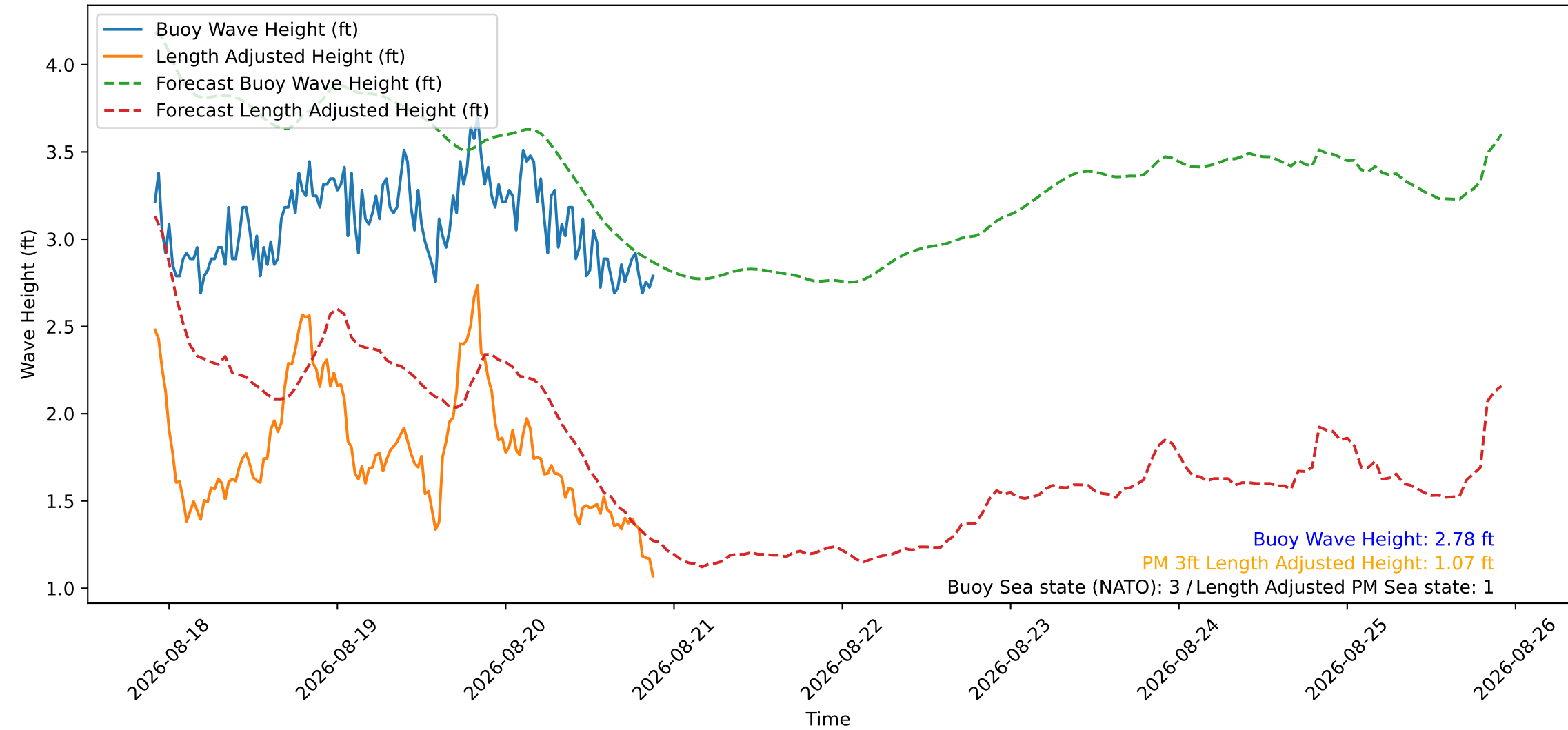
Wave Heights over Time for Green Beach at 2026-08-20 21:51:11
