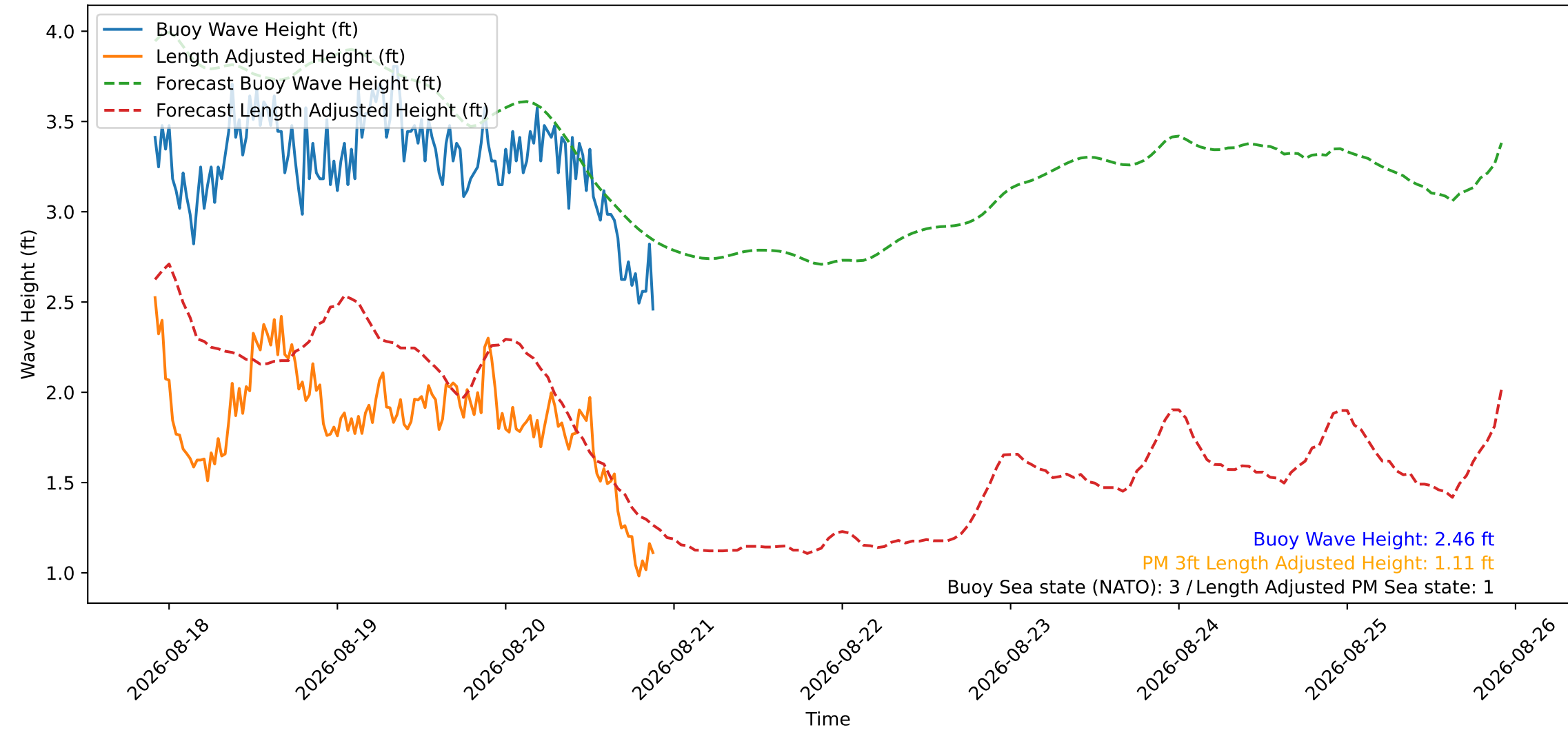
Wave Heights over Time for Oceanside Harbor at 2026-08-20 21:50:26
