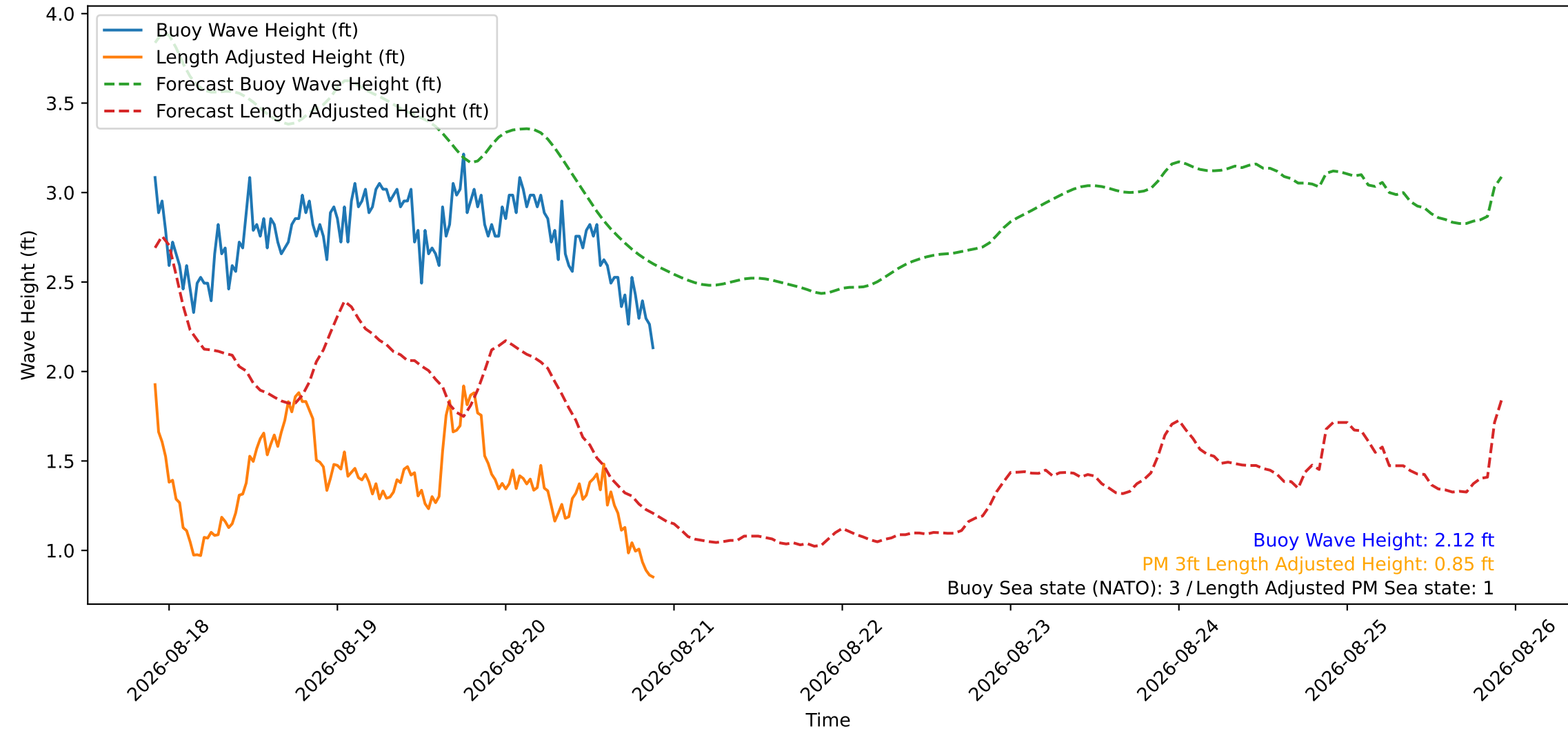
Wave Heights over Time for Red Beach at 2026-08-20 21:50:47
