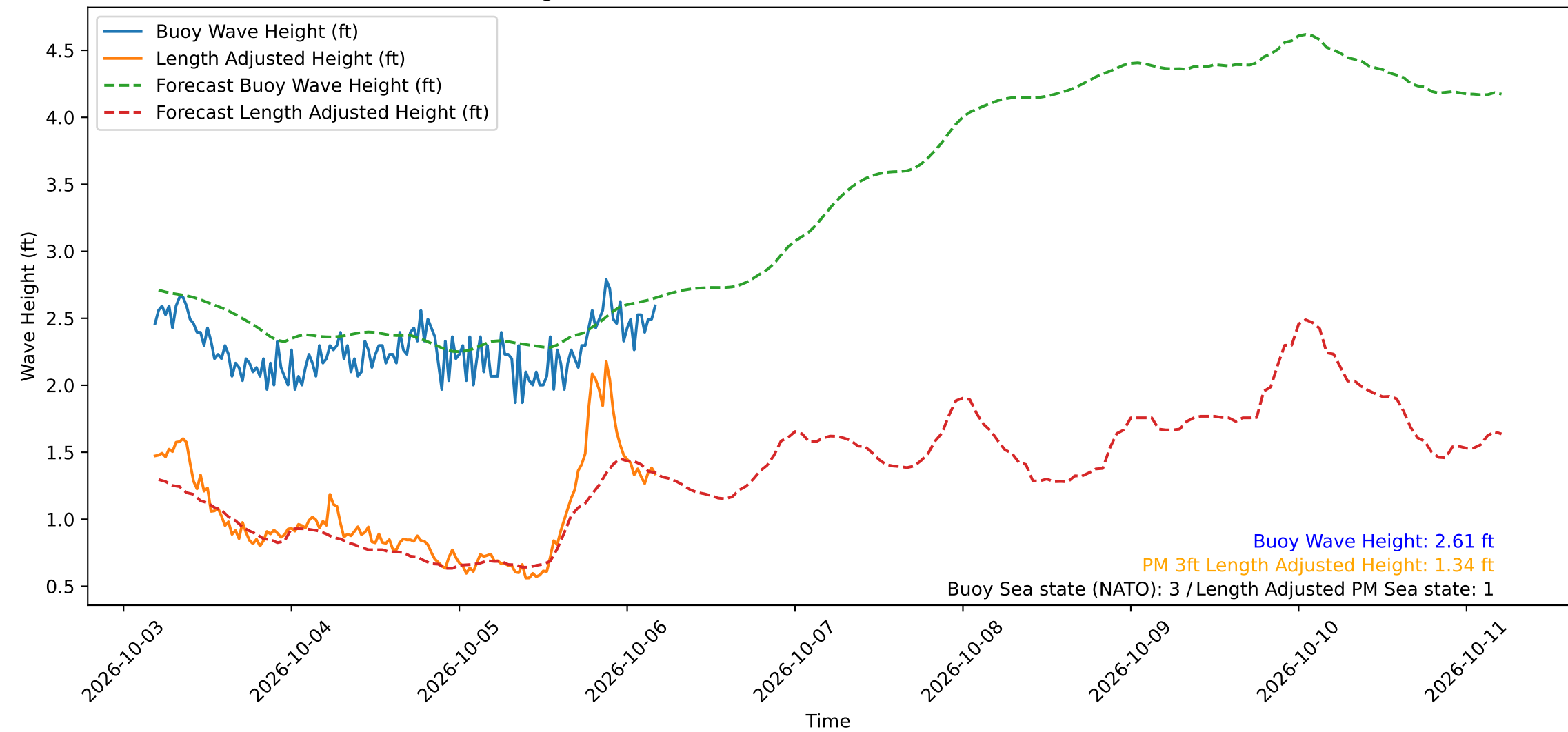
Wave Heights over Time for Oceanside Harbor at 2026-10-06 04:40:29
