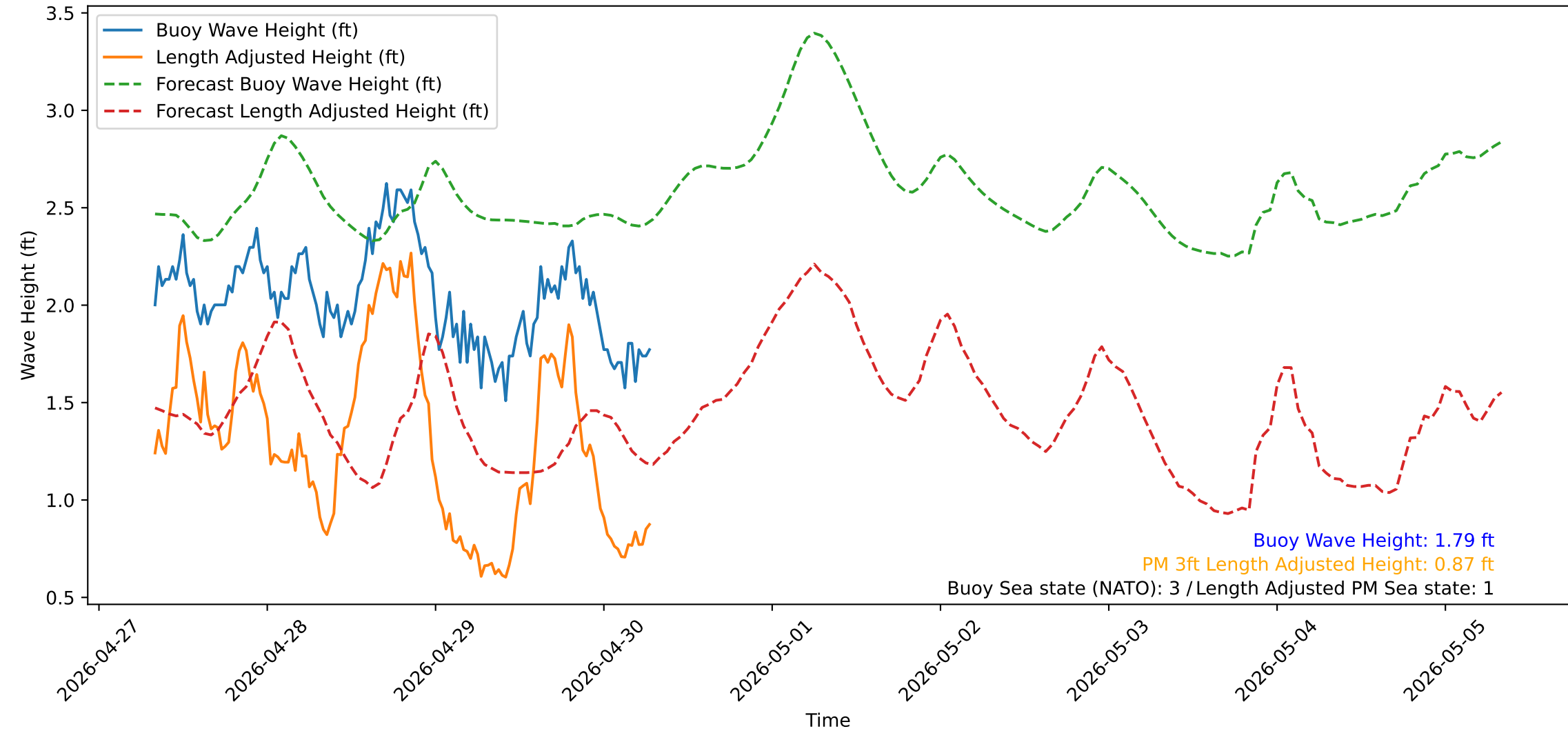
Wave Heights over Time for Red Beach at 2026-04-30 07:30:50
