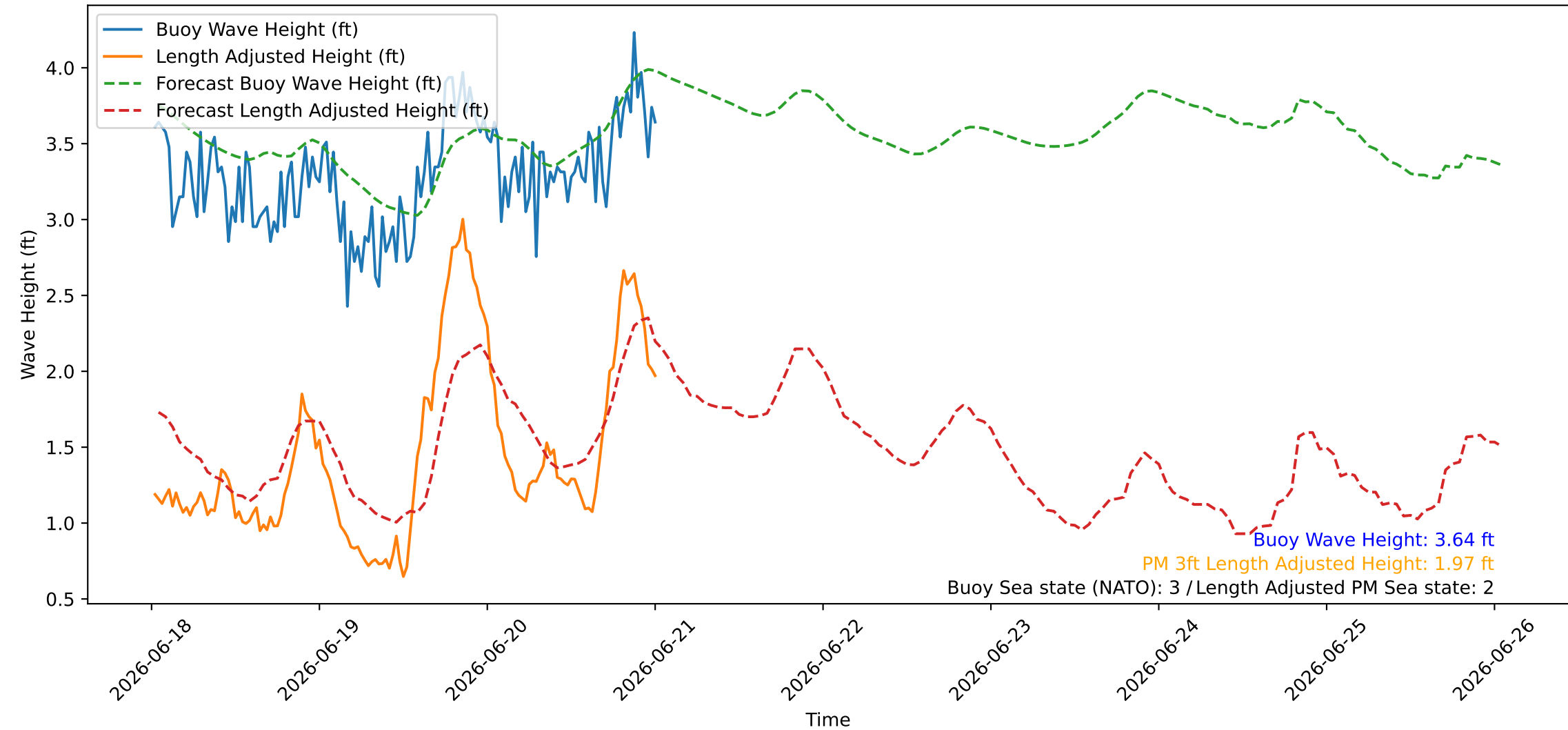
Wave Heights over Time for Green Beach at 2026-06-21 00:41:08
