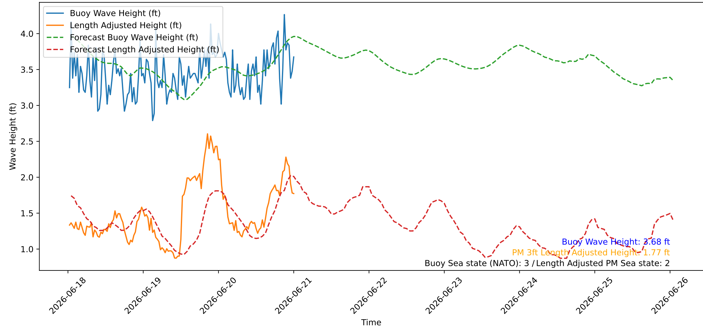
Wave Heights over Time for Oceanside Harbor at 2026-06-21 00:40:26
