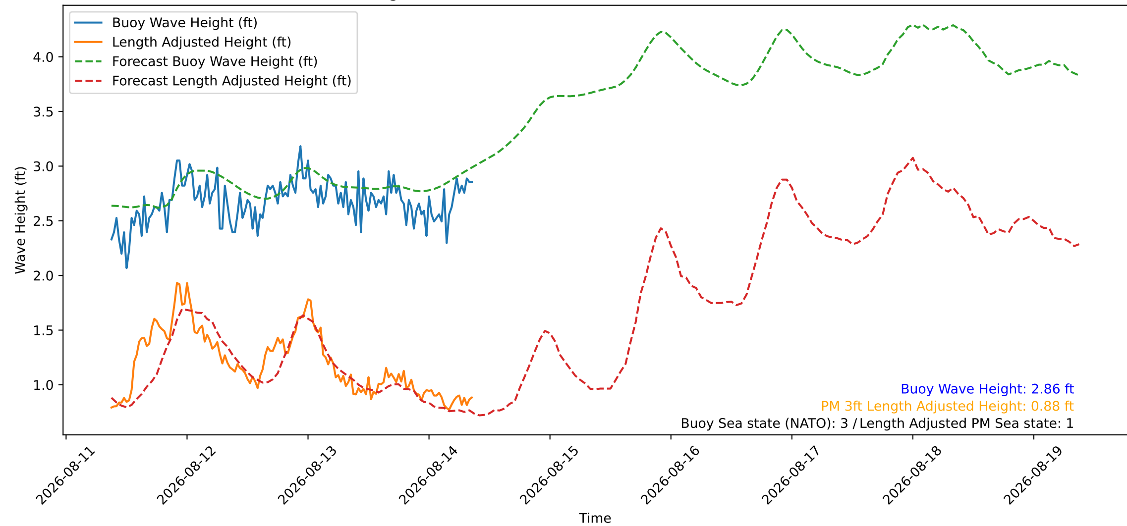
Wave Heights over Time for Oceanside Harbor at 2026-08-14 09:10:26
