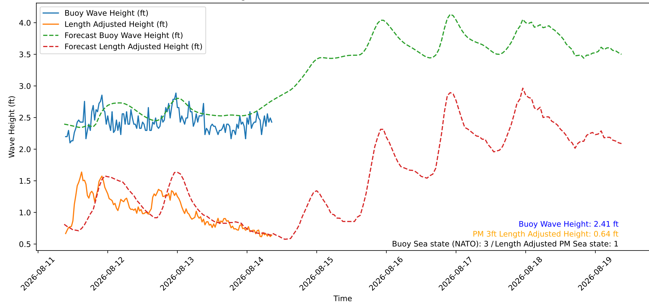
Wave Heights over Time for Red Beach at 2026-08-14 09:10:45
