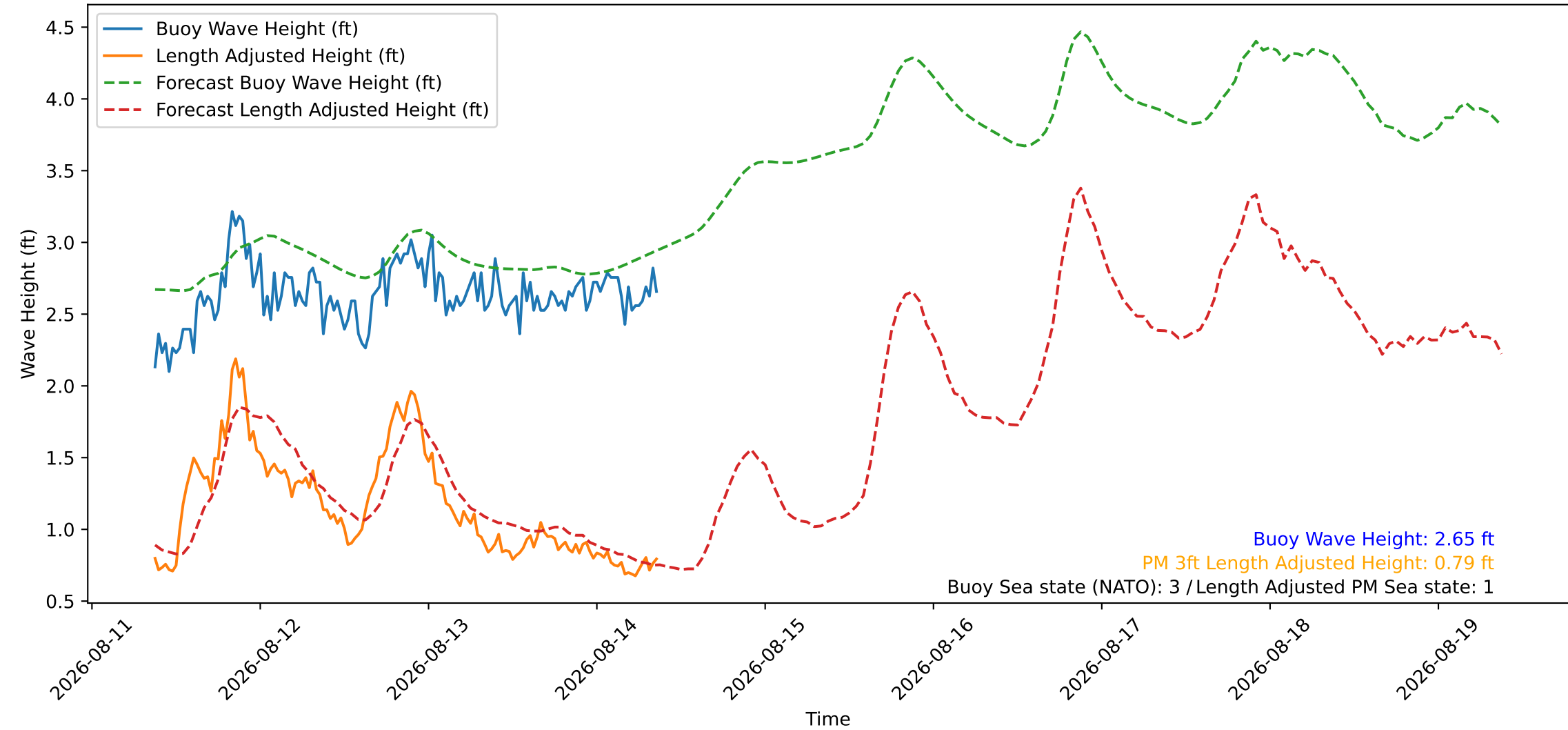
Wave Heights over Time for Green Beach at 2026-08-14 09:11:07
