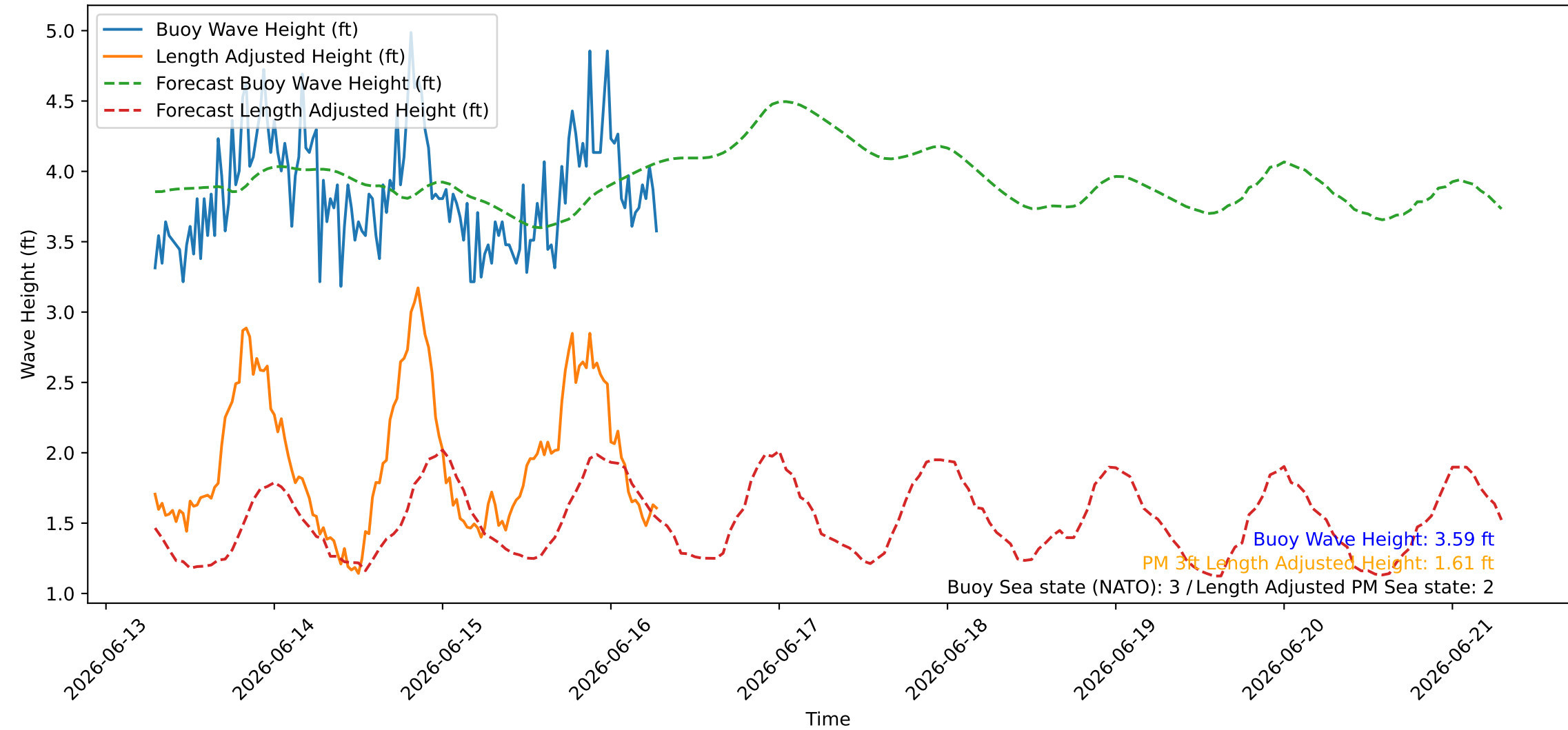
Wave Heights over Time for Oceanside Harbor at 2026-06-16 07:10:27
