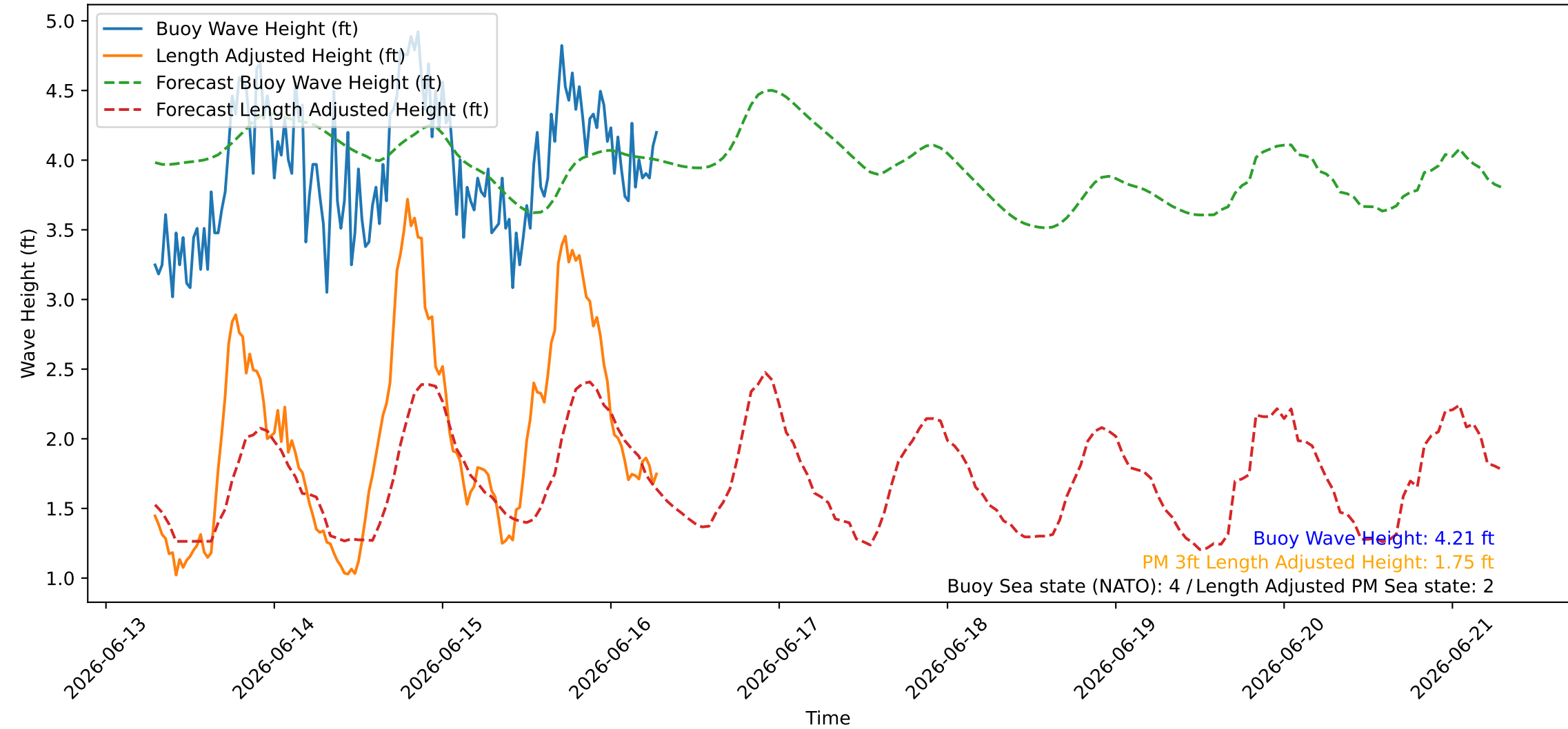
Wave Heights over Time for Green Beach at 2026-06-16 07:11:09
