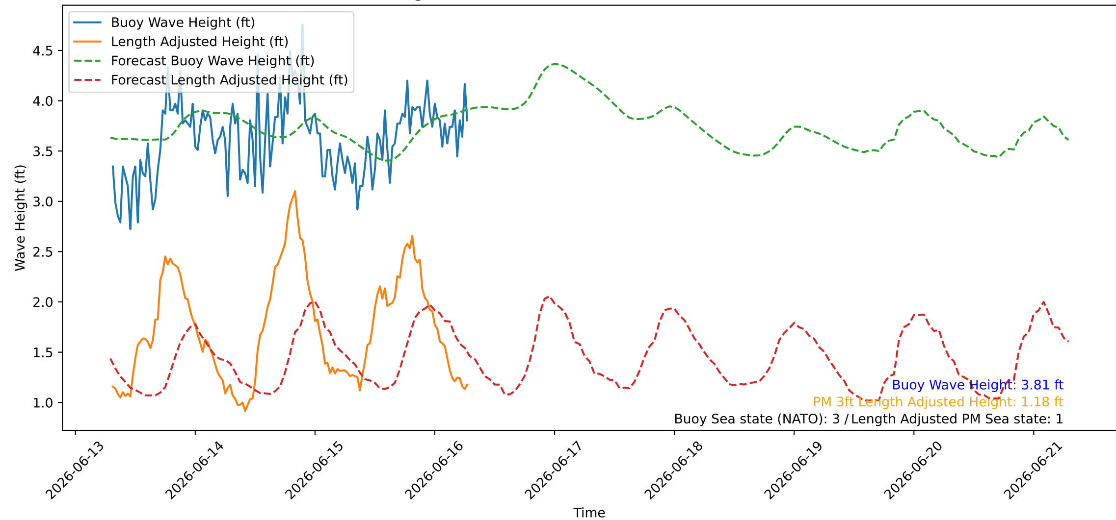
Wave Heights over Time for Red Beach at 2026-06-16 07:10:46
