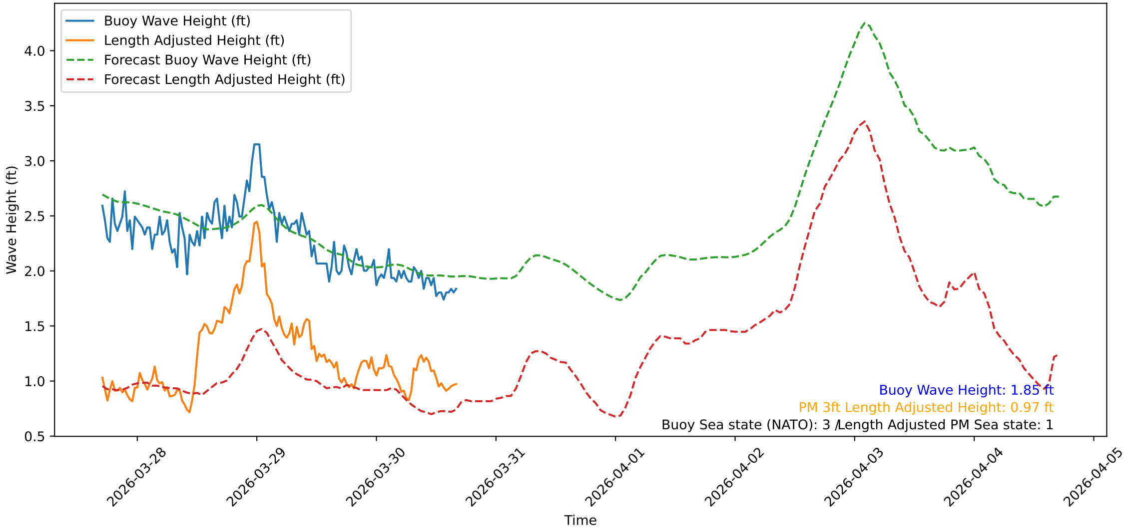
Wave Heights over Time for Oceanside Harbor at 2026-03-30 16:50:31
