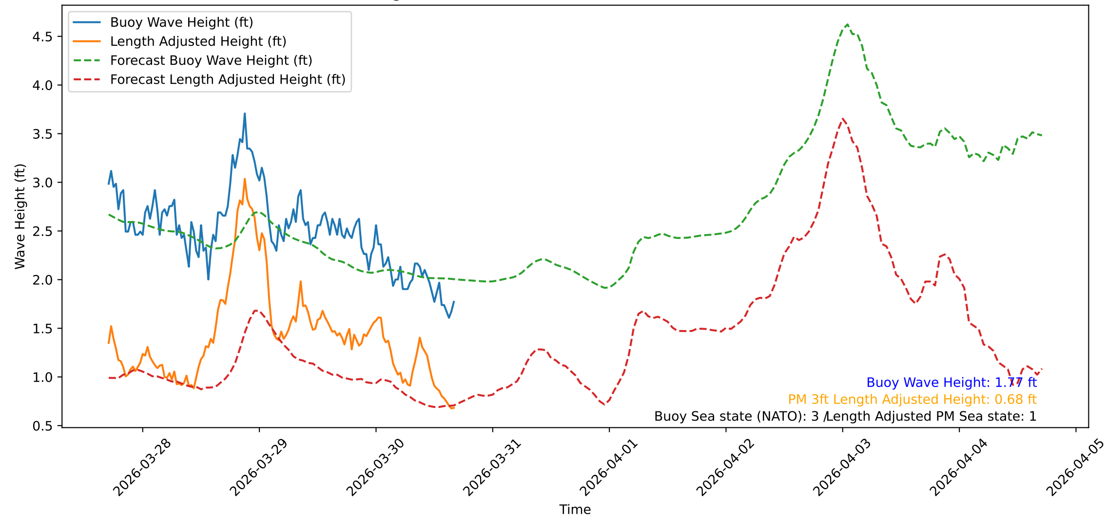
Wave Heights over Time for Green Beach at 2026-03-30 16:51:09
