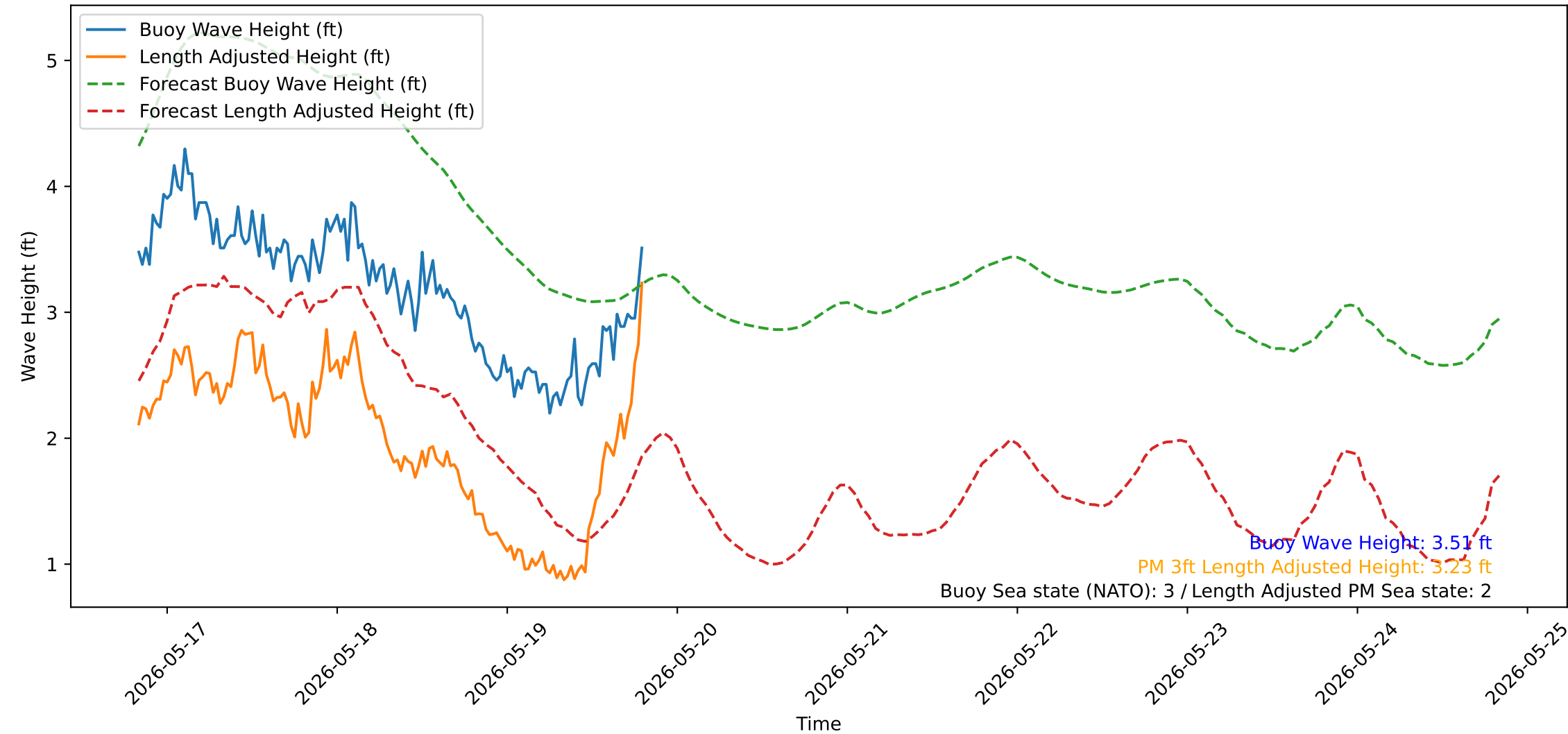
Wave Heights over Time for Oceanside Harbor at 2026-05-19 19:50:31
