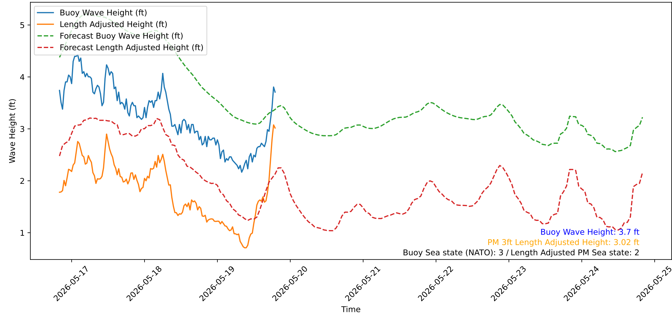
Wave Heights over Time for Green Beach at 2026-05-19 19:51:15
