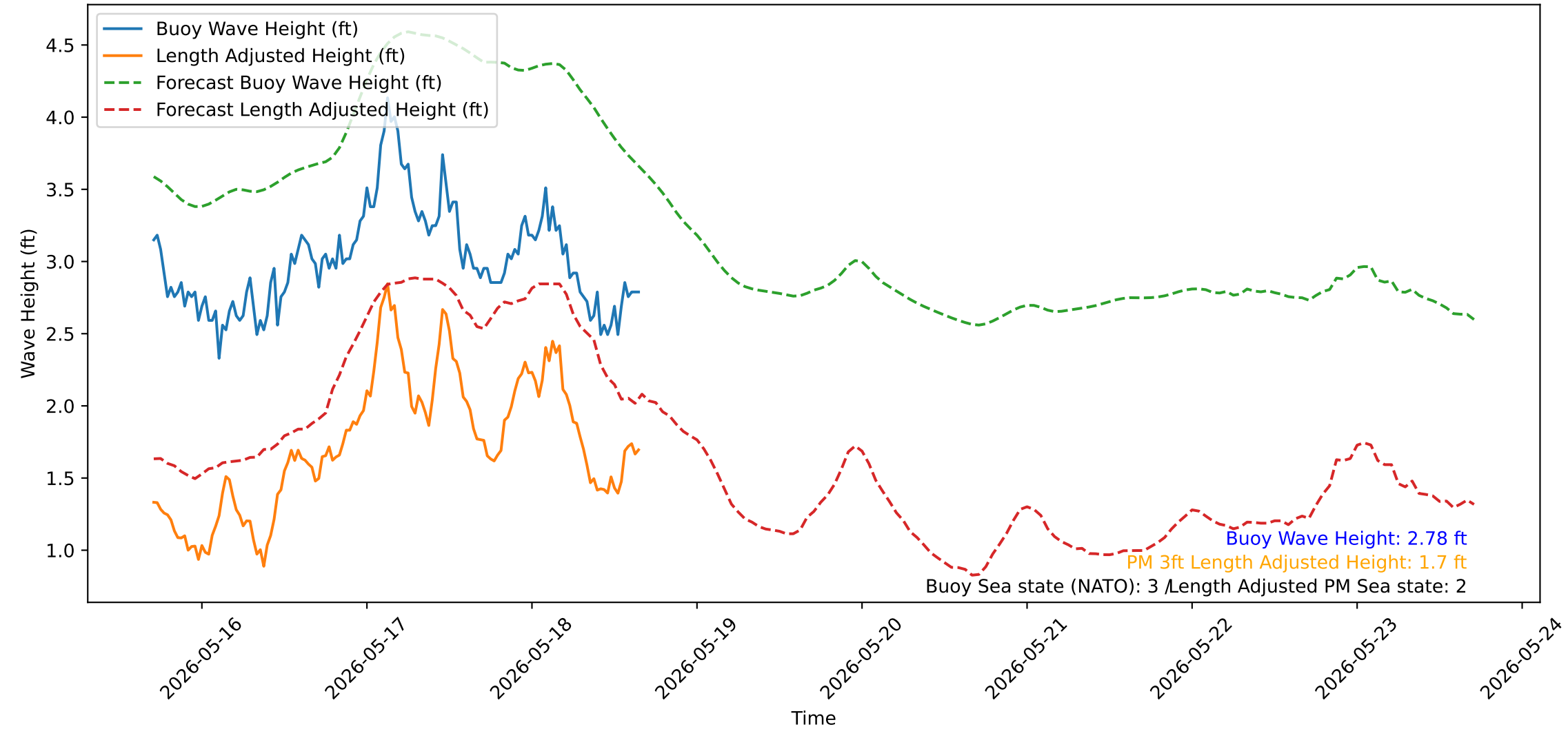
Wave Heights over Time for Red Beach at 2026-05-18 16:30:51
