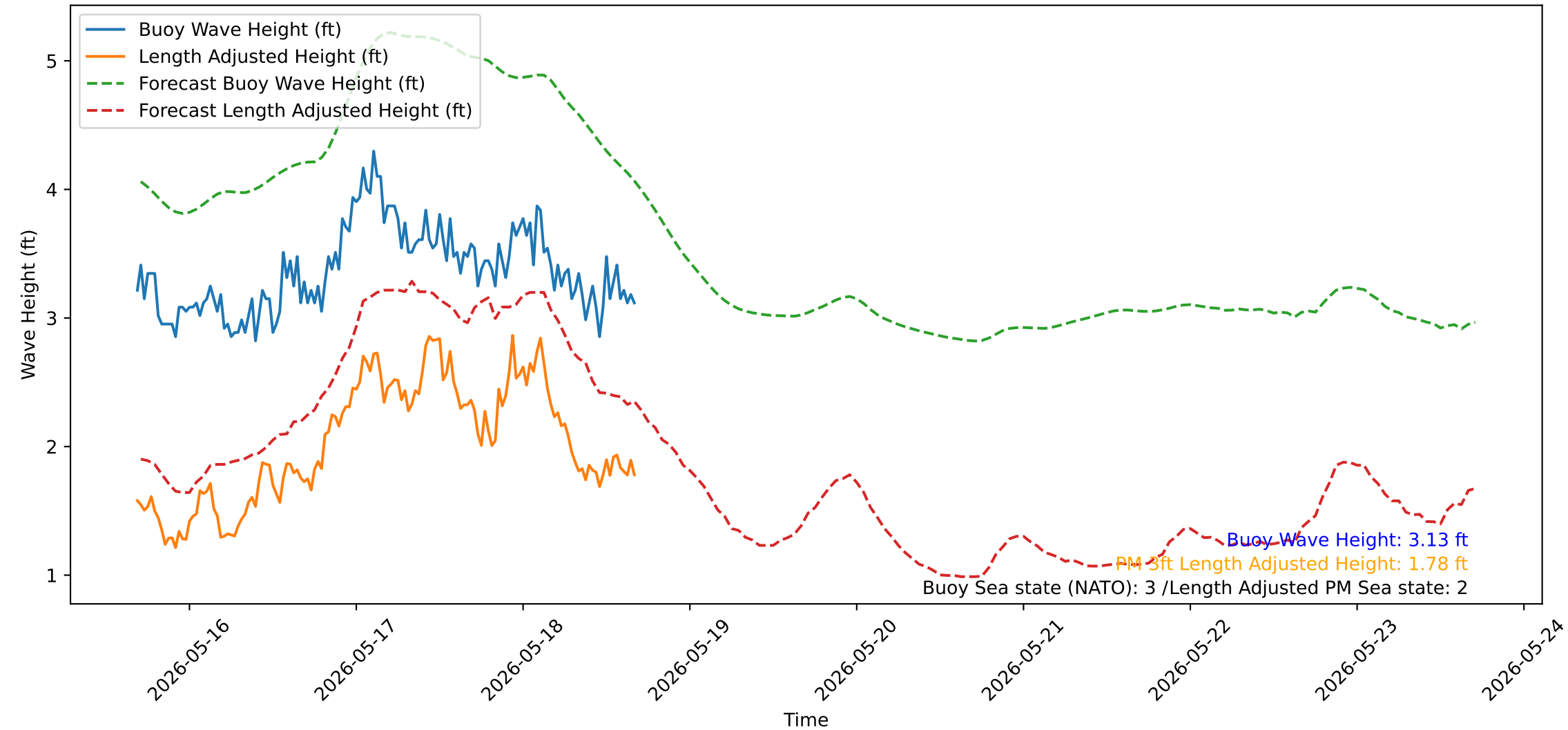
Wave Heights over Time for Oceanside Harbor at 2026-05-18 16:30:31
