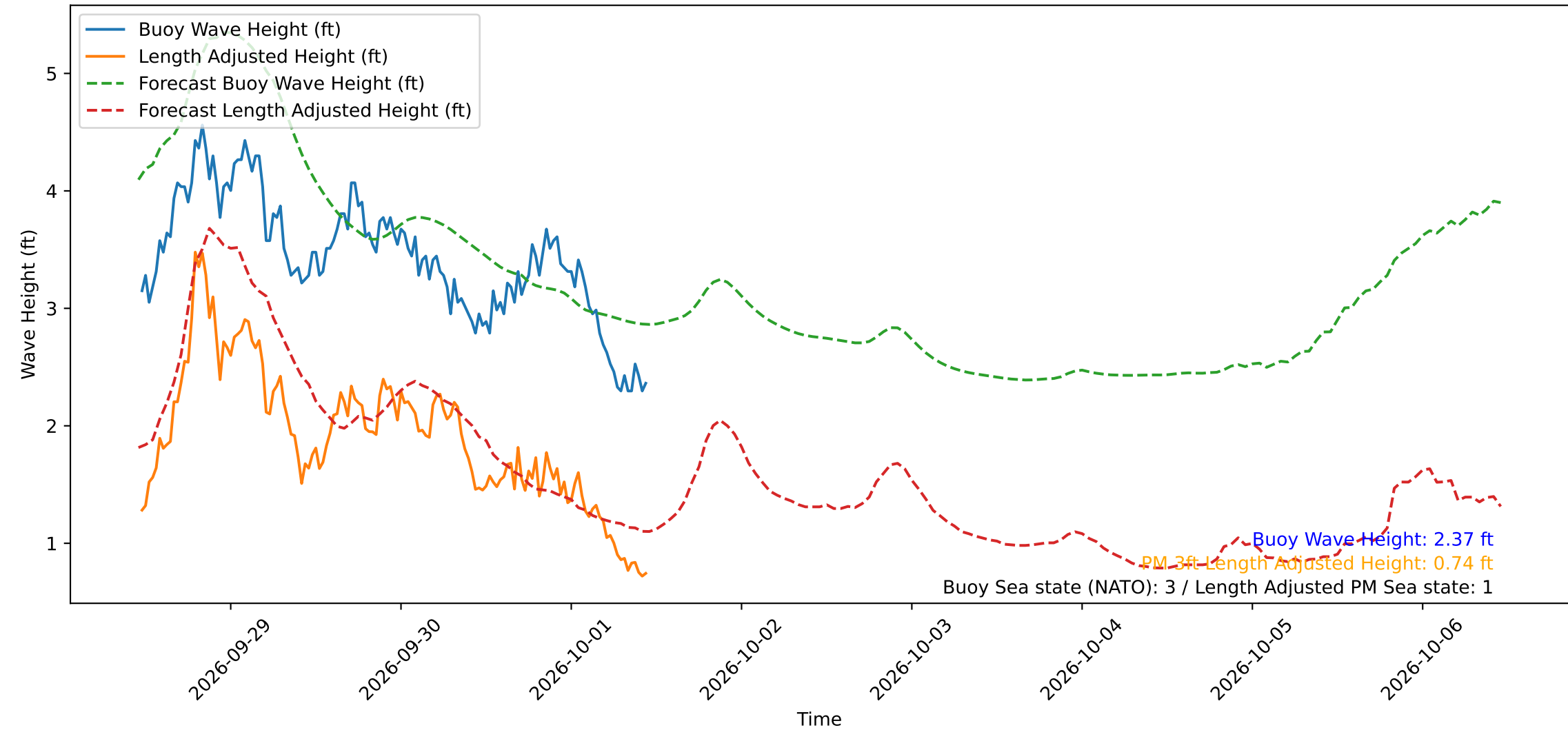
Wave Heights over Time for Green Beach at 2026-10-01 11:21:15
