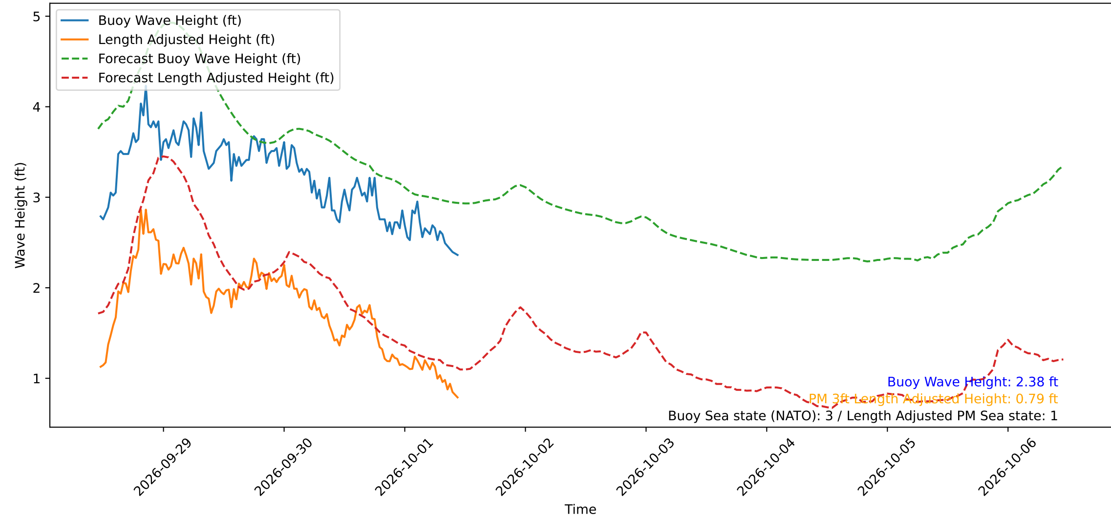
Wave Heights over Time for Oceanside Harbor at 2026-10-01 11:20:30
