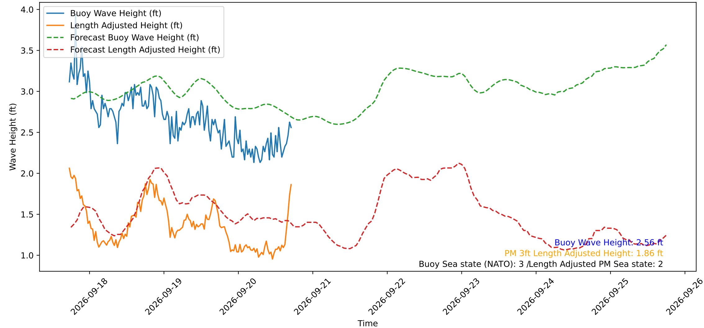
Wave Heights over Time for Oceanside Harbor at 2026-09-20 17:40:29
