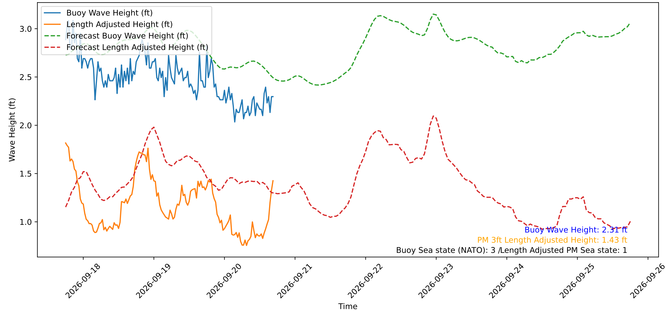
Wave Heights over Time for Red Beach at 2026-09-20 17:40:49
