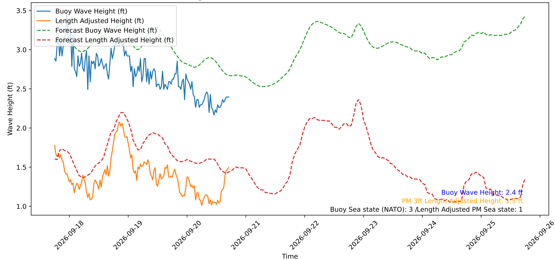
Wave Heights over Time for Green Beach at 2026-09-20 17:41:11
