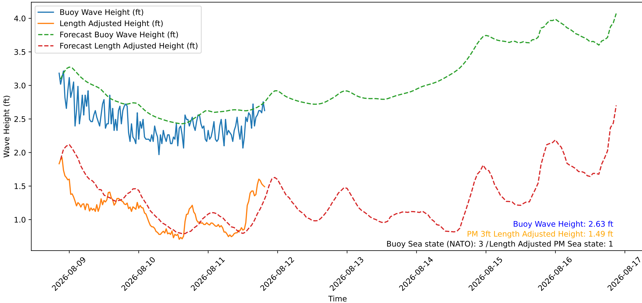
Wave Heights over Time for Oceanside Harbor at 2026-08-11 20:30:26
