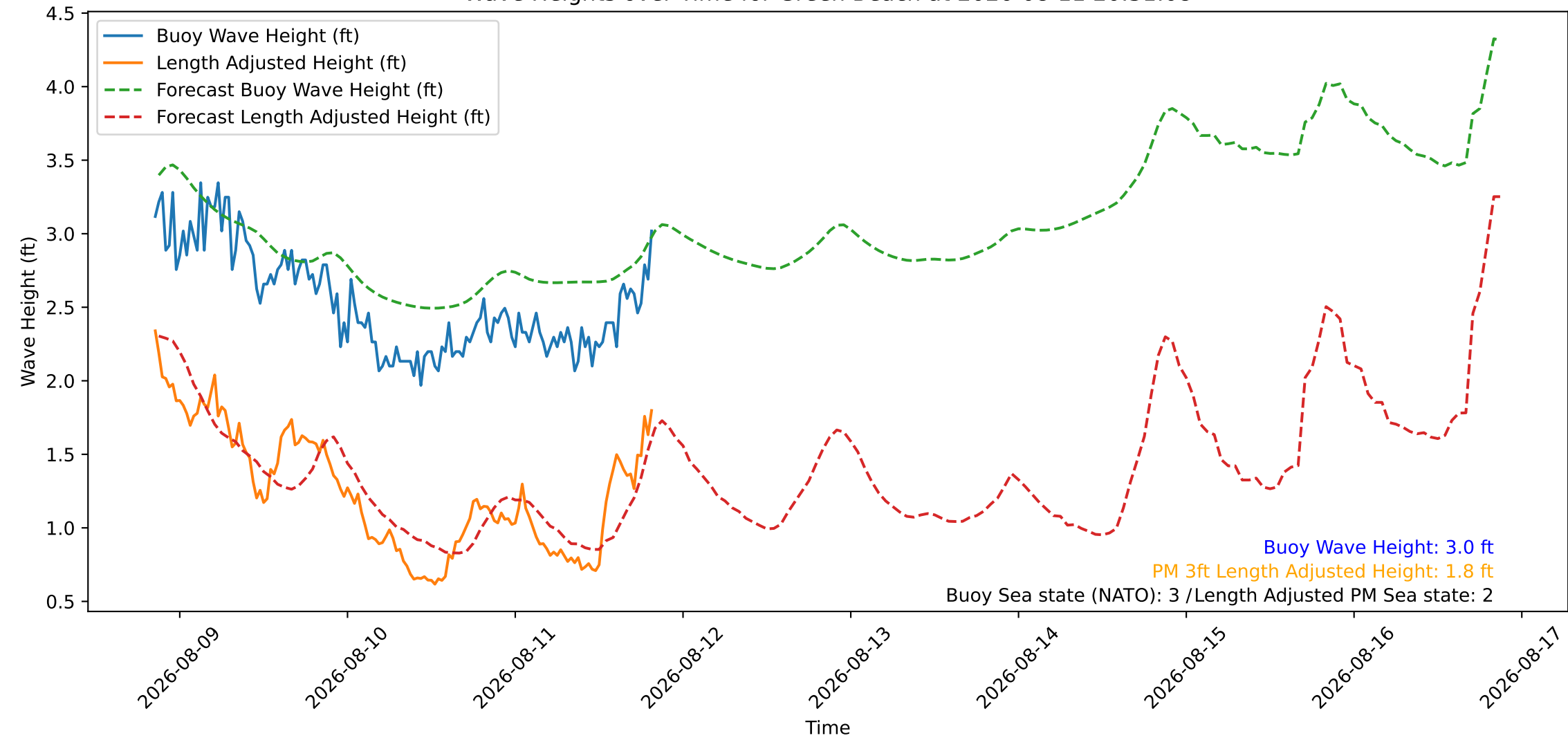
Wave Heights over Time for Green Beach at 2026-08-11 20:31:08
