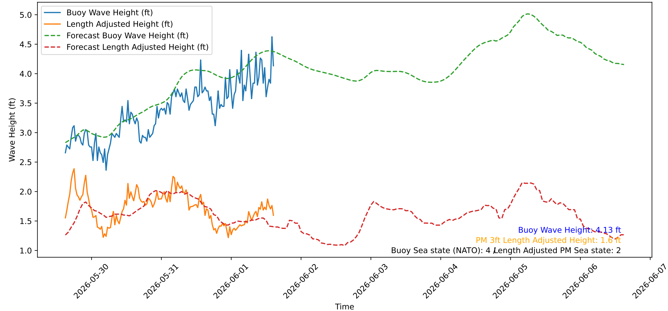
Wave Heights over Time for Oceanside Harbor at 2026-06-01 15:10:26
