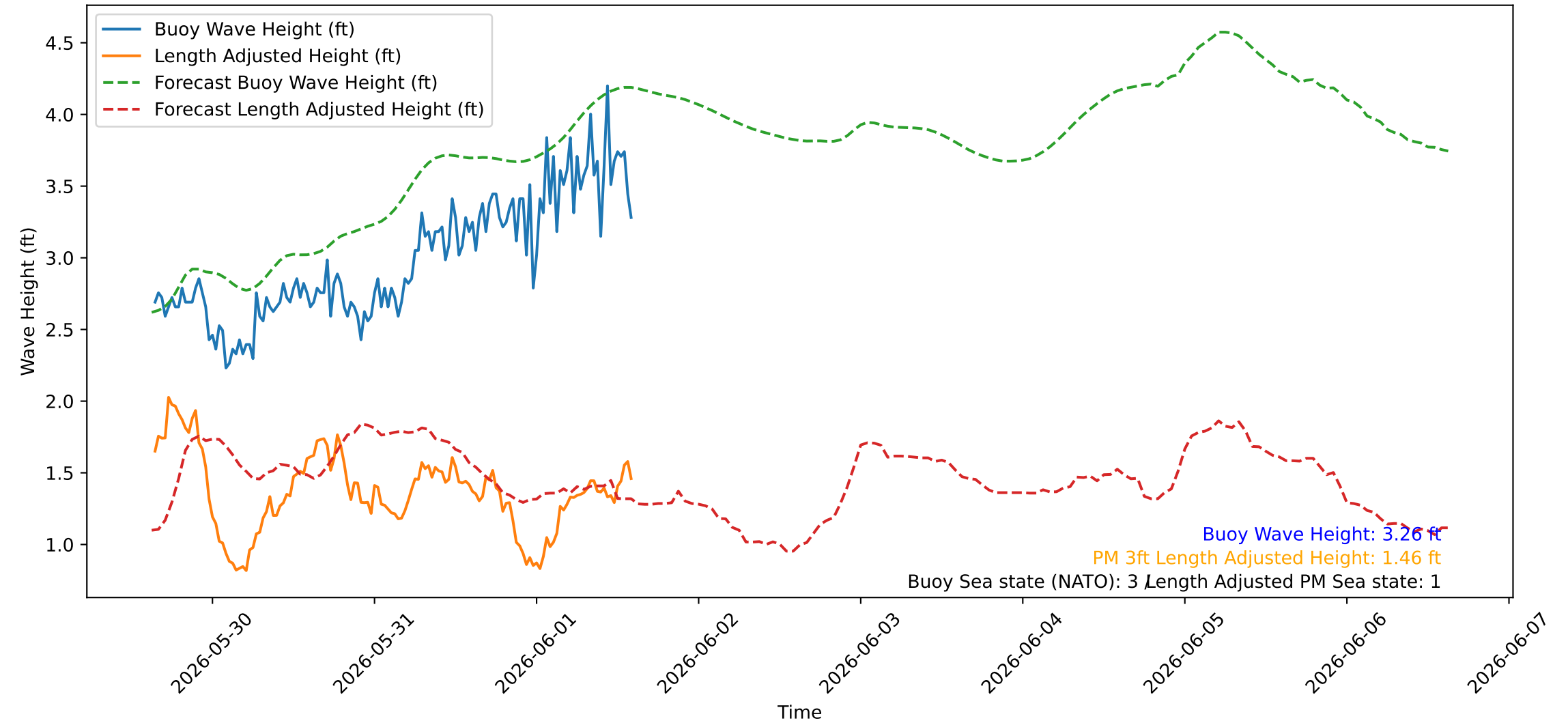
Wave Heights over Time for Red Beach at 2026-06-01 15:10:45
