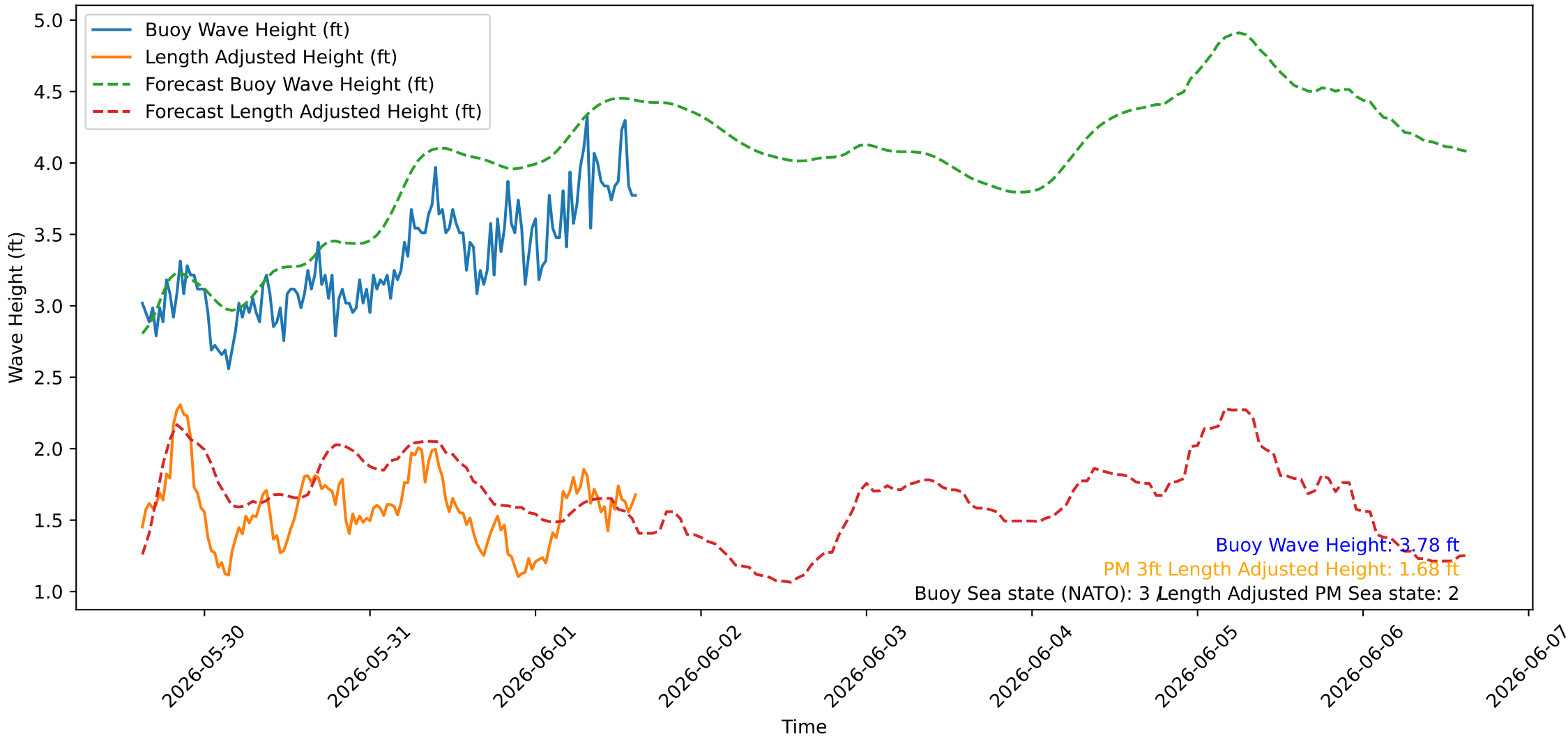
Wave Heights over Time for Green Beach at 2026-06-01 15:11:07
