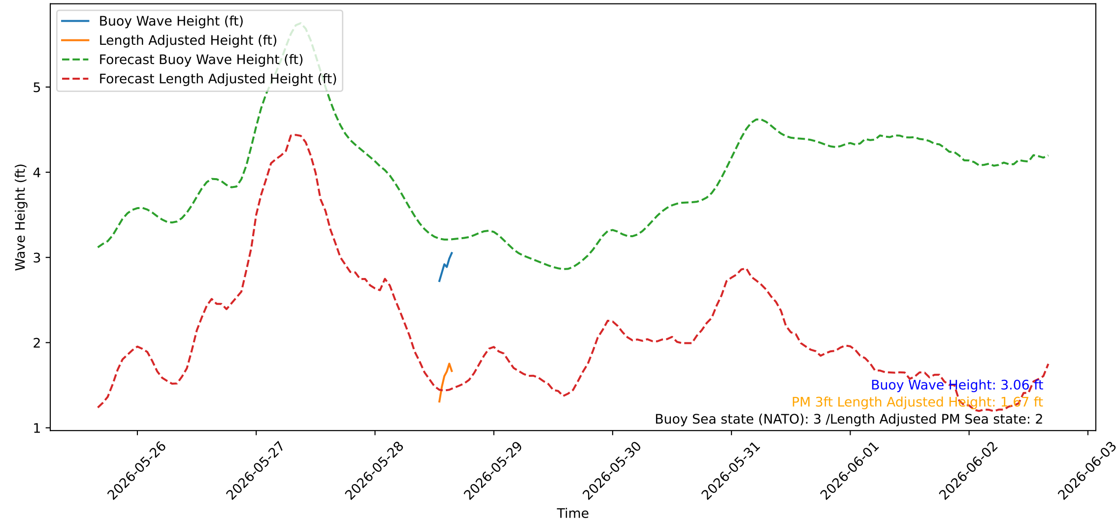
Wave Heights over Time for Oceanside Harbor at 2026-05-28 16:10:19
