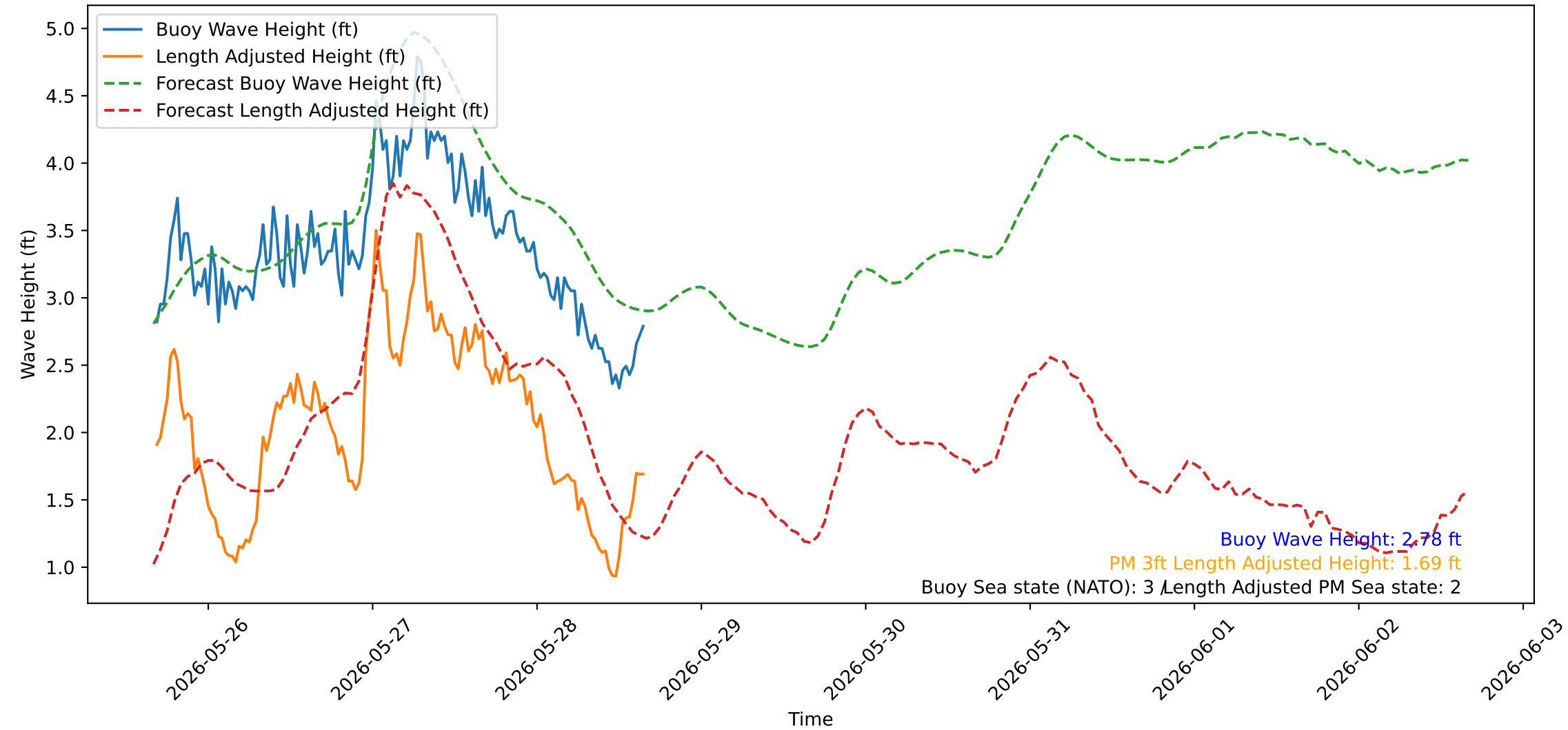
Wave Heights over Time for Red Beach at 2026-05-28 16:10:38
