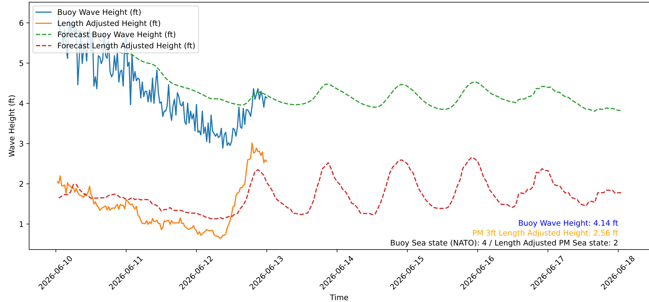
Wave Heights over Time for Green Beach at 2026-06-13 00:41:09
