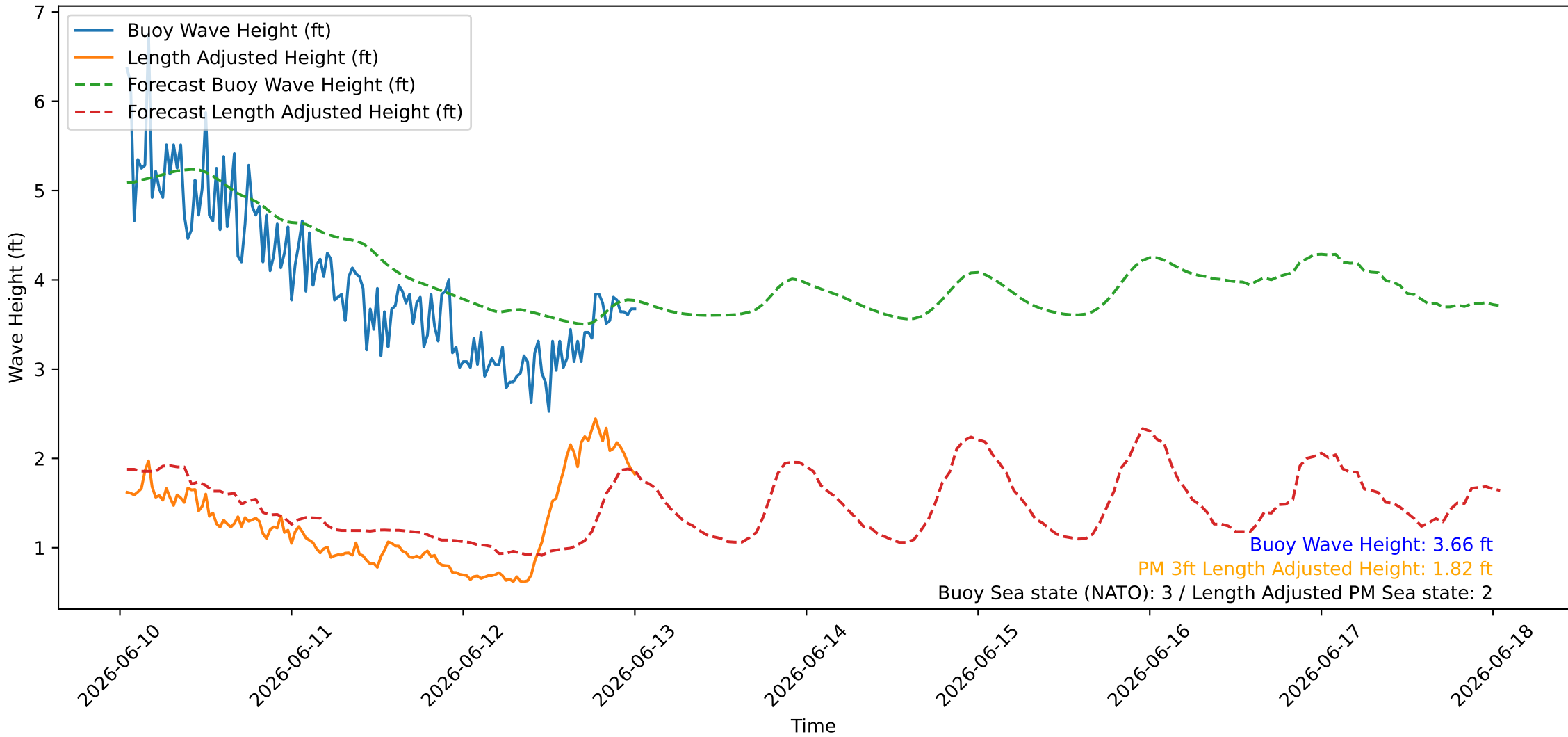
Wave Heights over Time for Red Beach at 2026-06-13 00:40:46
