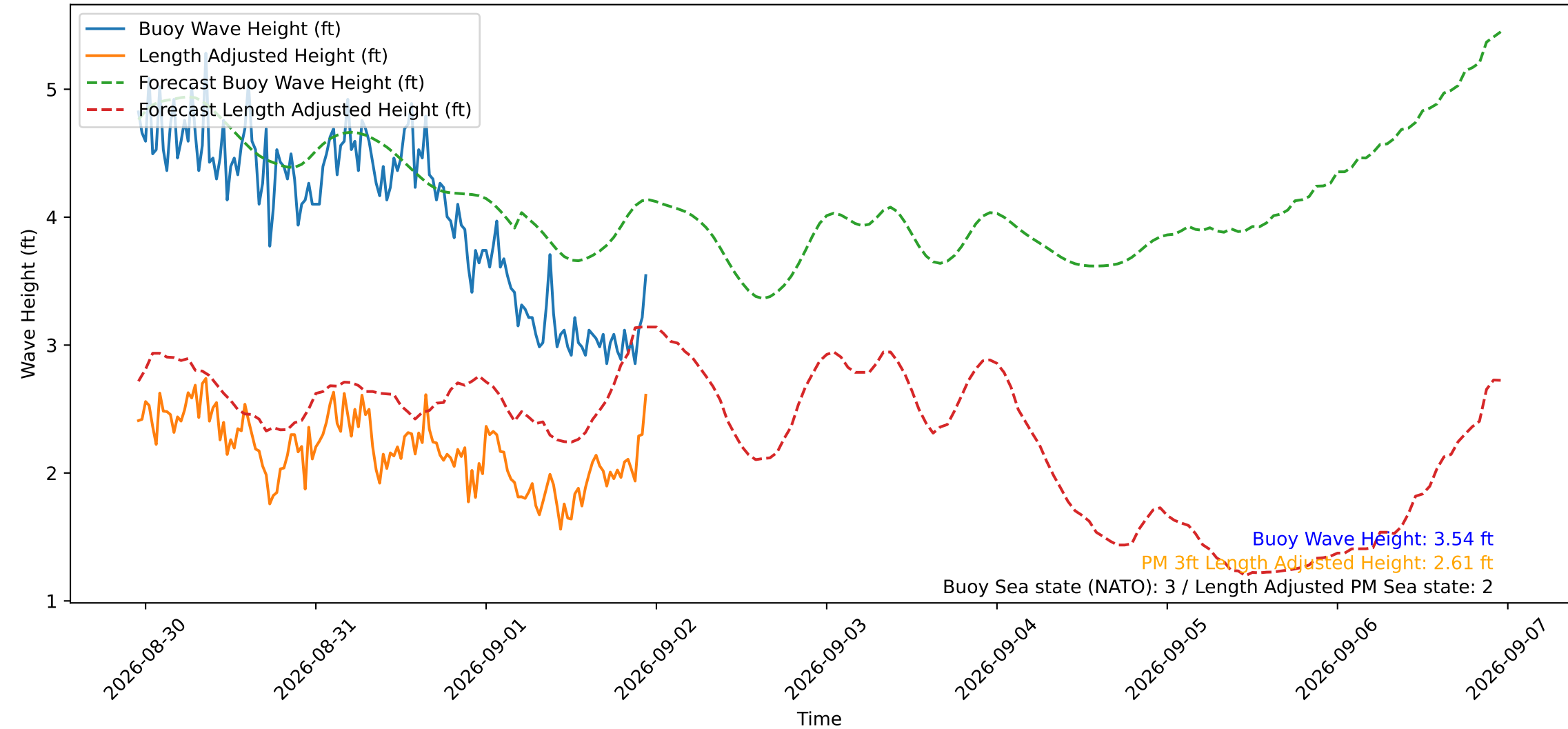
Wave Heights over Time for Oceanside Harbor at 2026-09-01 23:10:30
