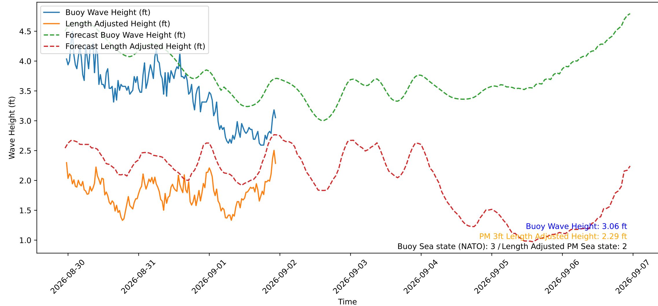
Wave Heights over Time for Red Beach at 2026-09-01 23:10:50
