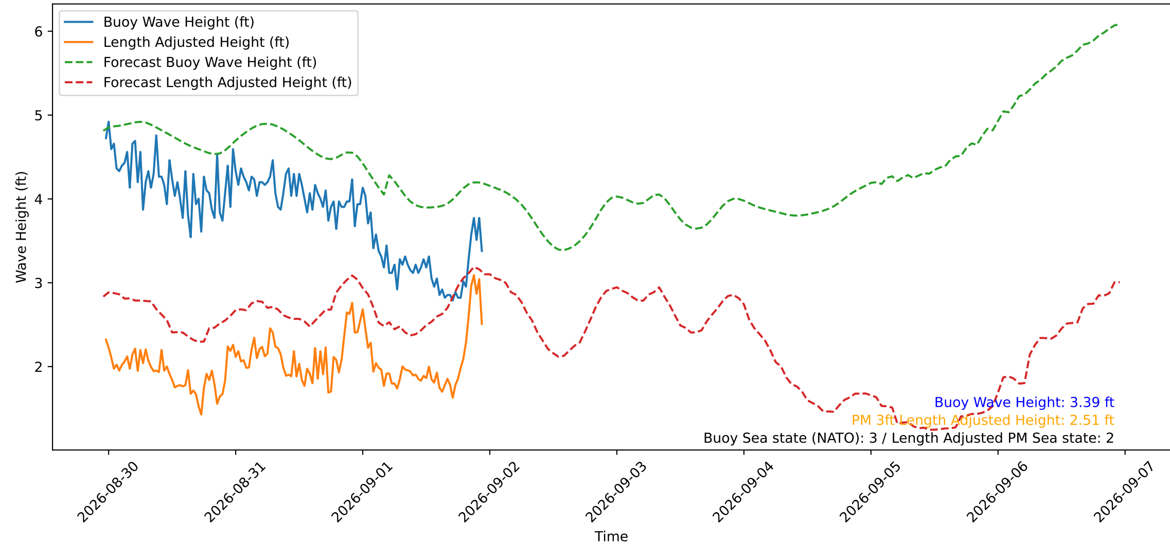
Wave Heights over Time for Green Beach at 2026-09-01 23:11:13
