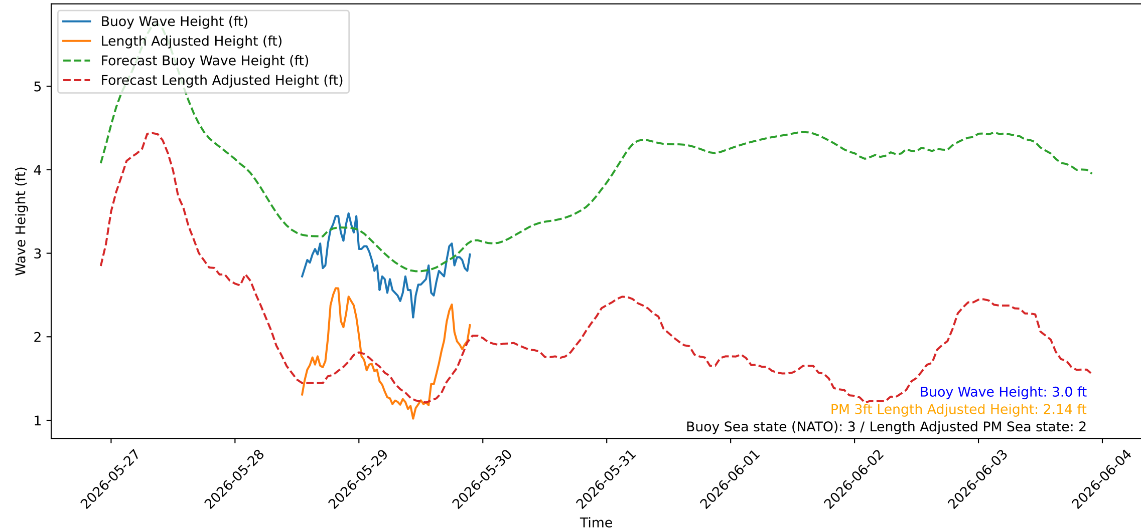
Wave Heights over Time for Oceanside Harbor at 2026-05-29 22:10:22
