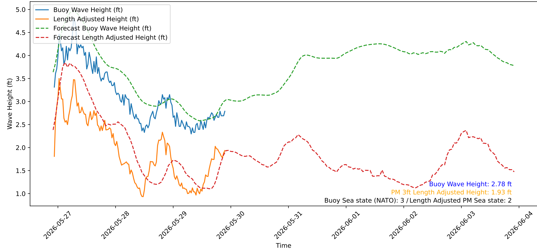
Wave Heights over Time for Red Beach at 2026-05-29 22:10:42
