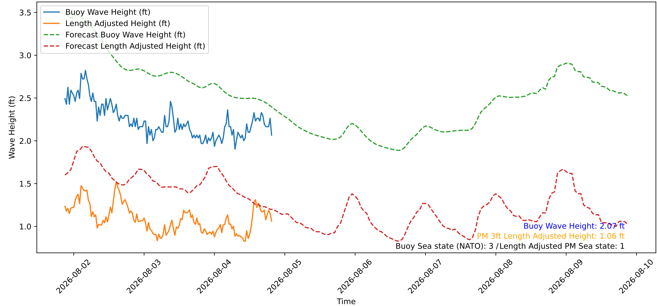
Wave Heights over Time for Red Beach at 2026-08-04 20:40:46
