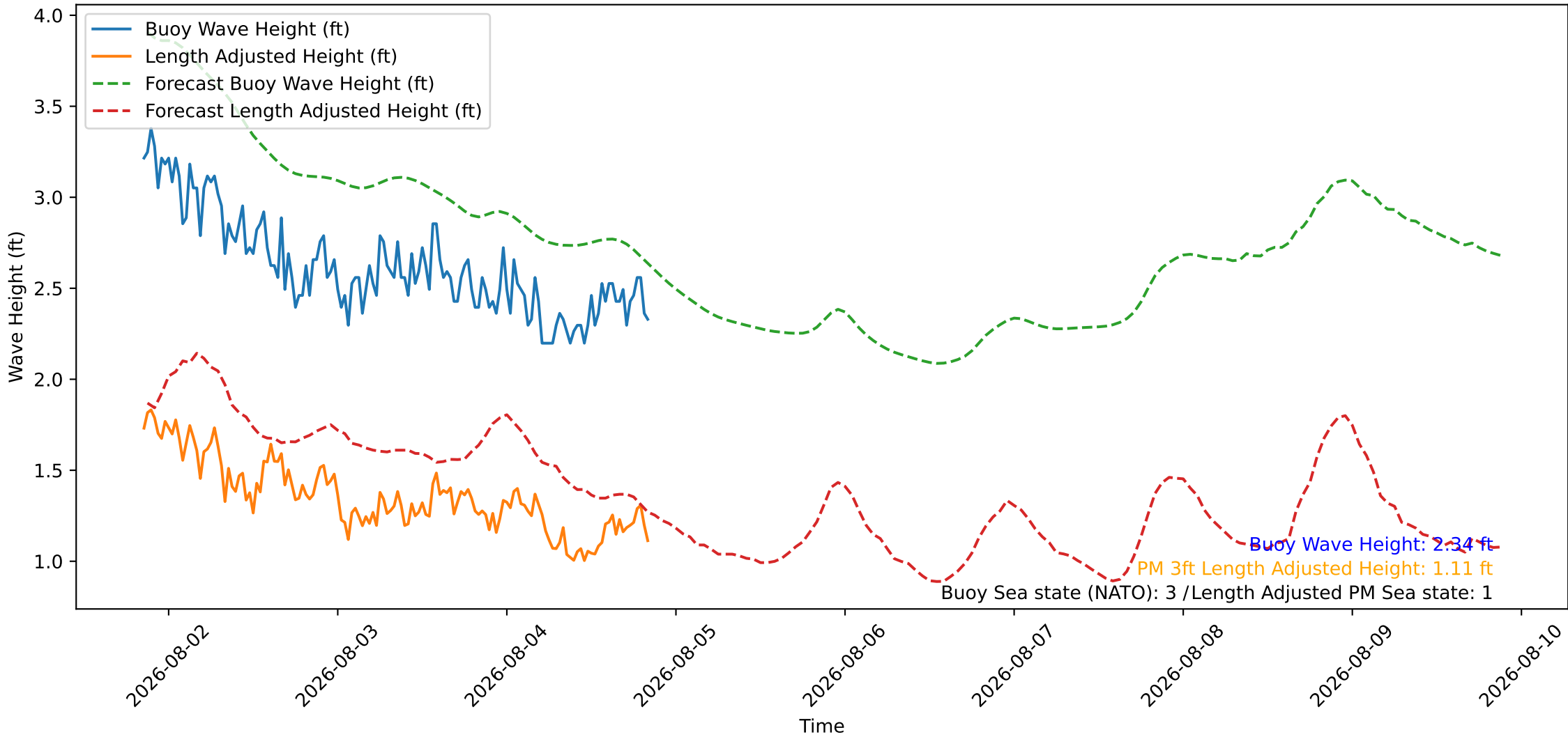
Wave Heights over Time for Oceanside Harbor at 2026-08-04 20:40:27
