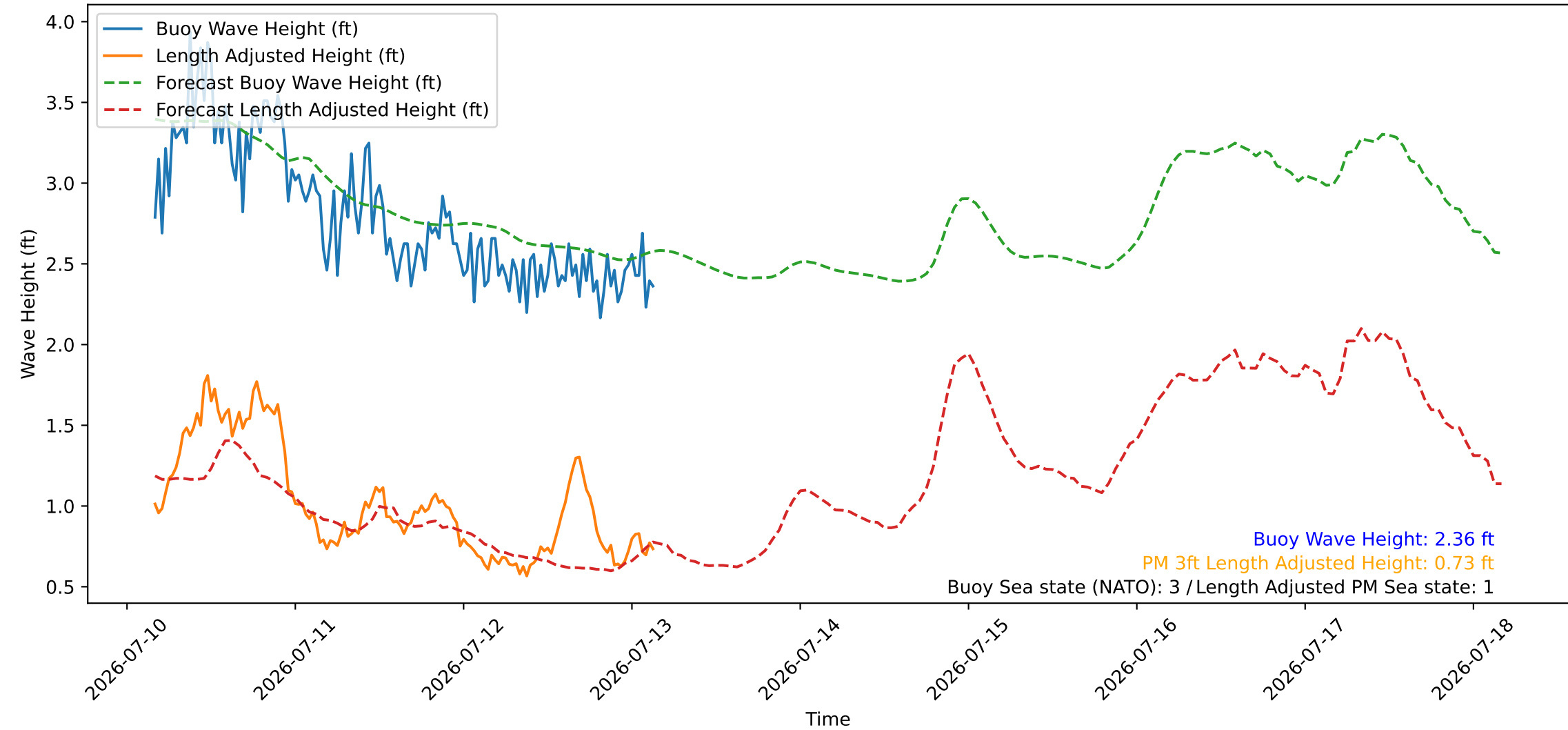
Wave Heights over Time for Red Beach at 2026-07-13 03:50:46
