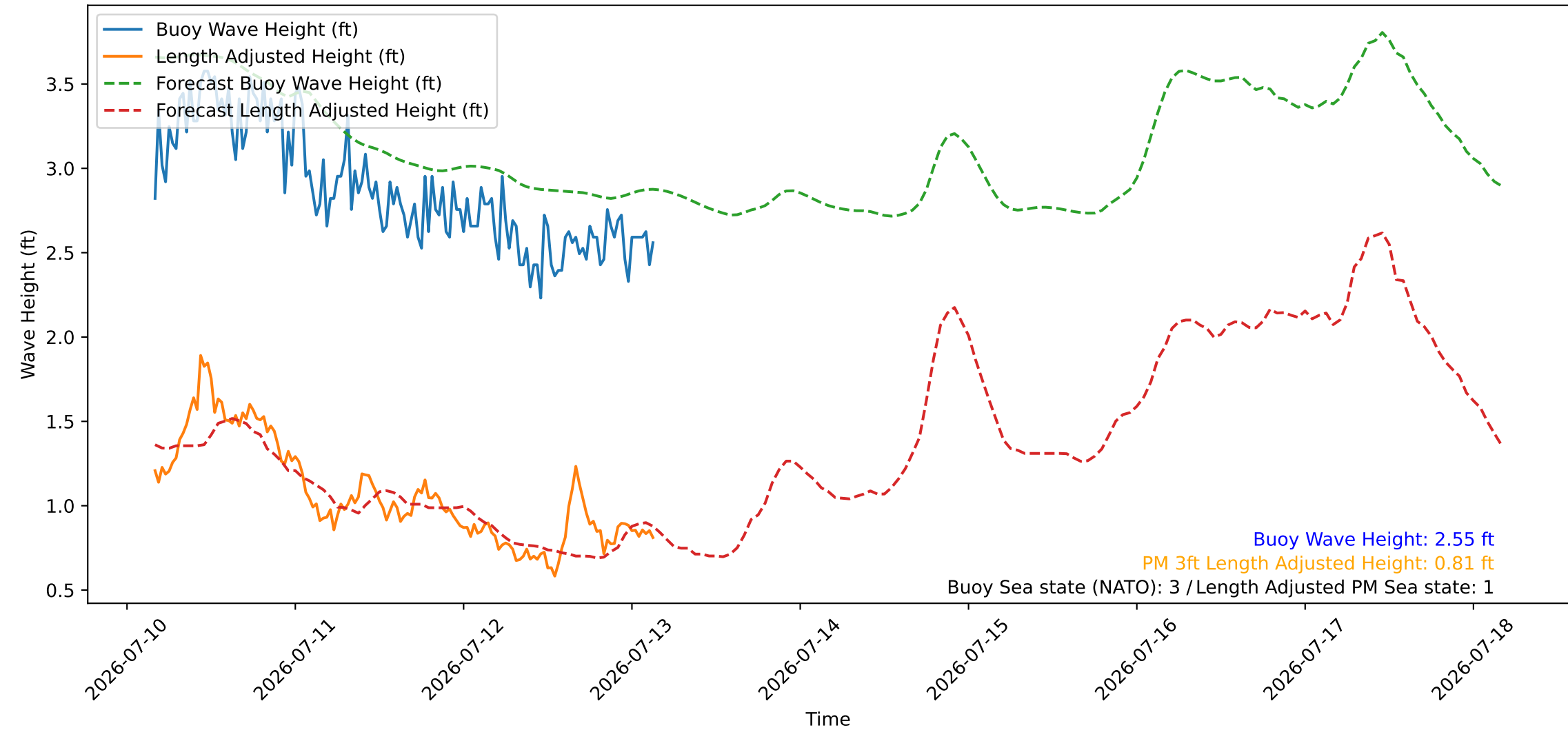
Wave Heights over Time for Green Beach at 2026-07-13 03:51:08
