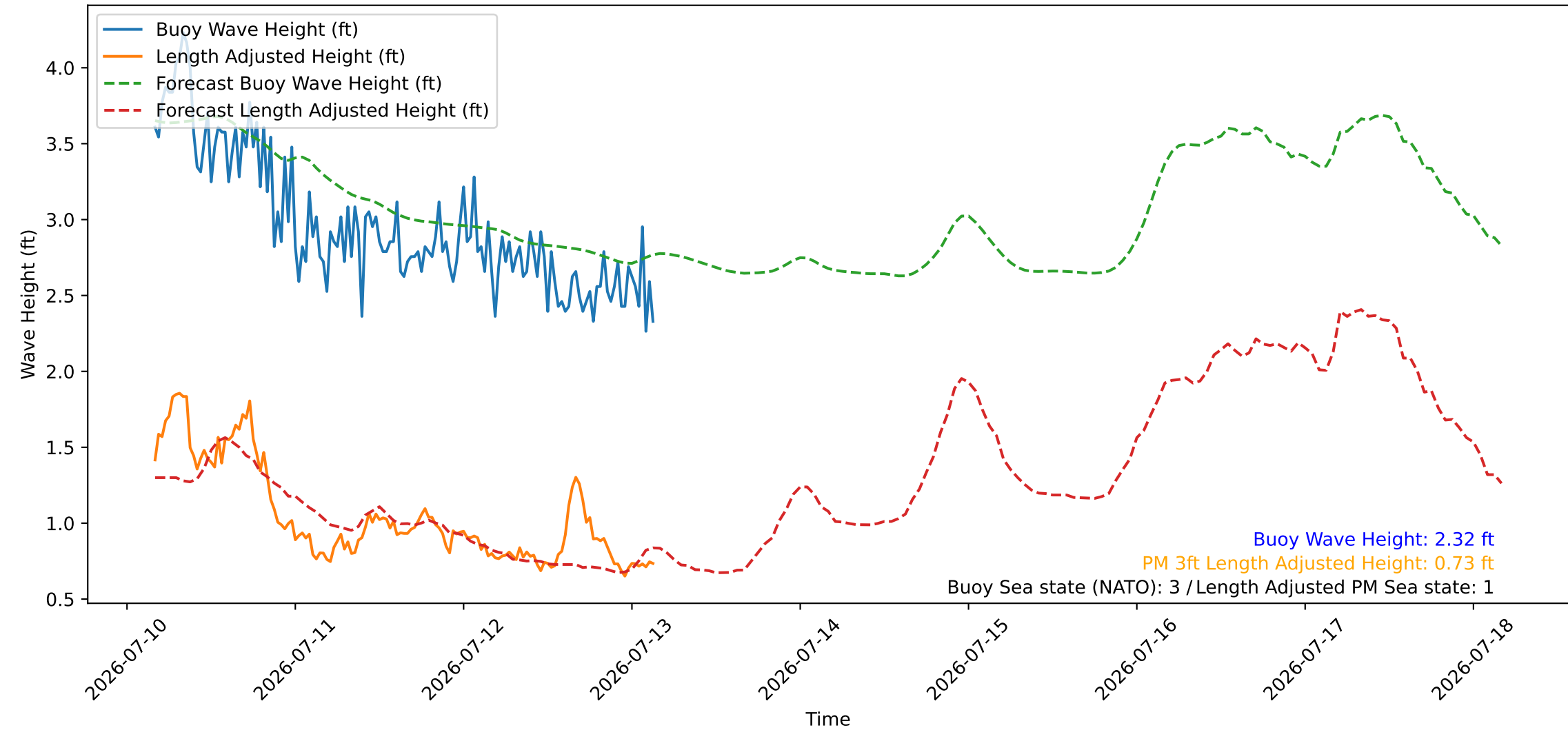
Wave Heights over Time for Oceanside Harbor at 2026-07-13 03:50:25
