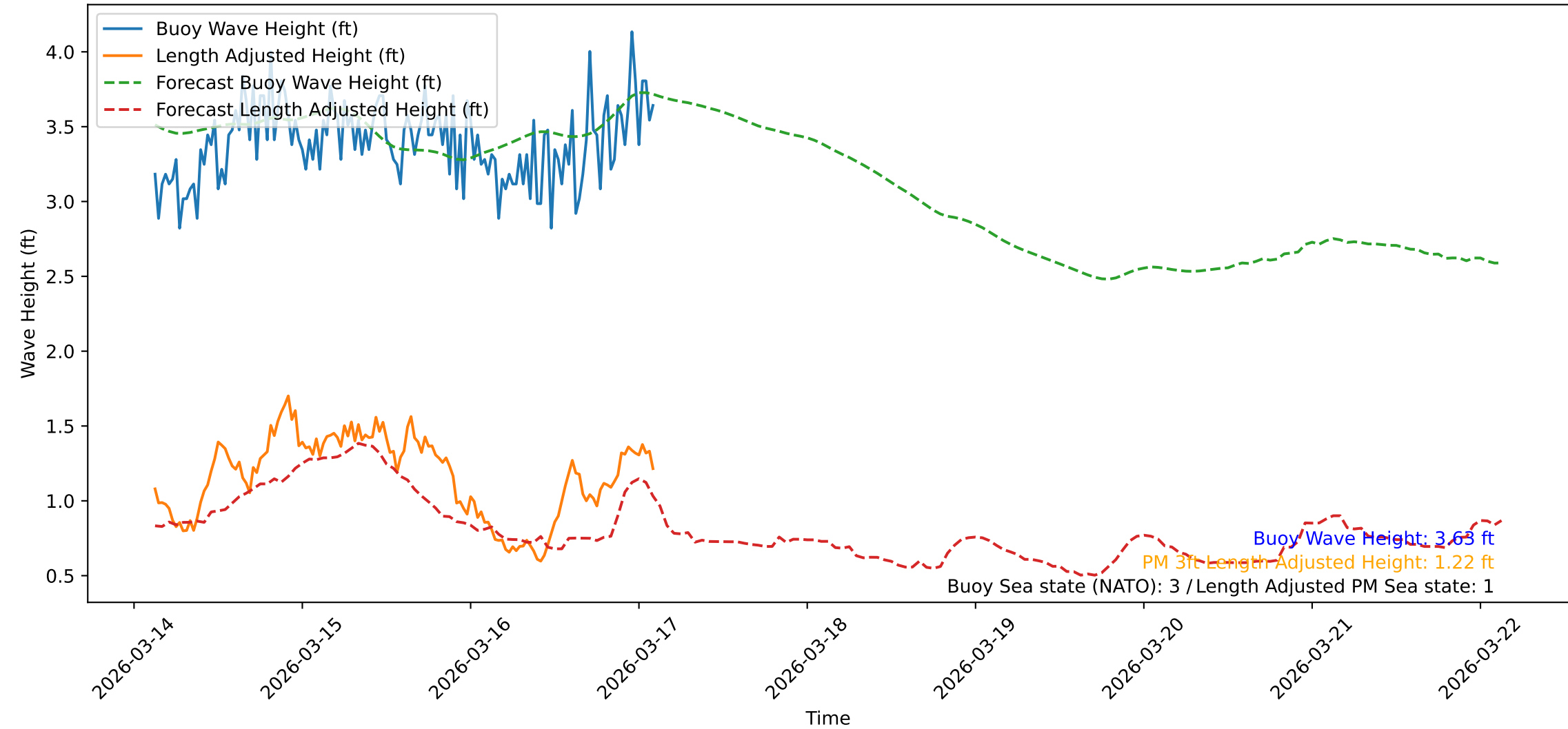
Wave Heights over Time for Green Beach at 2026-03-17 03:01:43
