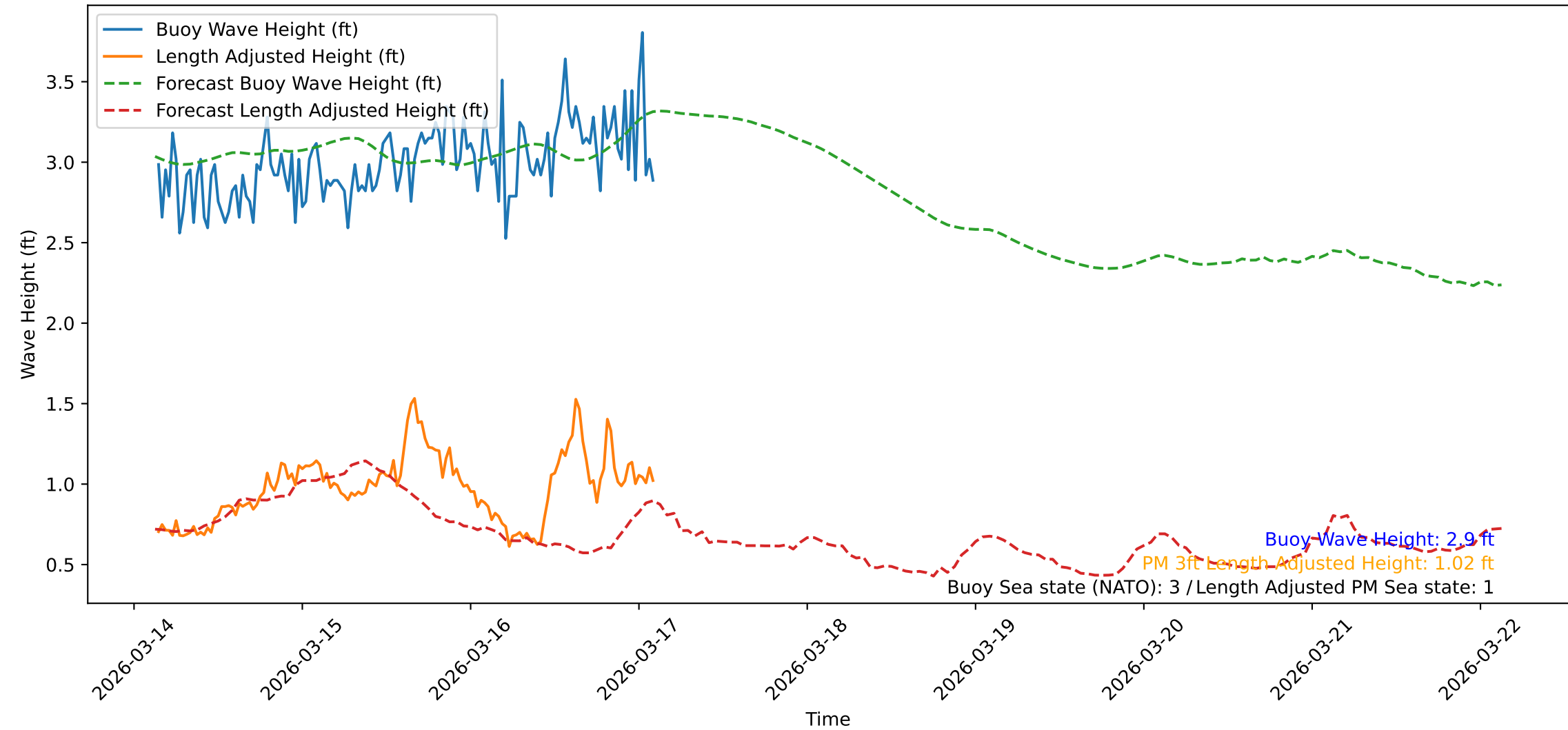
Wave Heights over Time for Red Beach at 2026-03-17 03:01:06
