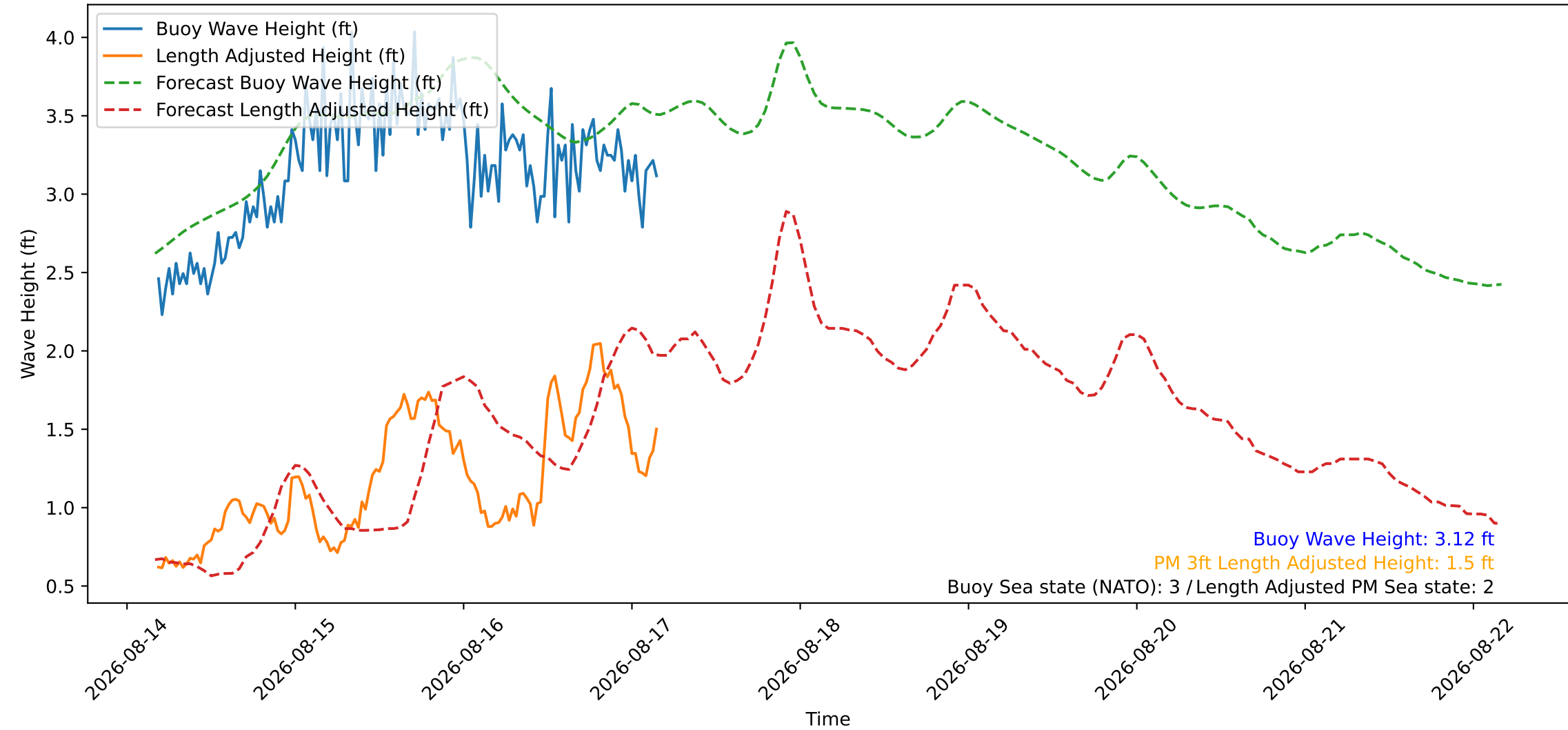
Wave Heights over Time for Red Beach at 2026-08-17 04:10:45
