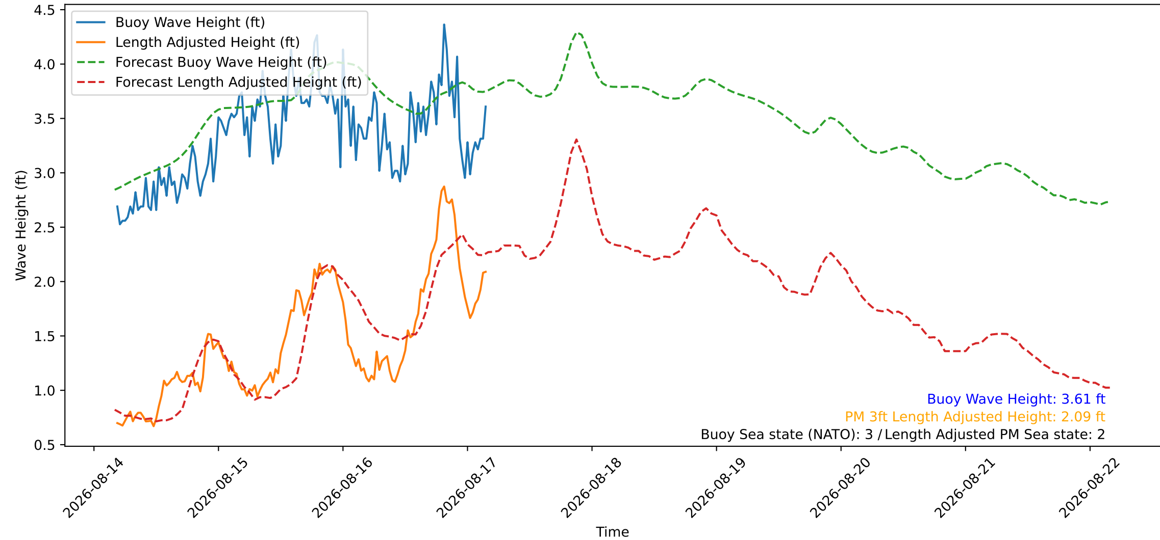
Wave Heights over Time for Green Beach at 2026-08-17 04:11:08
