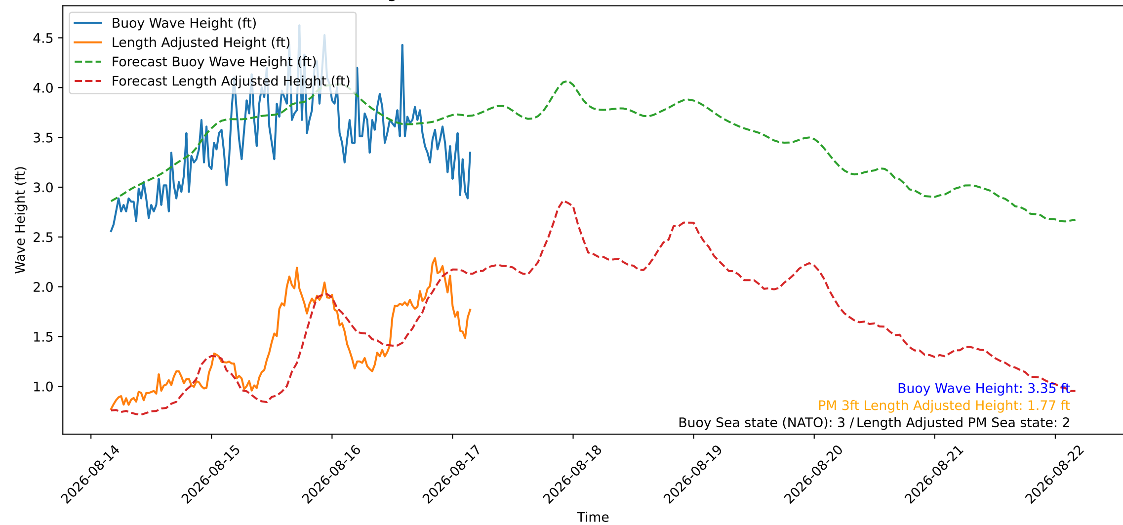
Wave Heights over Time for Oceanside Harbor at 2026-08-17 04:10:26
