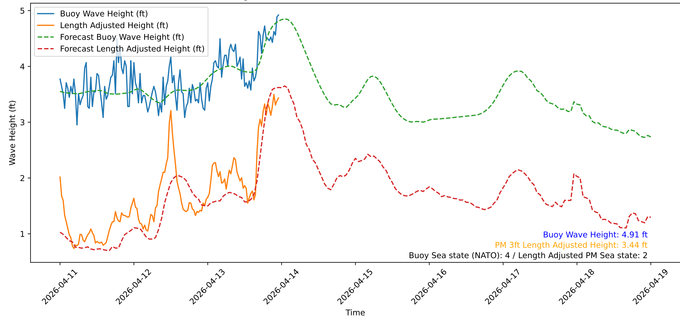
Wave Heights over Time for Green Beach at 2026-04-13 23:51:13
