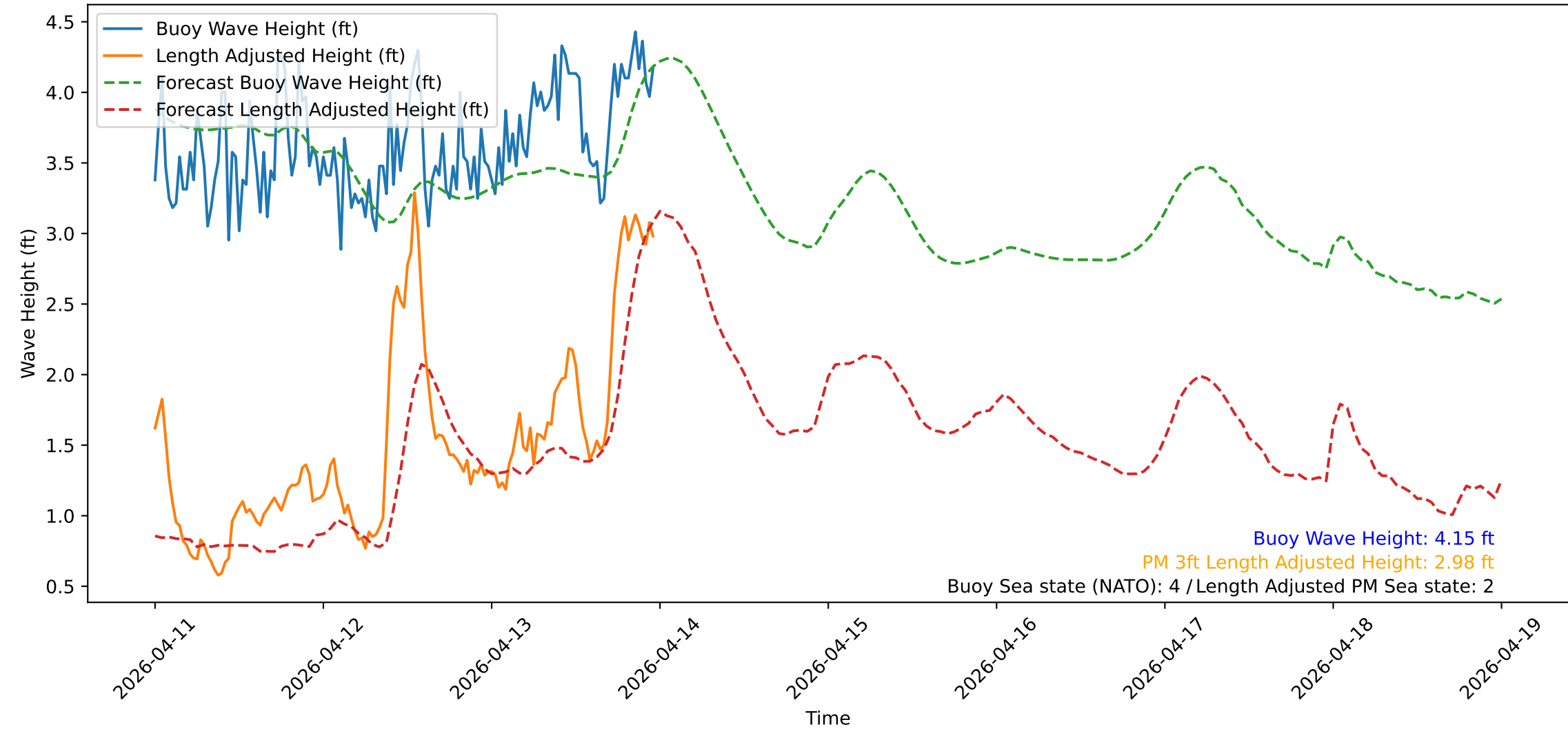
Wave Heights over Time for Red Beach at 2026-04-13 23:50:51
