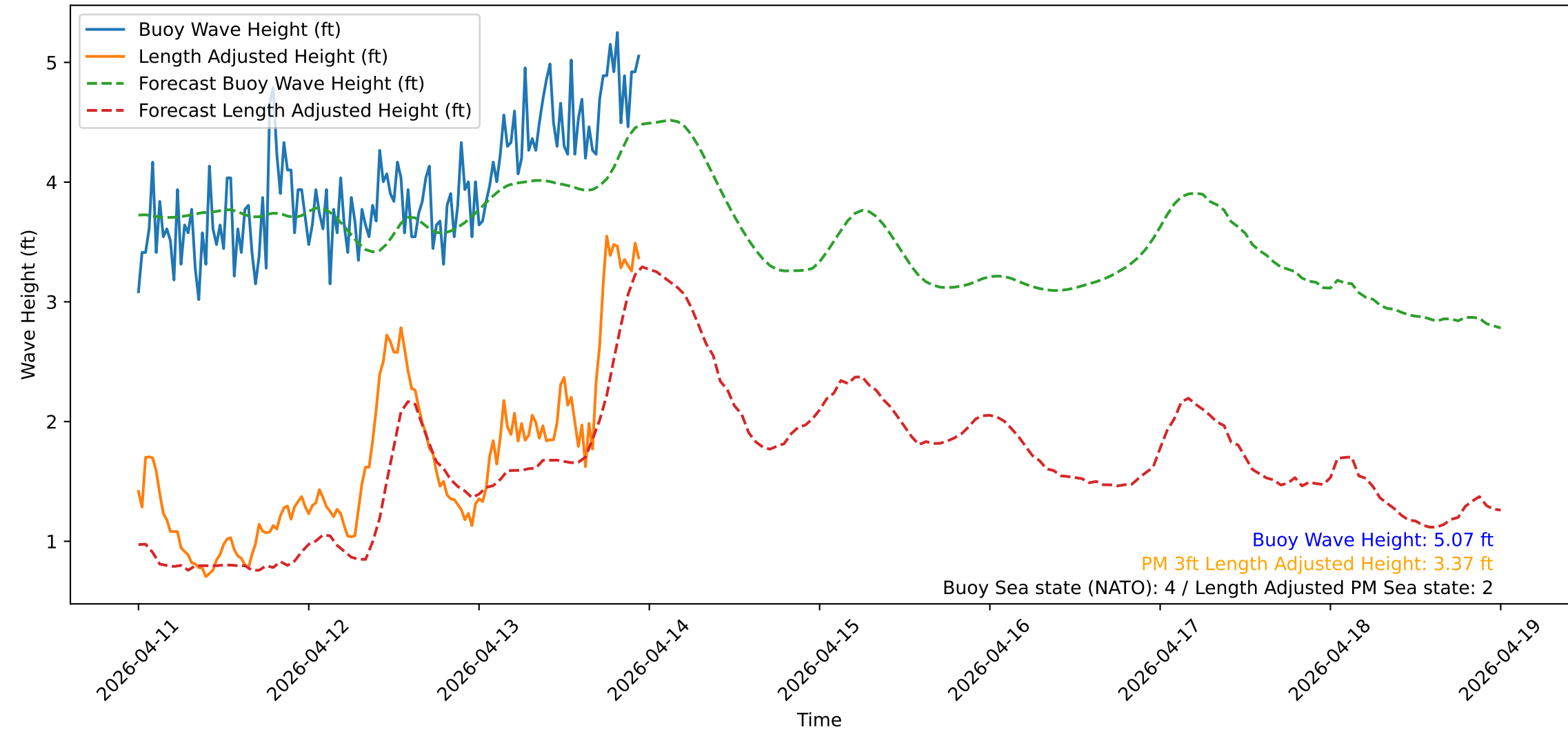
Wave Heights over Time for Oceanside Harbor at 2026-04-13 23:50:31
