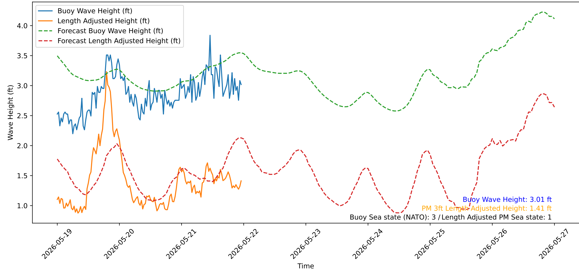
Wave Heights over Time for Oceanside Harbor at 2026-05-21 23:50:30
