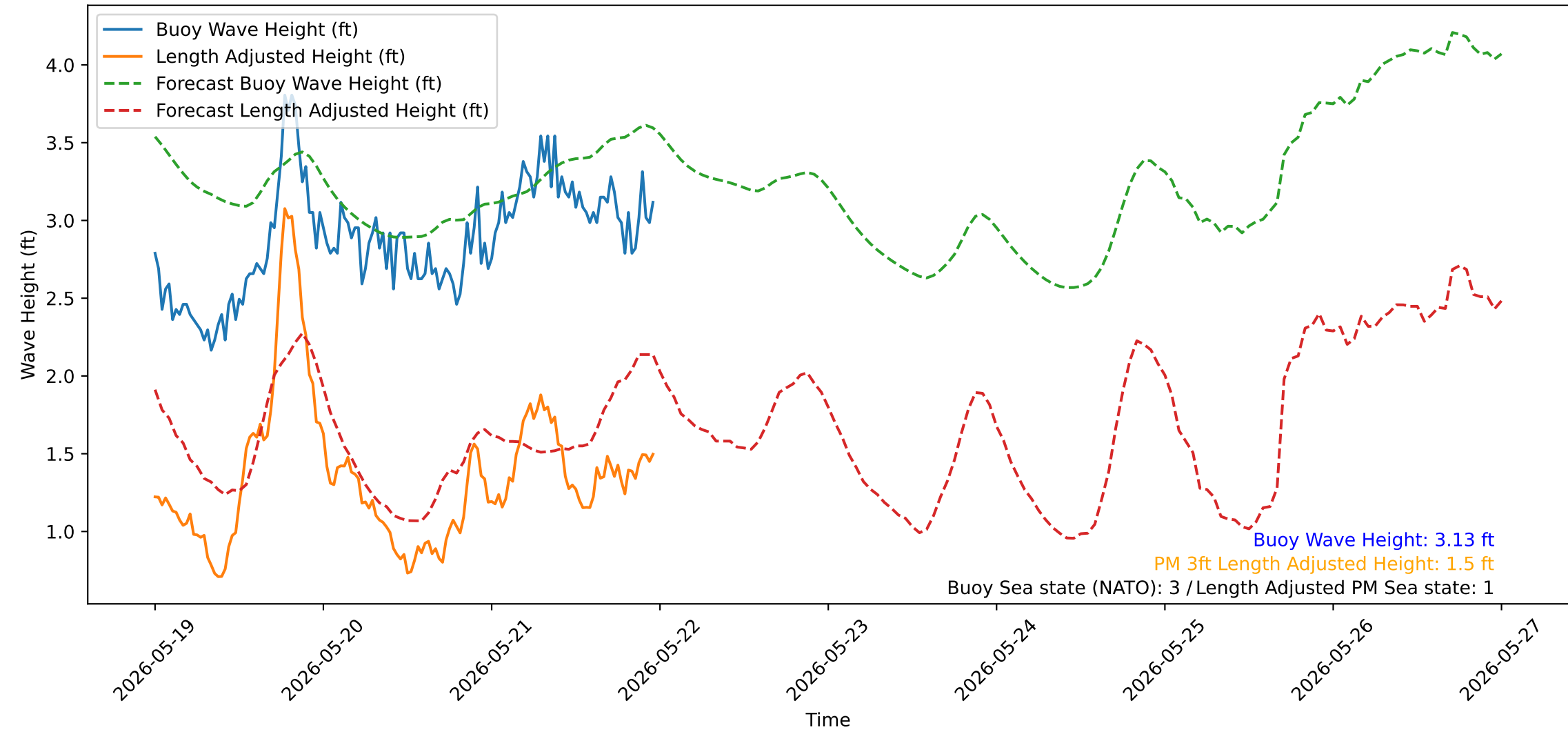
Wave Heights over Time for Green Beach at 2026-05-21 23:51:13
