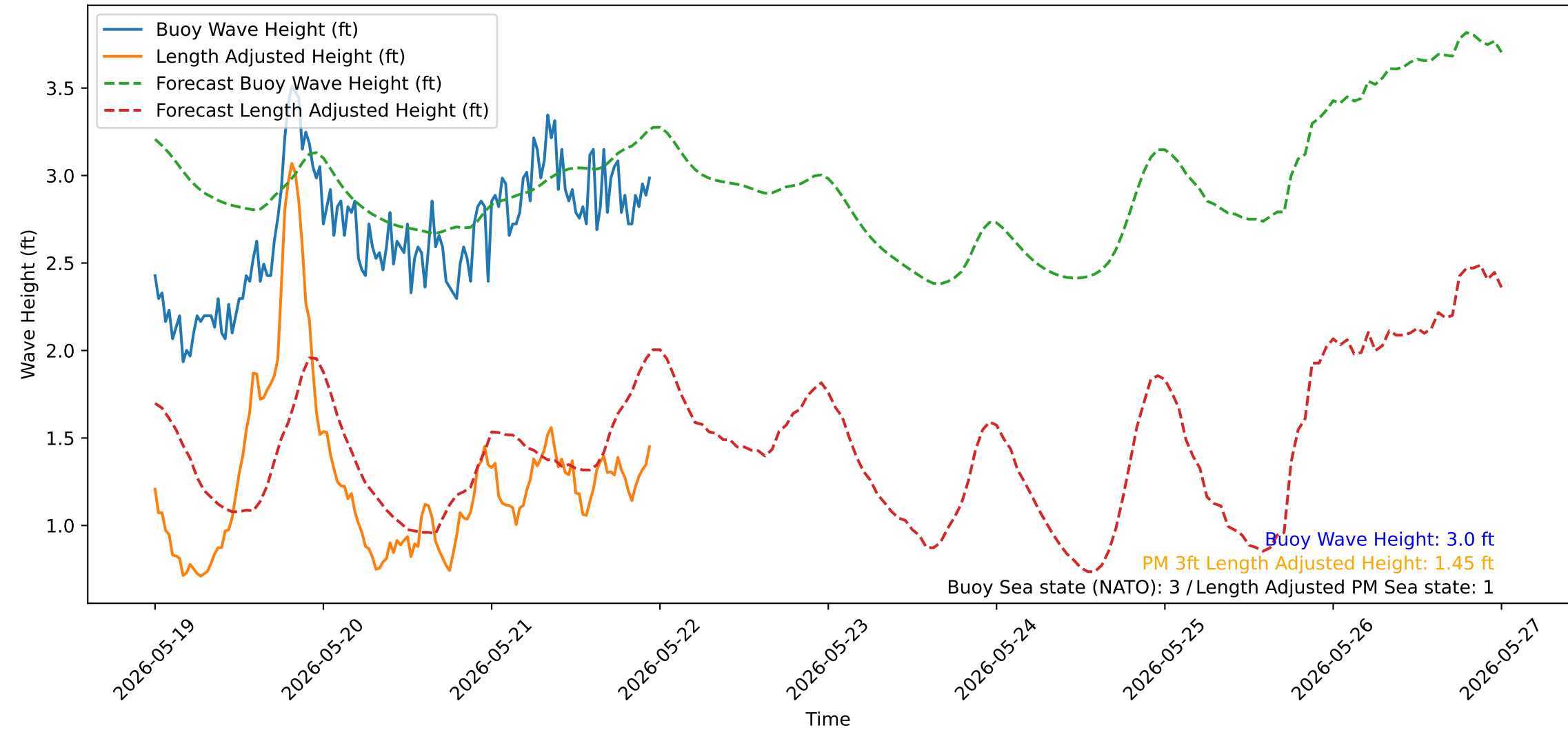
Wave Heights over Time for Red Beach at 2026-05-21 23:50:51
