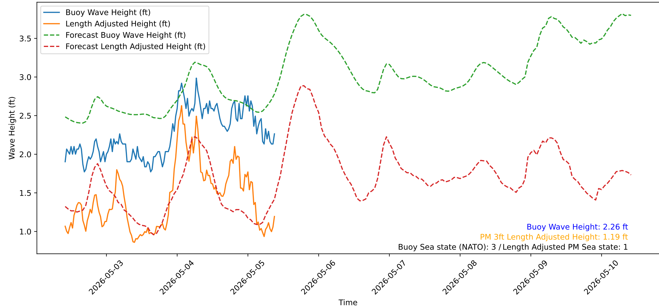
Wave Heights over Time for Green Beach at 2026-05-05 10:01:13
