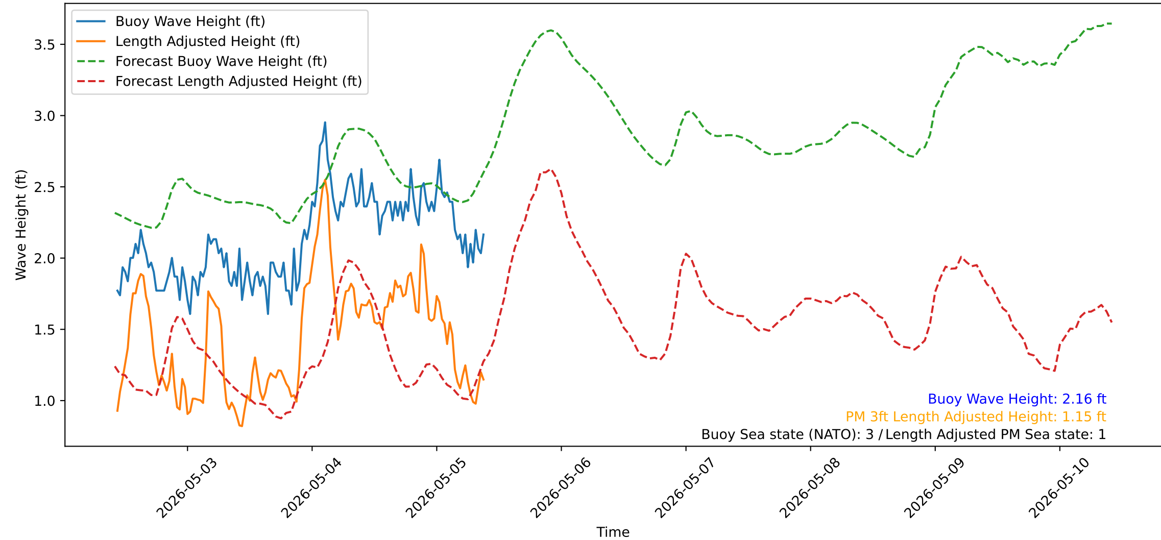
Wave Heights over Time for Red Beach at 2026-05-05 10:00:51
