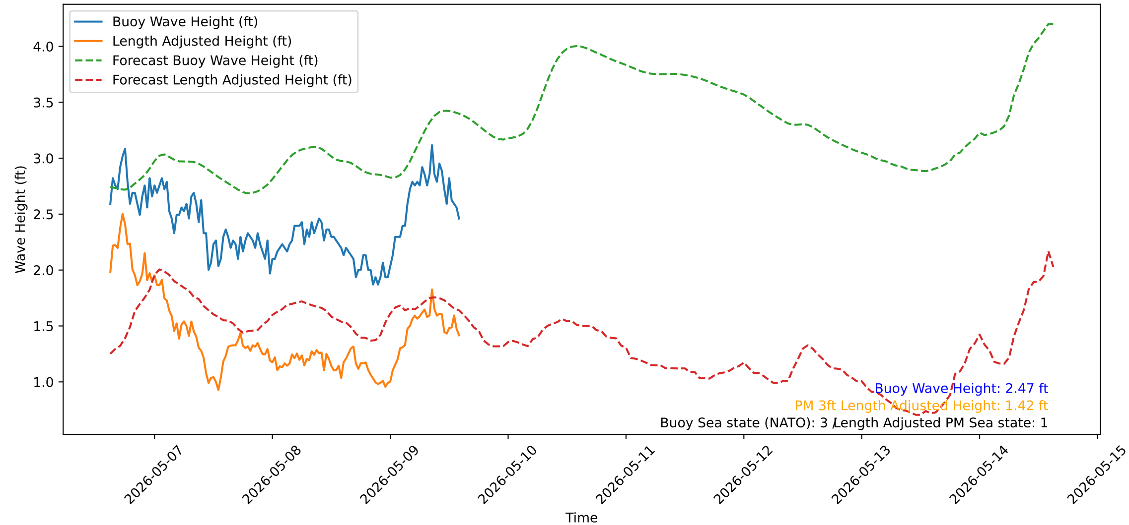
Wave Heights over Time for Oceanside Harbor at 2026-05-09 14:50:31
