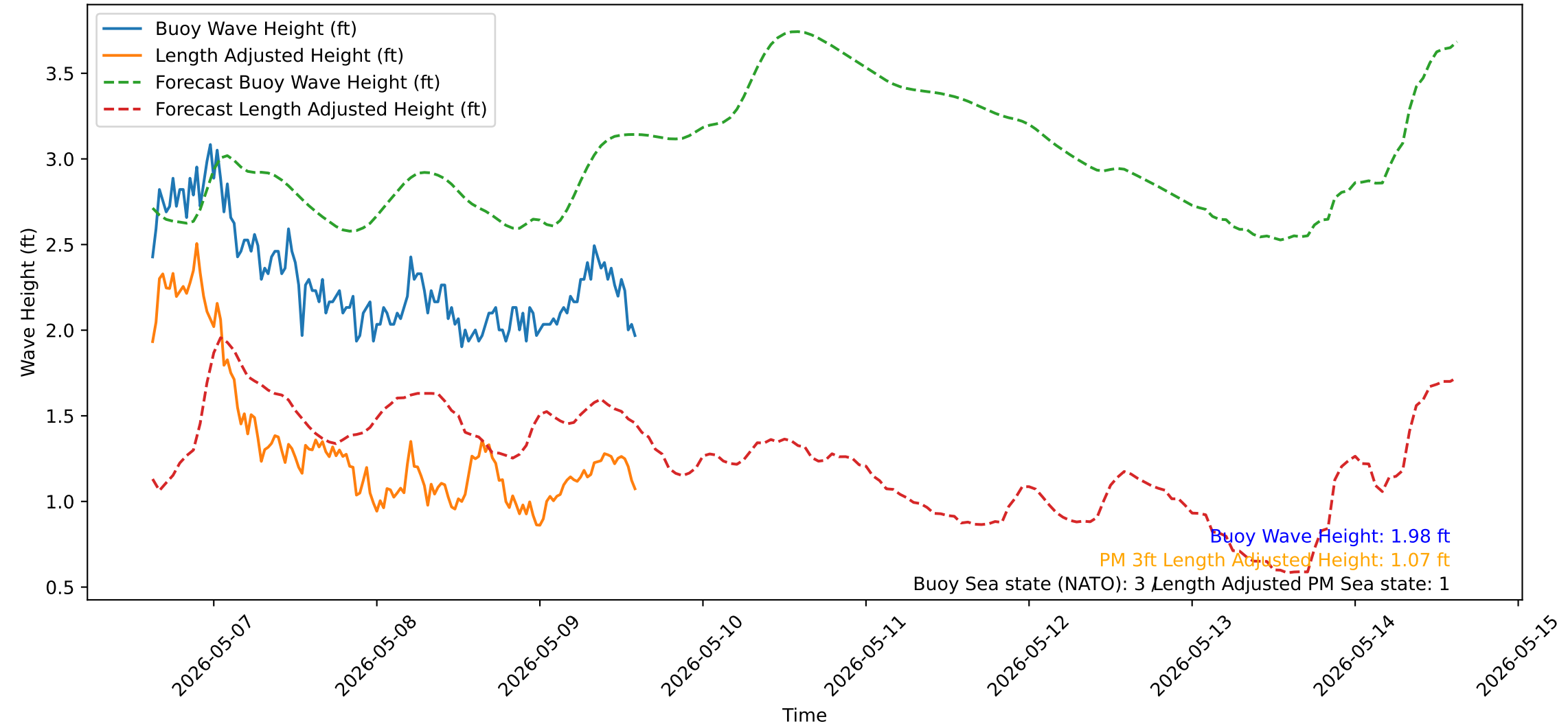
Wave Heights over Time for Red Beach at 2026-05-09 14:50:51
