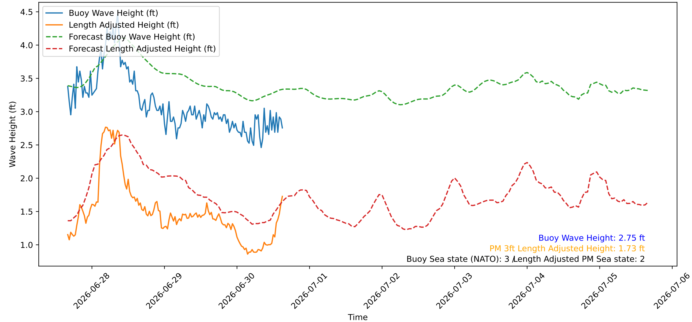
Wave Heights over Time for Red Beach at 2026-06-30 15:50:46
