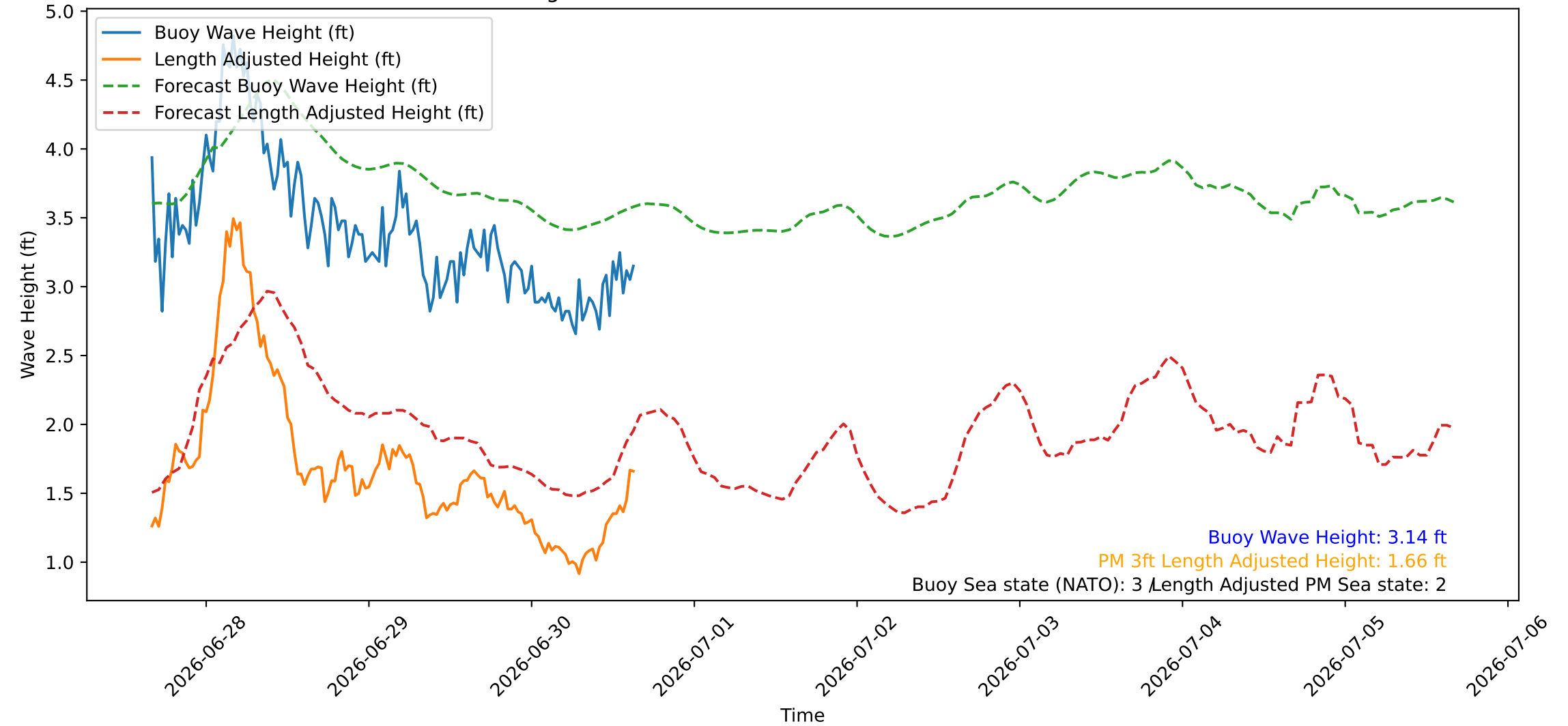
Wave Heights over Time for Green Beach at 2026-06-30 15:51:08
