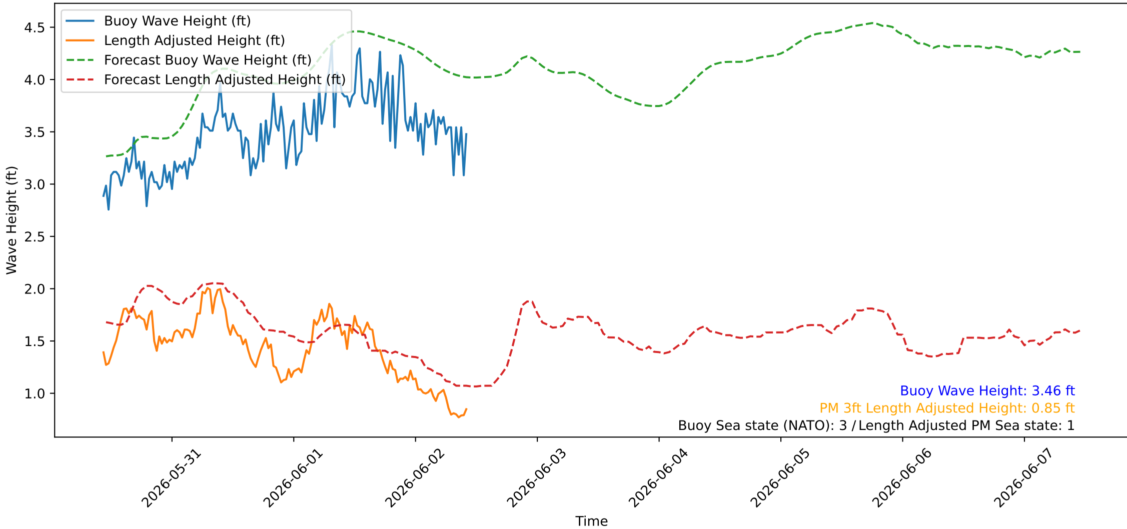
Wave Heights over Time for Green Beach at 2026-06-02 10:41:07
